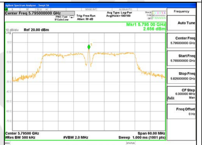
Test Mode: 802.11AC(40)---5795
