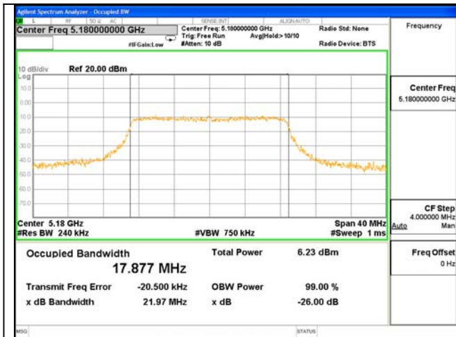
26dB & 99% Bandwidth Test Mode: 802.11n(HT20)--5180
