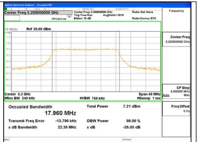
26dB & 99% Bandwidth Test Mode: 802.11n(HT20)---5200
