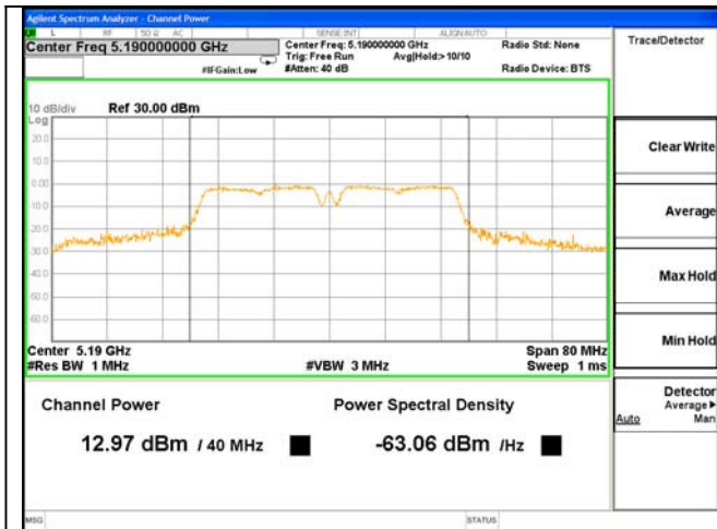
Test Mode: 802.11AC(40)---5190
