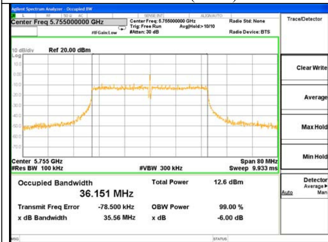
6dB Bandwidth Test Mode: 802.11n(HT40)--5755
