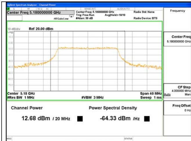
Test Mode: 802.11AC(20)---5180
