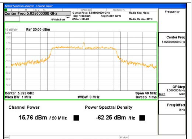
Test Mode: 802.11n(HT20)---5825
