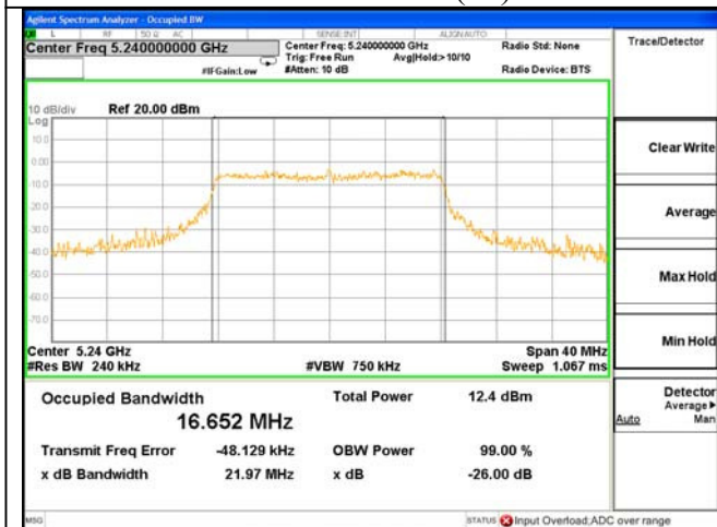
26dB & 99% Bandwidth Test Mode: 802.11AC(20)--5240
