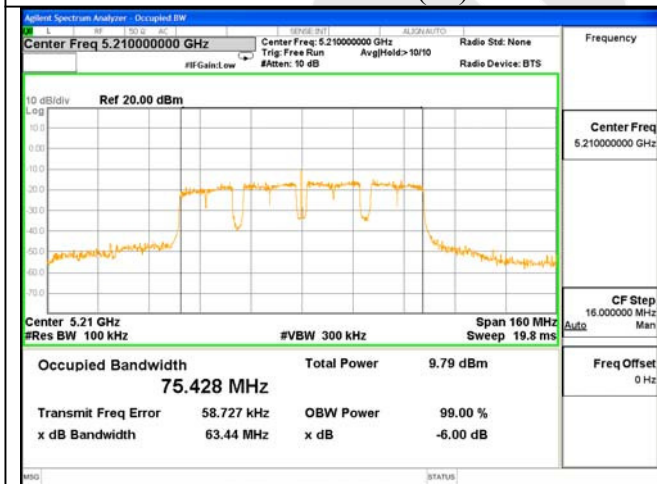
6dB Bandwidth Test Mode: 802.11AC(80)--5210
