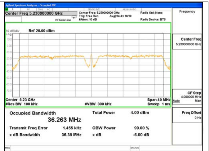
6dB Bandwidth Test Mode: 802.11AC(40)---5230
