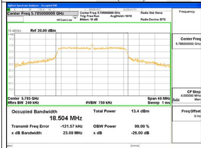
26dB & 99% Bandwidth Test Mode: 802.11n(HT20)--5785
