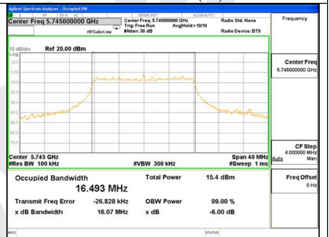
6dB Bandwidth Test Mode: 802.11AC(20)---5745
