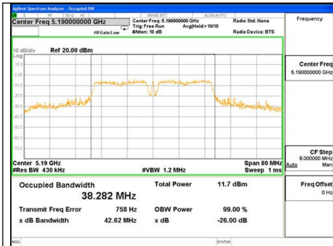
26dB & 99% Bandwidth Test Mode: 802.11AC(40)--5190
