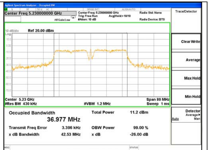
26dB & 99% Bandwidth Test Mode: 802.11AC(40)---5230
