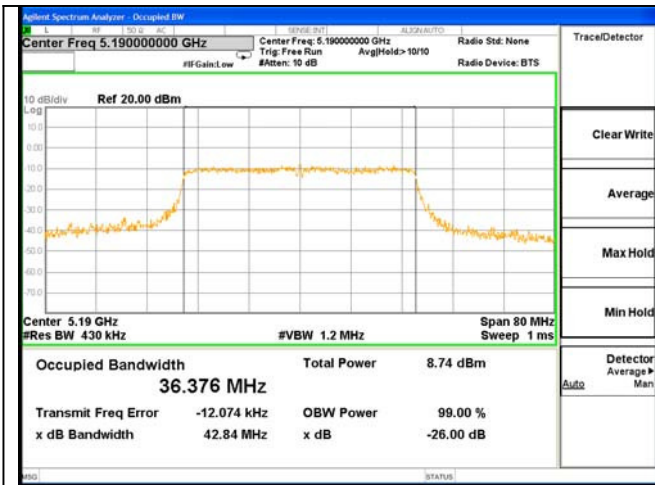
26dB & 99% Bandwidth Test Mode: 802.11n(HT40)--5190
