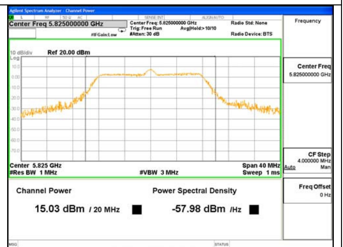
Test Mode: 802.11AC(20)---5825
