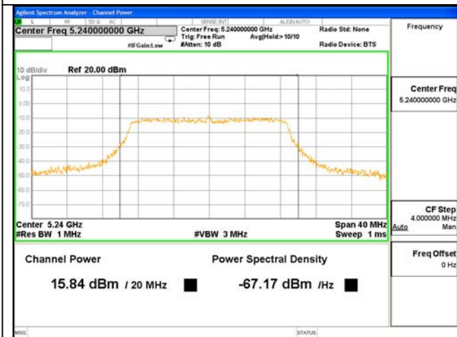
Test Mode: 802.11n(HT20)---5240
