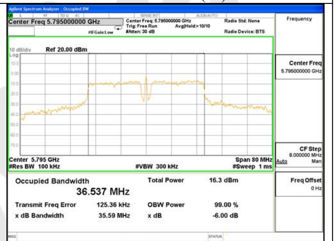
6dB Bandwidth Test Mode: 802.11AC(40)---5795
