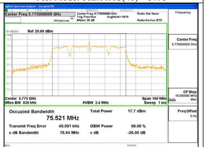
26dB & 99% Bandwidth Test Mode: 802.11AC(80)---5775
