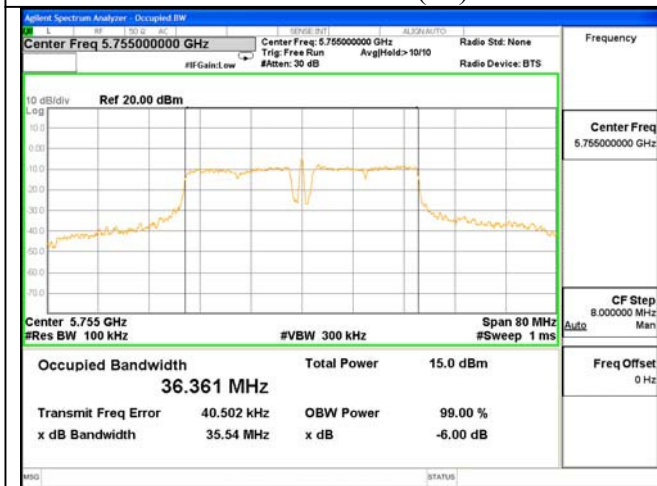
6dB Bandwidth Test Mode: 802.11AC(40)--5755
