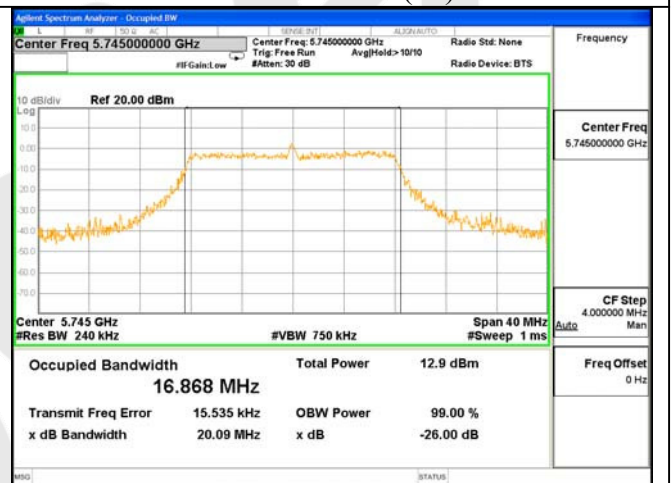
26dB & 99% Bandwidth Test Mode: 802.11AC(20)---5745
