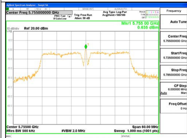
Test Mode: 802.11AC(40)---5755
