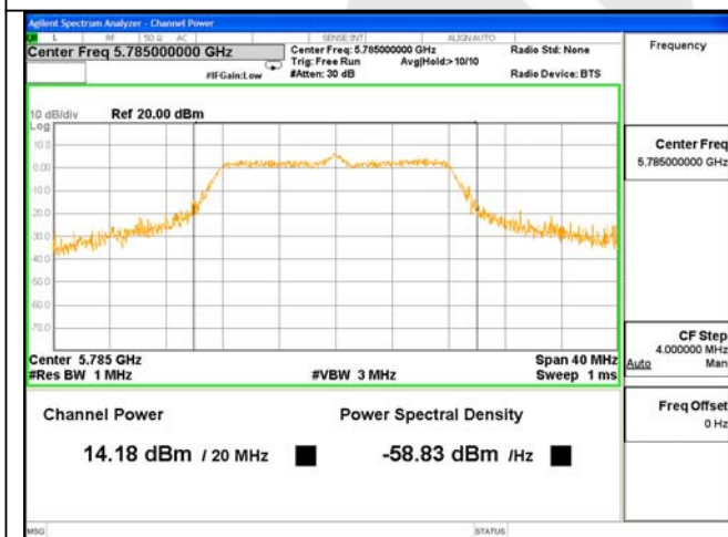
Test Mode: 802.11AC(20)---5785
