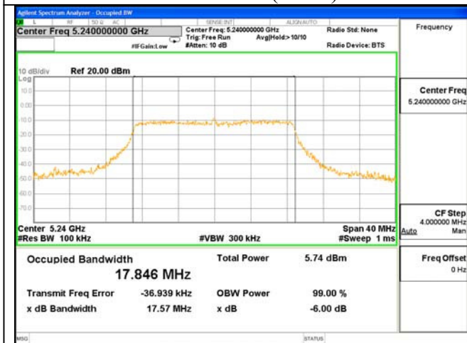
6dB Bandwidth Test Mode: 802.11n(HT20)--5240
