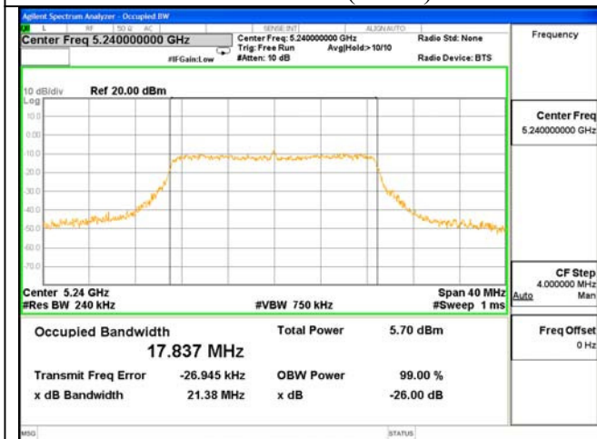
26dB & 99% Bandwidth Test Mode: 802.11n(HT20)--5240
