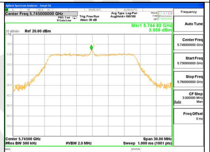
Test Mode: 802.11AC(20)---5745
