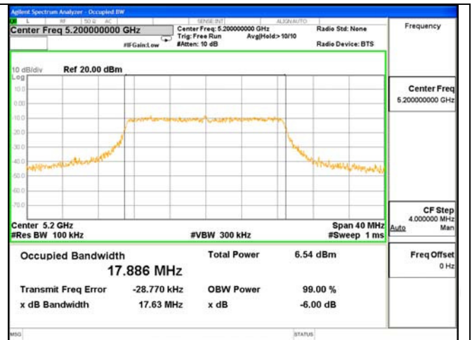
6dB Bandwidth Test Mode: 802.11n(HT20)---5200
