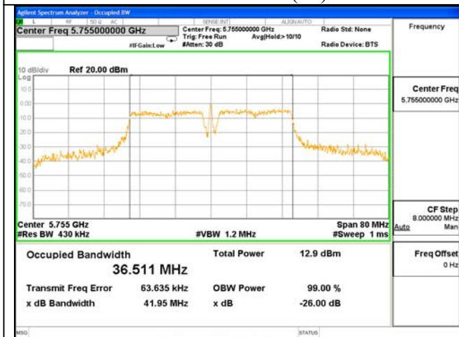
26dB & 99% Bandwidth Test Mode: 802.11AC(40)--5755
