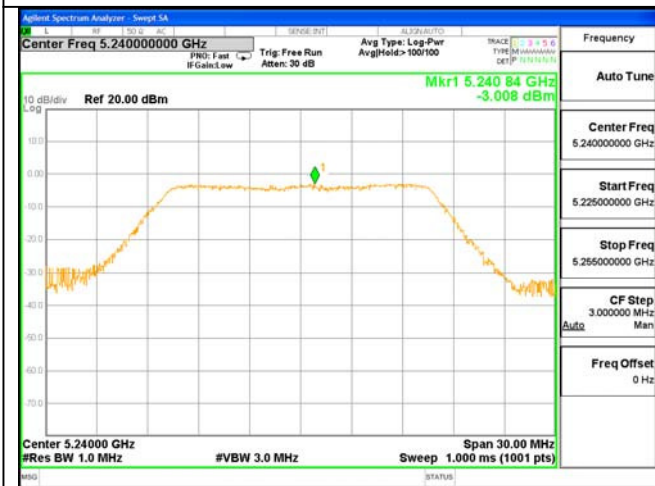
Test Mode: 802.11AC(20)---5240
