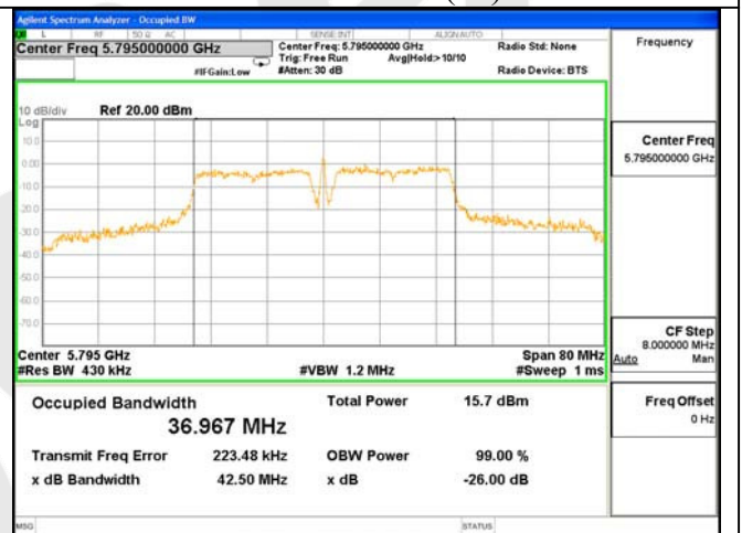
26dB & 99% Bandwidth Test Mode: 802.11AC(40)---5795
