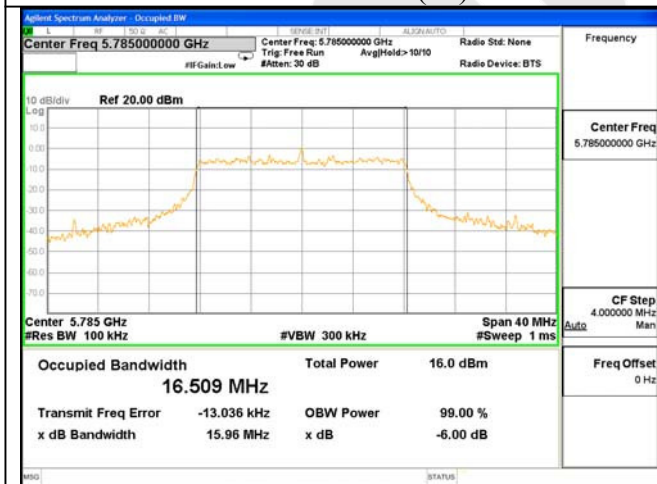
6dB Bandwidth Test Mode: 802.11AC(20)--5785
