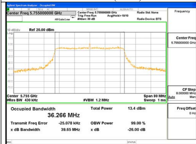
26dB & 99% Bandwidth Test Mode: 802.11n(HT40)--5755
