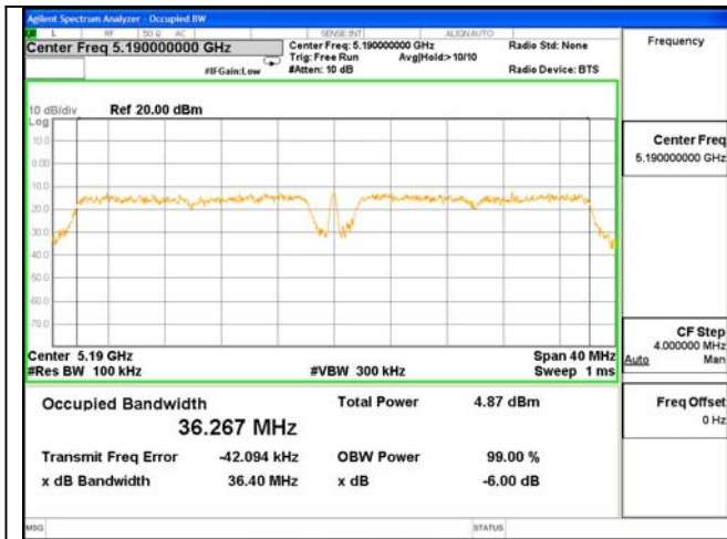
6dB Bandwidth Test Mode: 802.11AC(40)--5190
