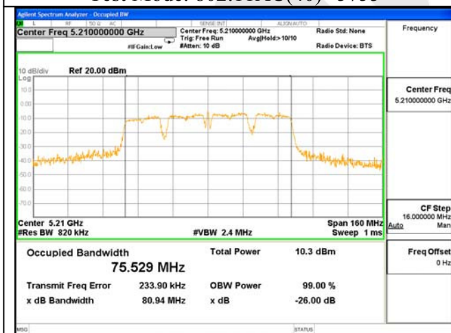
26dB & 99% Bandwidth Test Mode: 802.11AC(80)--5210
