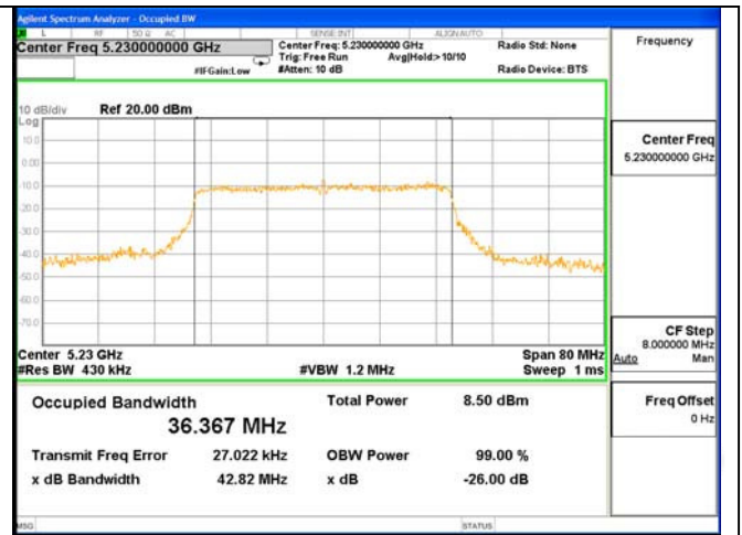
26dB & 99% Bandwidth Test Mode: 802.11n(HT40)---5230
