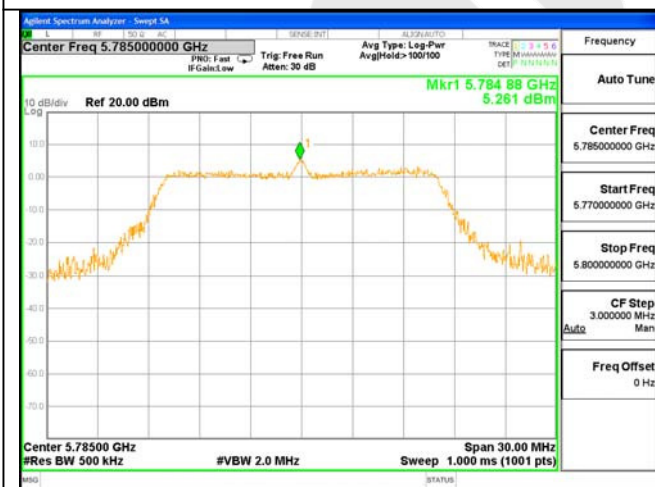
Test Mode: 802.11AC(20)---5785
