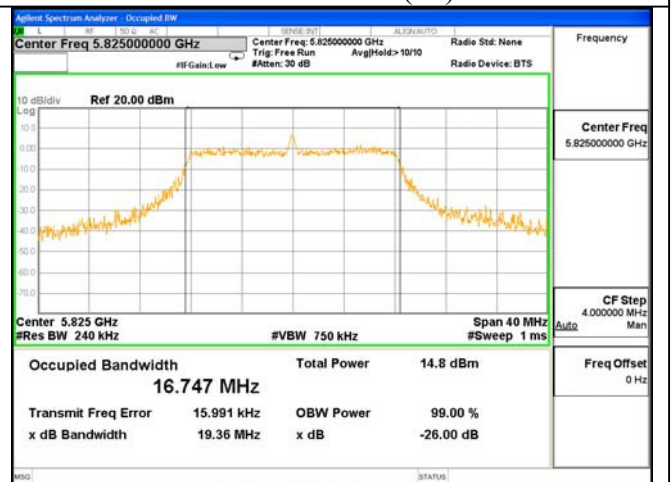
26dB & 99% Bandwidth Test Mode: 802.11AC(20)---5825
