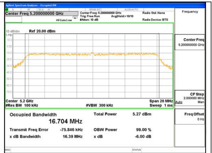
6dB Bandwidth Test Mode: 802.11AC(20)---5200
