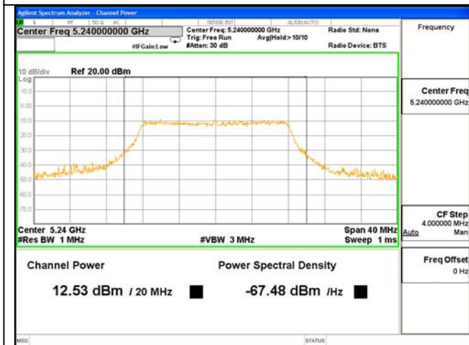
Test Mode: 802.11AC(20)---5240
