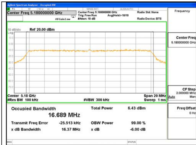
6dB Bandwidth Test Mode: 802.11AC(20)--5180
