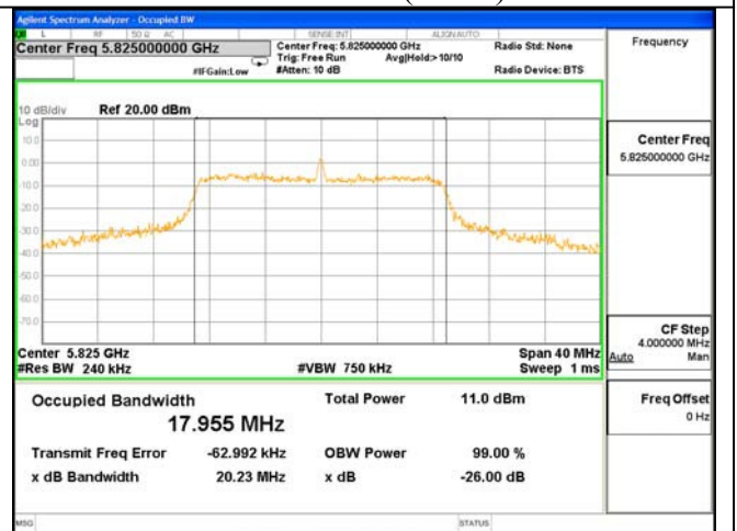
26dB & 99% Bandwidth Test Mode: 802.11n(HT20)---5825
