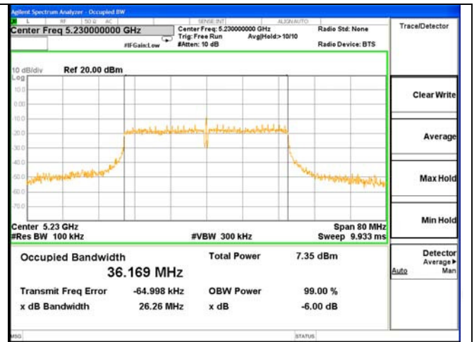
6dB Bandwidth Test Mode: 802.11n(HT40)---5230
