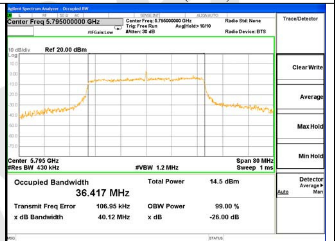
26dB & 99% Bandwidth Test Mode: 802.11n(HT40)---5795
