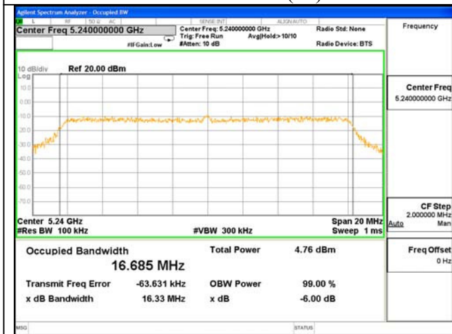
6dB Bandwidth Test Mode: 802.11AC(20)--5240
