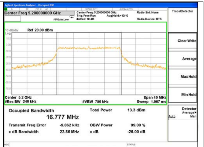
26dB & 99% Bandwidth Test Mode: 802.11AC(20)---5200
