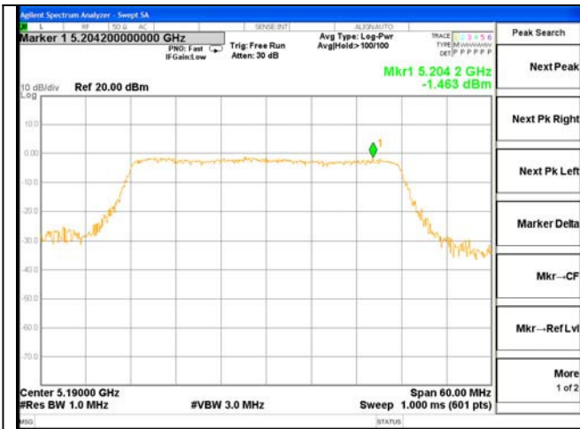
Test Mode: 802.11n(HT40)---5190
