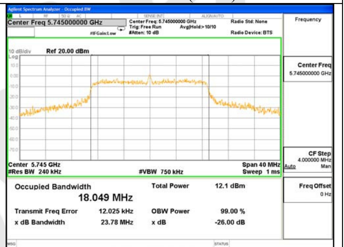
26dB & 99% Bandwidth Test Mode: 802.11n(HT20)---5745
