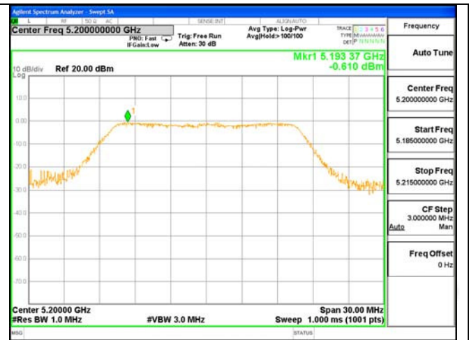
Test Mode: 802.11AC(20)---5200
