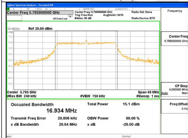
26dB & 99% Bandwidth Test Mode: 802.11AC(20)--5785
