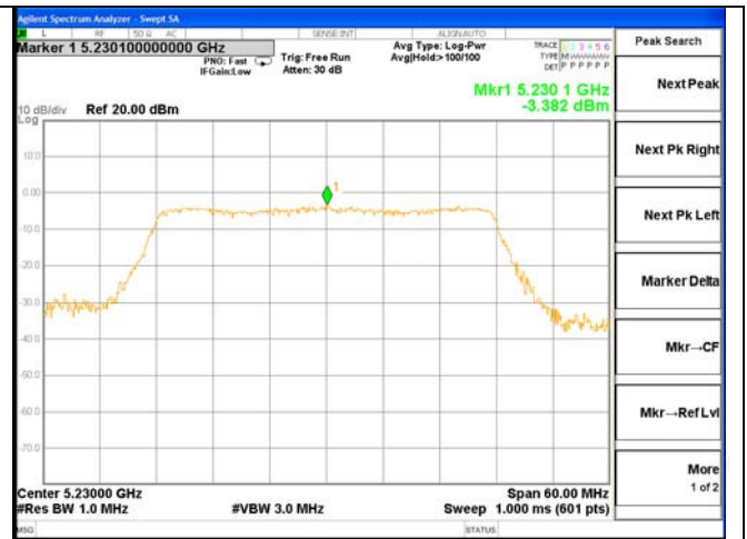
Test Mode: 802.11n(HT40)---5230
