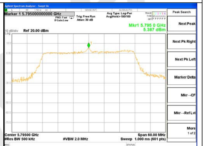
Test Mode: 802.11n(HT40)---5795
