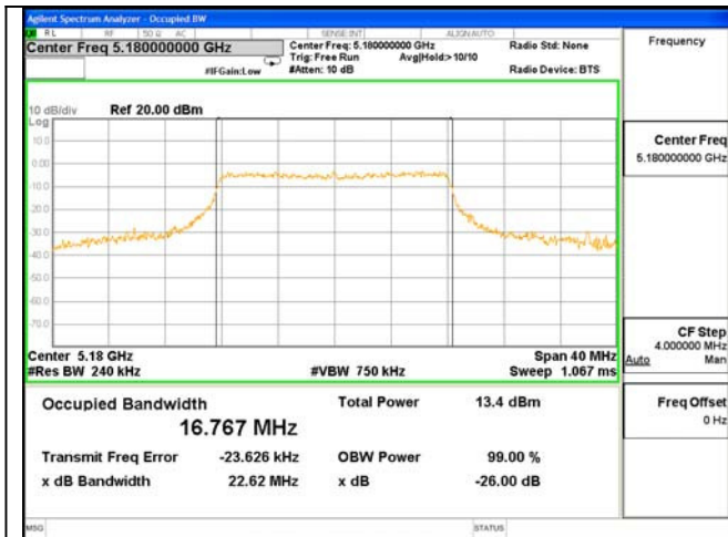
26dB & 99% Bandwidth Test Mode: 802.11AC(20)--5180
