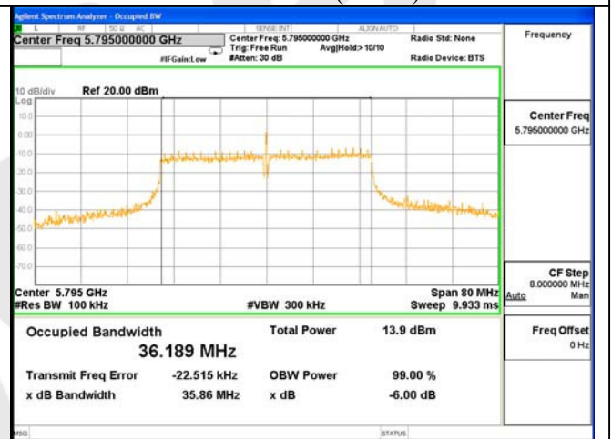
6dB Bandwidth Test Mode: 802.11n(HT40)---5795
