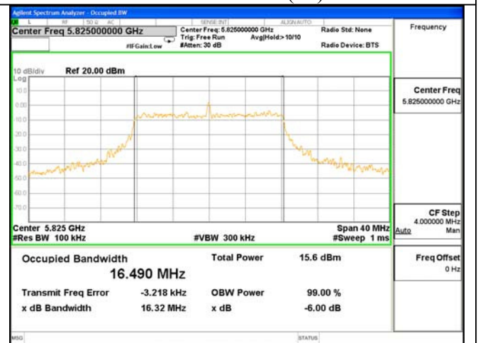
6dB Bandwidth Test Mode: 802.11AC(20)---5825
