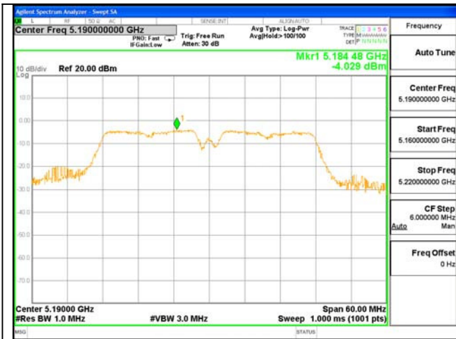
Test Mode: 802.11AC(40)---5190
