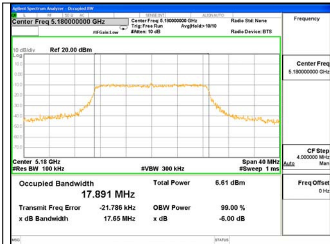
6dB Bandwidth Test Mode: 802.11n(HT20)--5180
