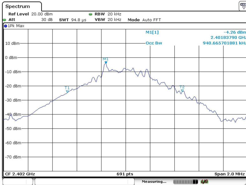
2402MHz, GFSK
