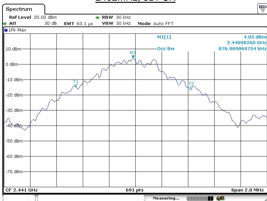
2441MHz, GFSK
