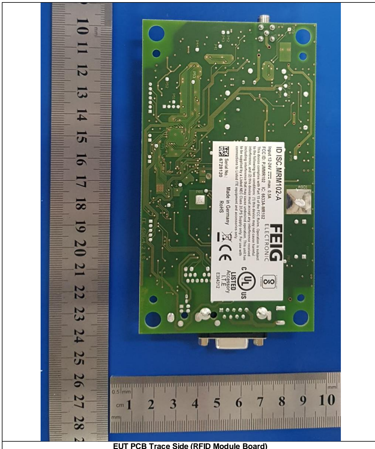
EUT PCB Trace Side (RFID Module Board)
