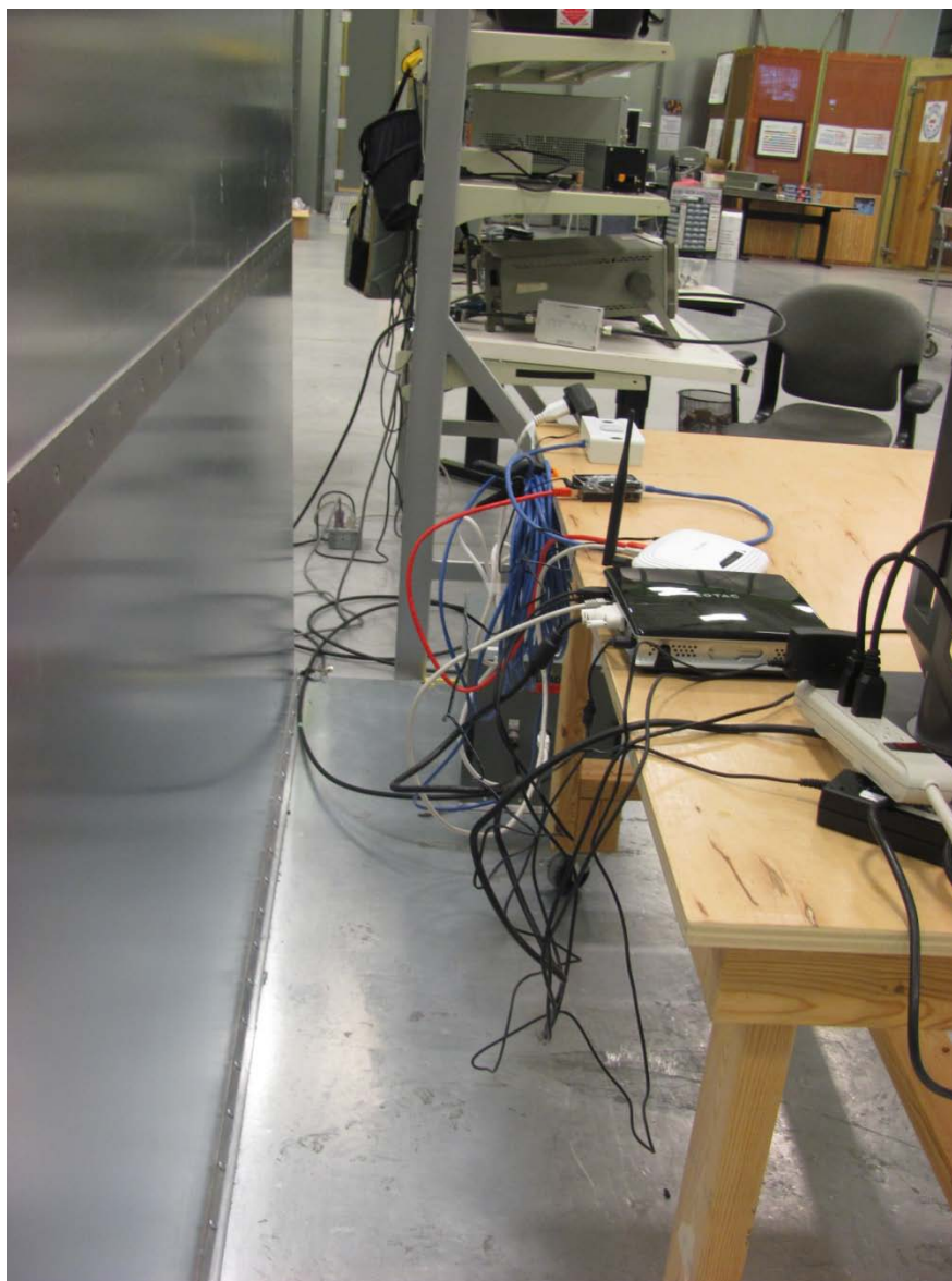
Figure 6: Power line conducted emission setup – photo 2
