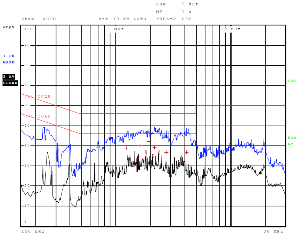
Figure 1 AC Line Conducted emissions of EUT line 1 (EUT – CPU)
