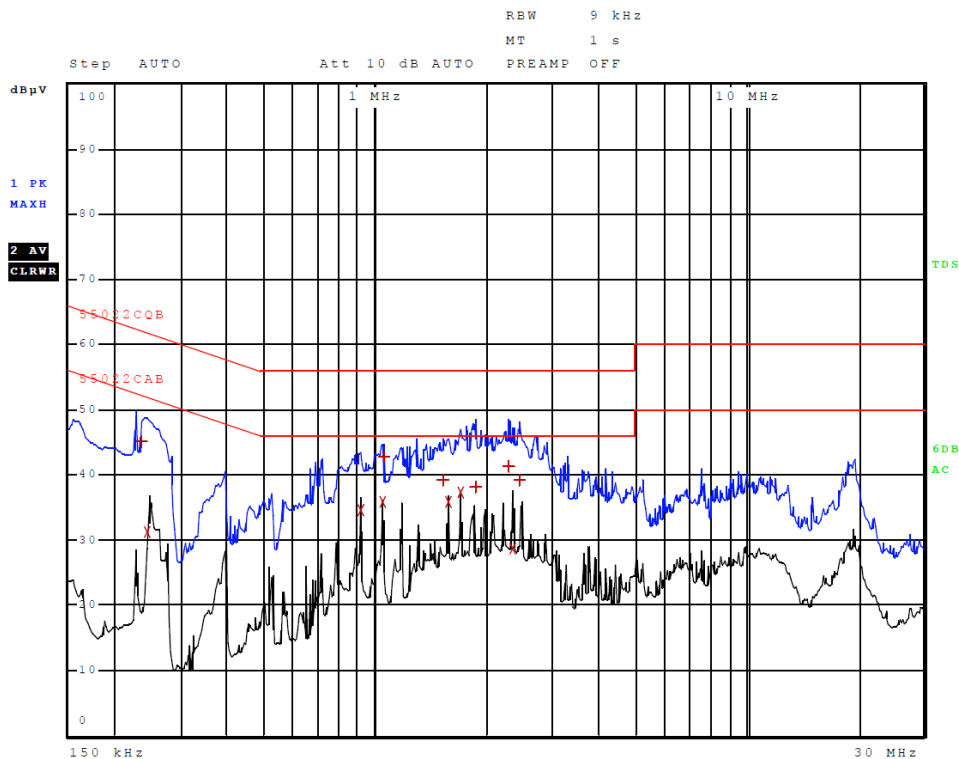
Figure 2 AC Line Conducted emissions of EUT line 2 (EUT – CPU)
