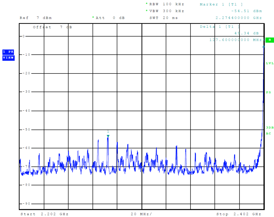
Figure 5 Plot of Transmitter Emissions (Low Band Edge, BT GFSK)
