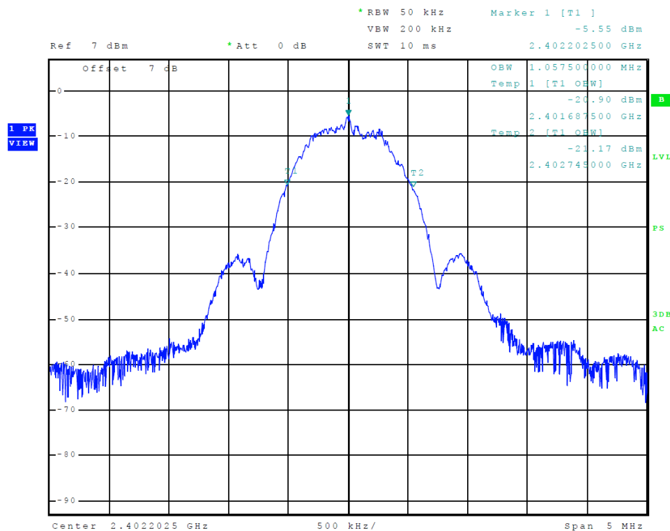
Figure 4 Plot of Transmitter Emissions (99% Occupied Bandwidth, BT GFSK)
