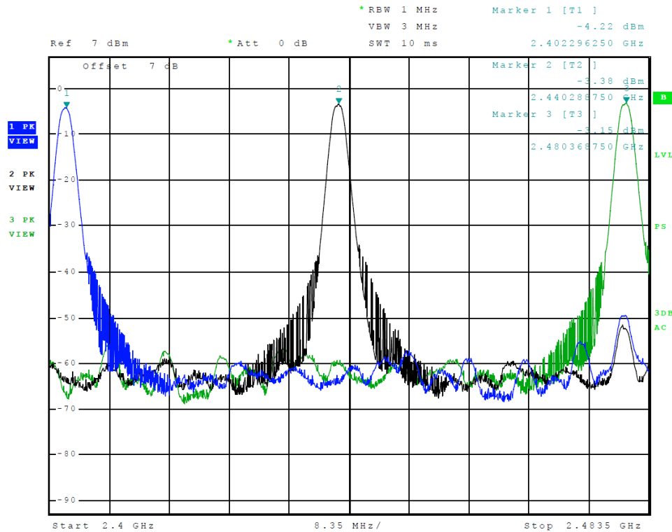
Figure 3 Plot of Transmitter Emissions (Operation in 2402-2480 MHz, BT GFSK)
