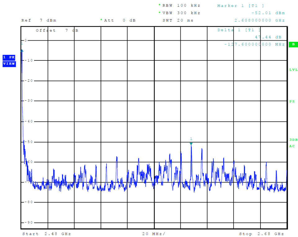
Figure 6 Plot of Transmitter Emissions (High Band Edge, BT GFSK)
