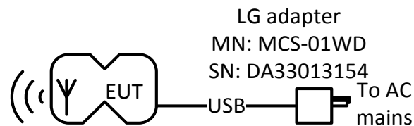
Figure 3.6-1: Setup diagram
