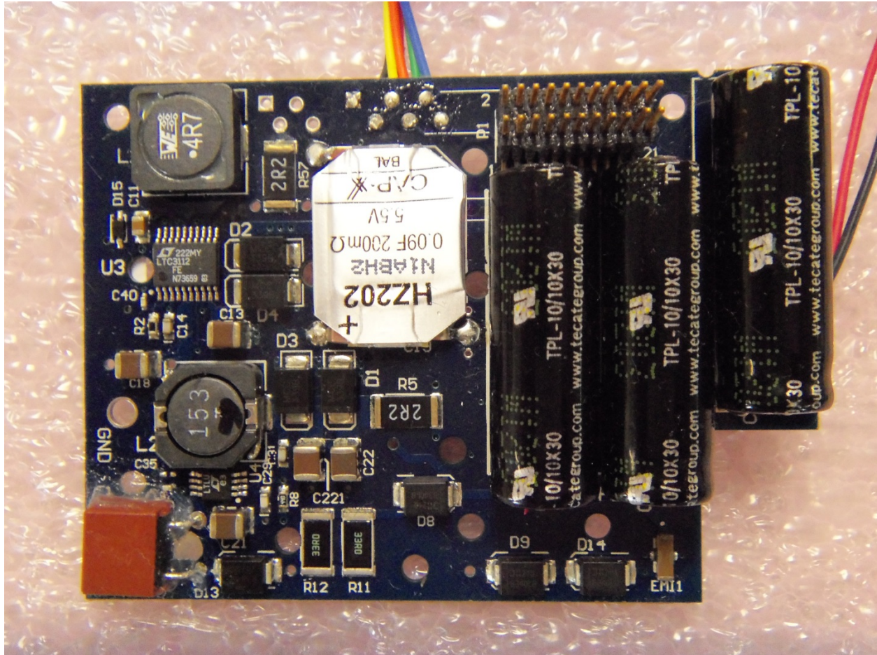
Power Supply Circuit Board, Top
