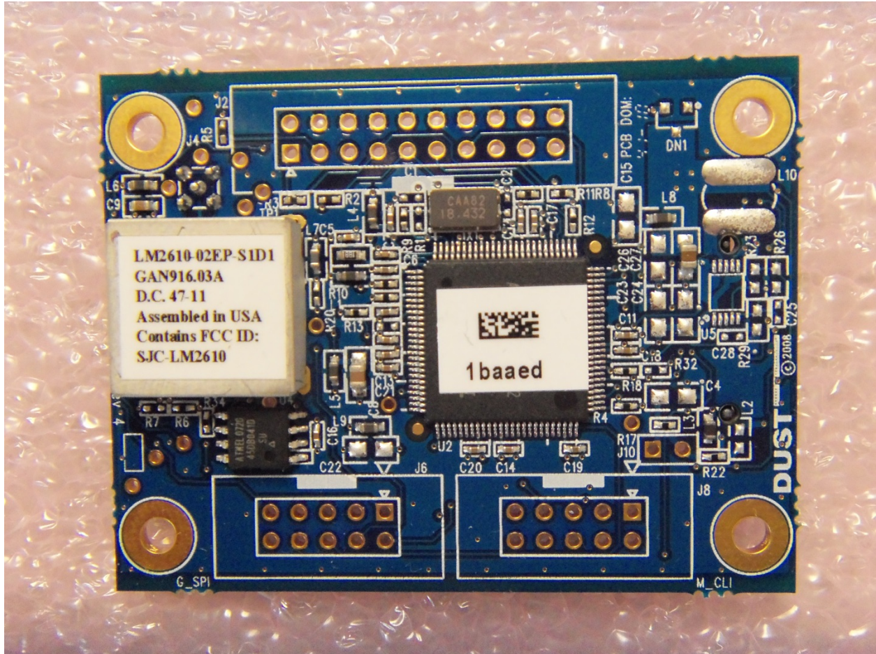
LM2610 Circuit Board, Top
