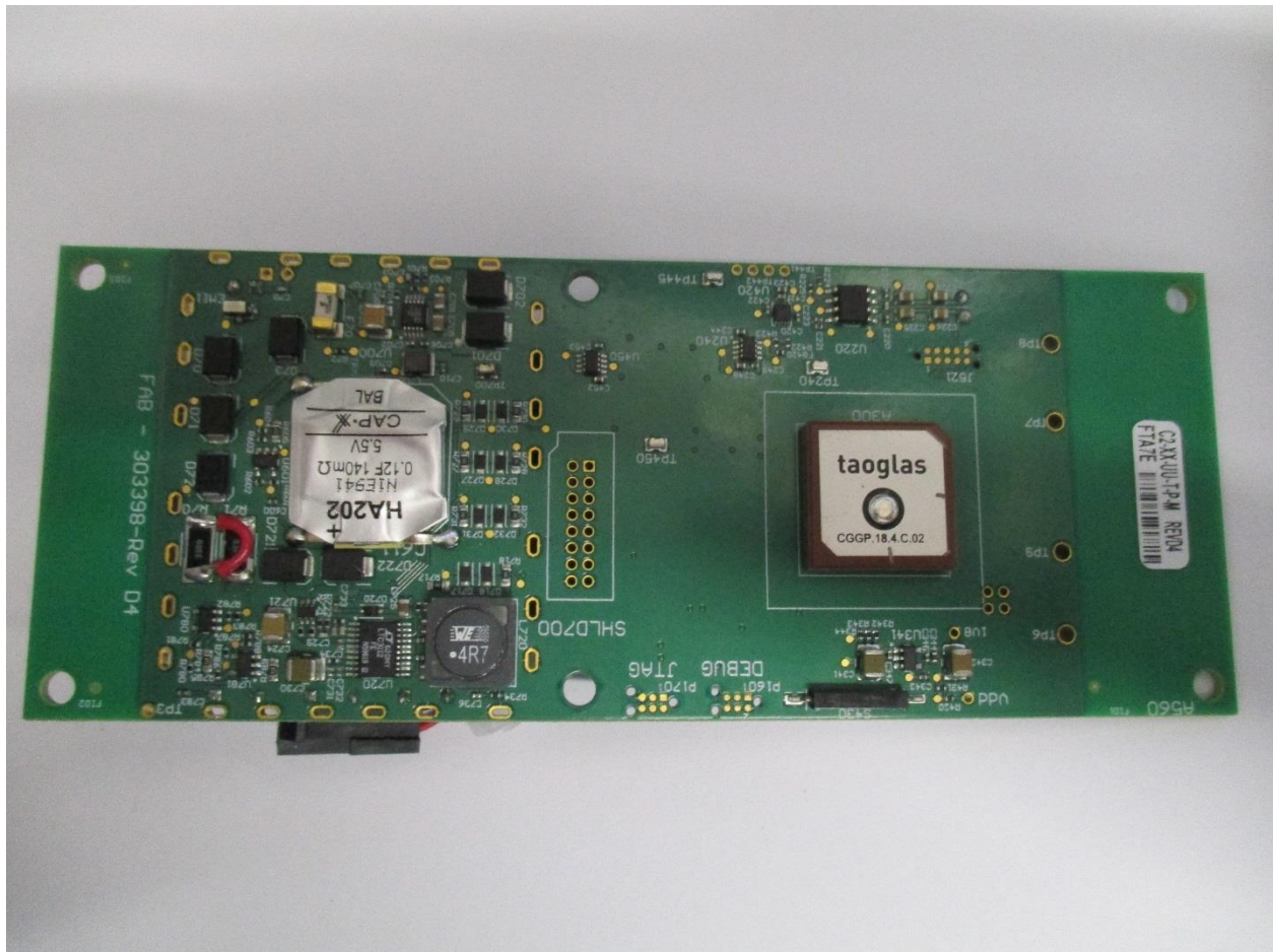
RF Shield Removed
