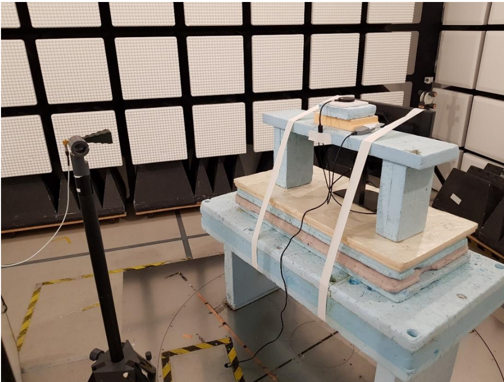
Radiated measurements 18-26.5 GHz
