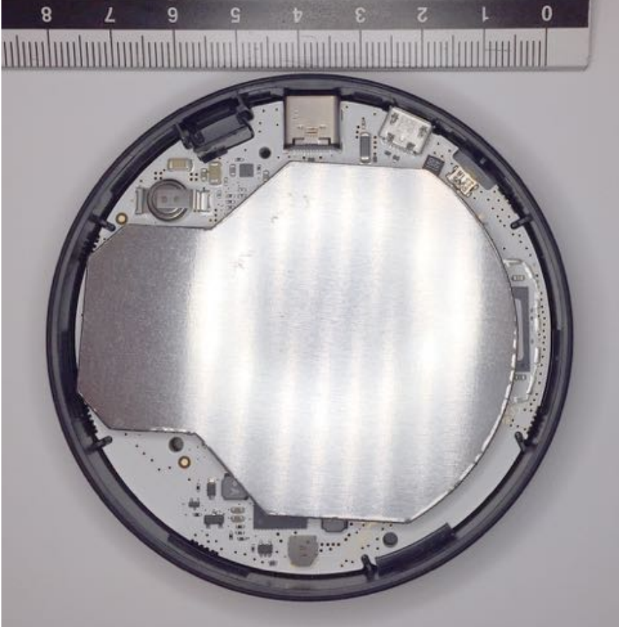
Top assembly with PCB
