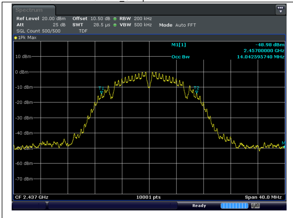
Test mode : 802.11b / 2 437 MHz_Occupied Bandwidth
