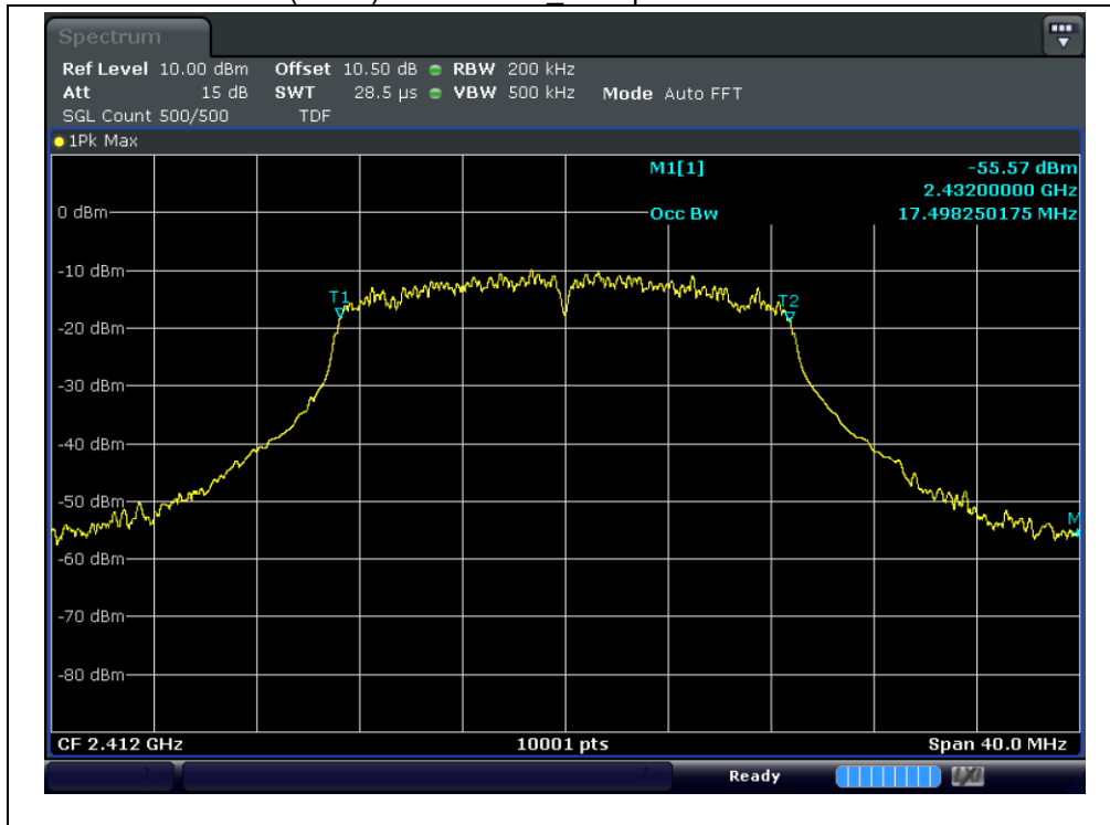
Test mode : 802.11n(HT20) / 2 412 MHz_Occupied Bandwidth
