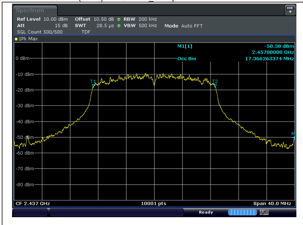
Test mode : 802.11n(HT20) / 2 437 MHz_Occupied Bandwidth
