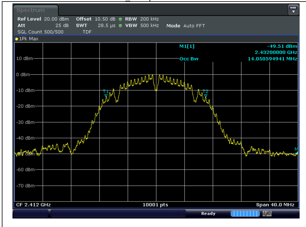
Test mode : 802.11b / 2 412 MHz_Occupied Bandwidth
