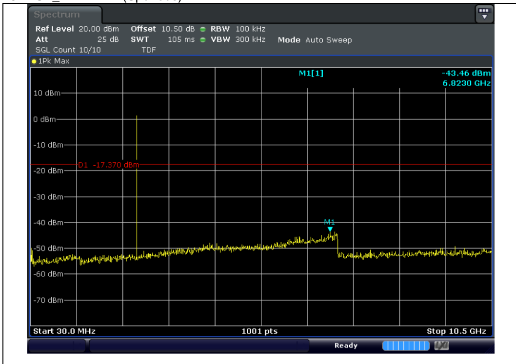
8DPSK_2 441 MHz(Spurious)
