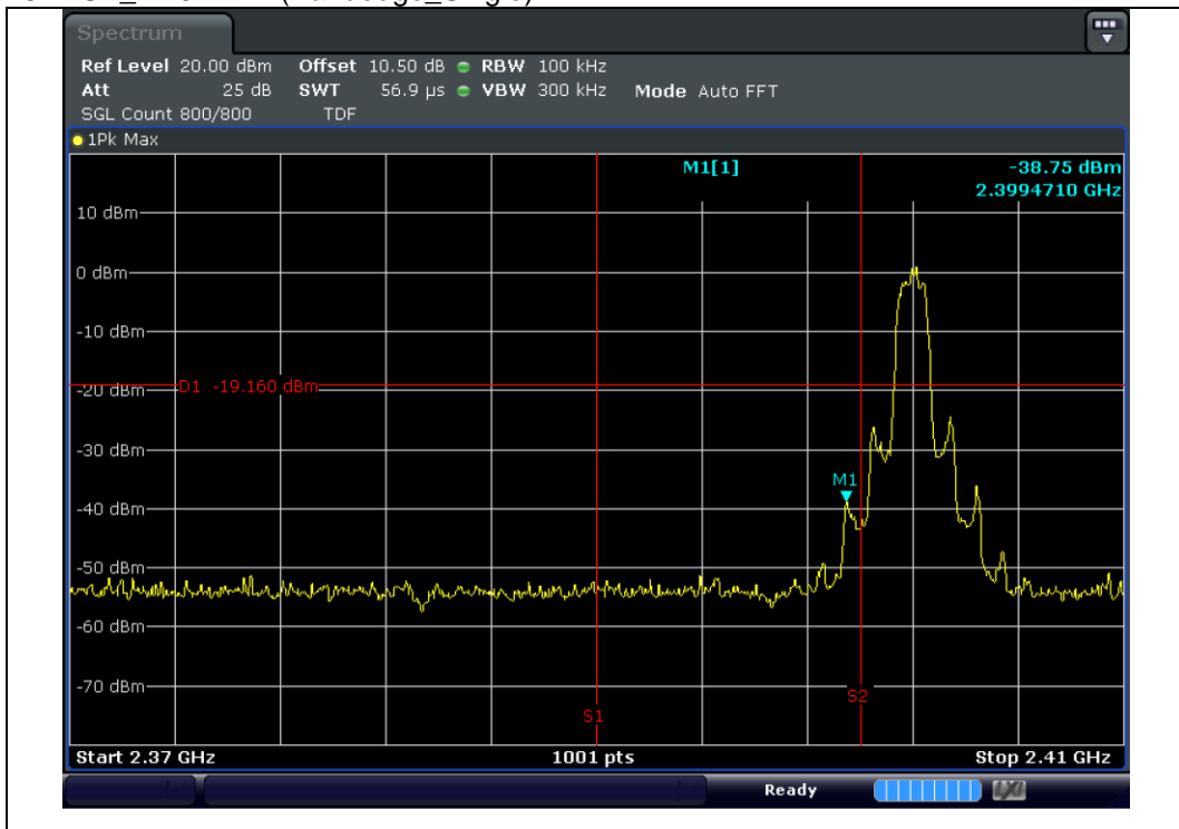
8DPSK_2 402 MHz(Bandedge_Single)
