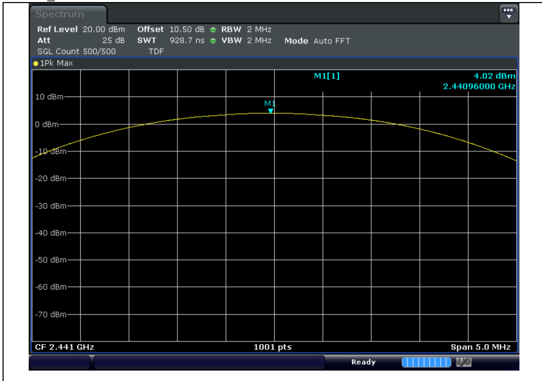
GFSK_2 441 MHz
