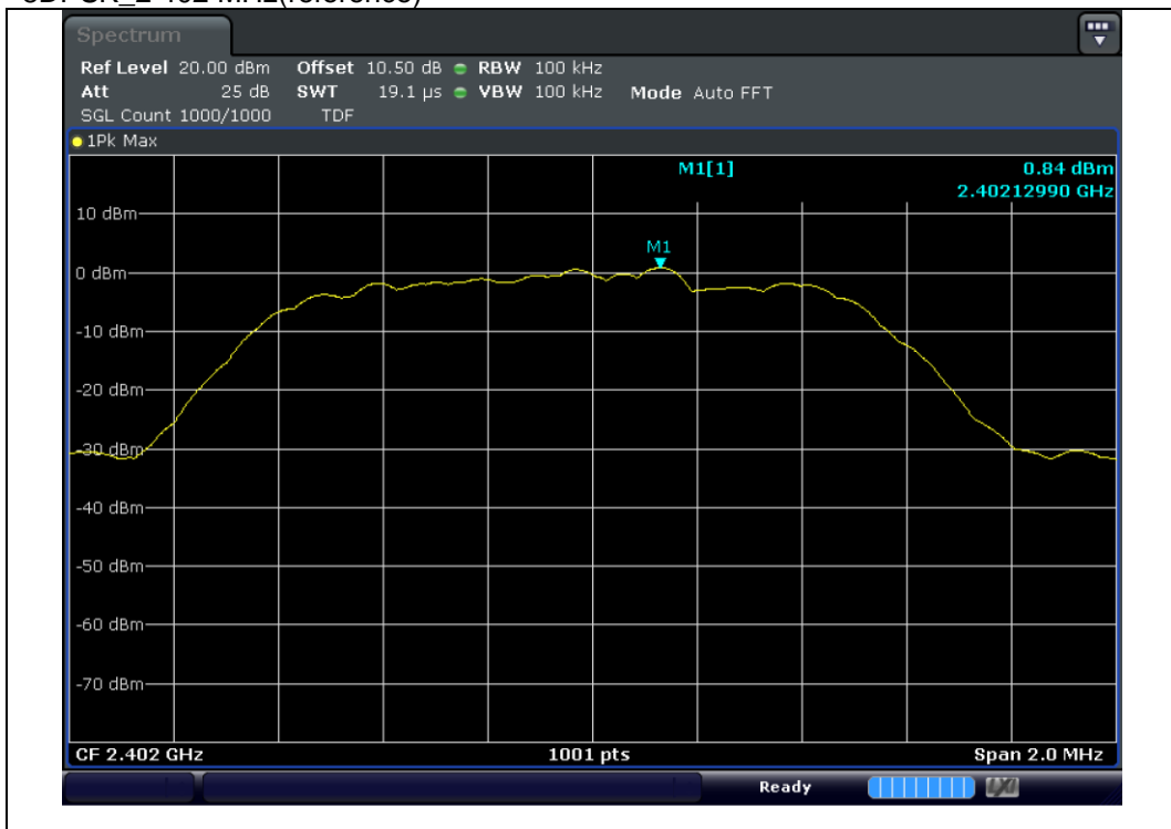
8DPSK_2 402 MHz(reference)
