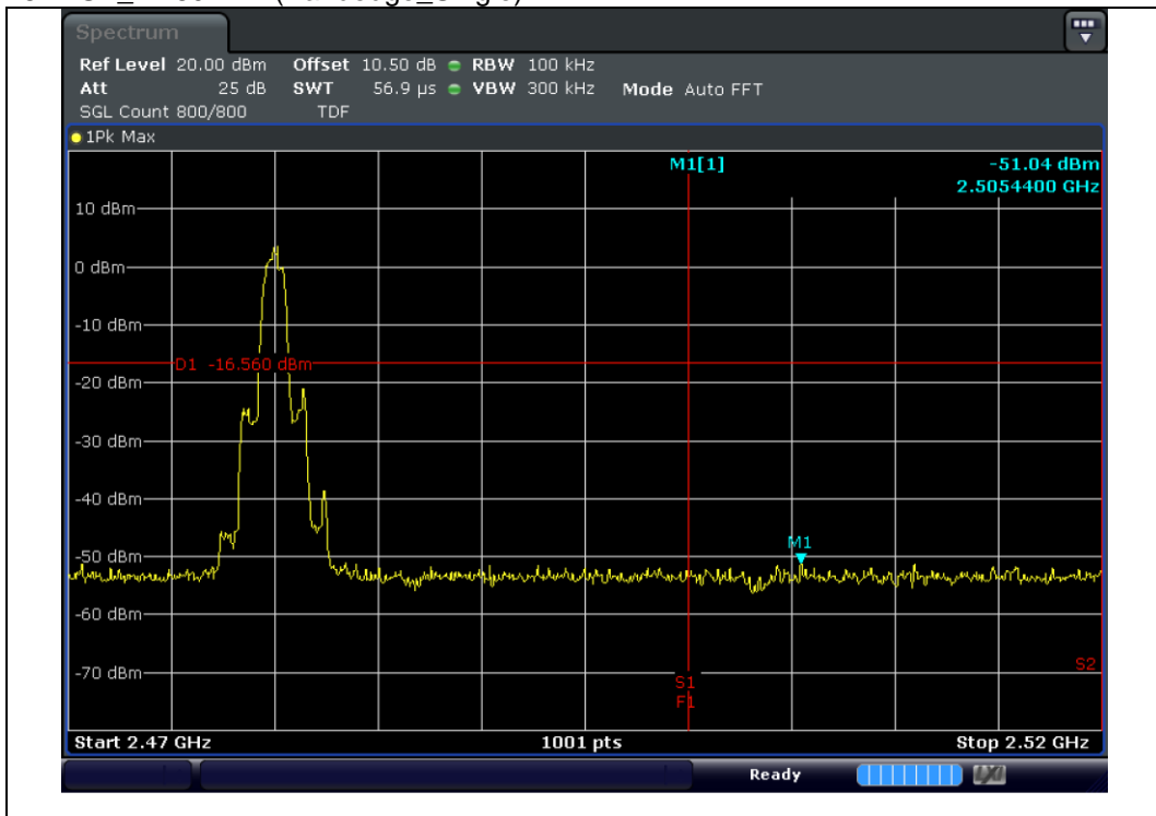
8DPSK_2 480 MHz(Bandedge_Single)
