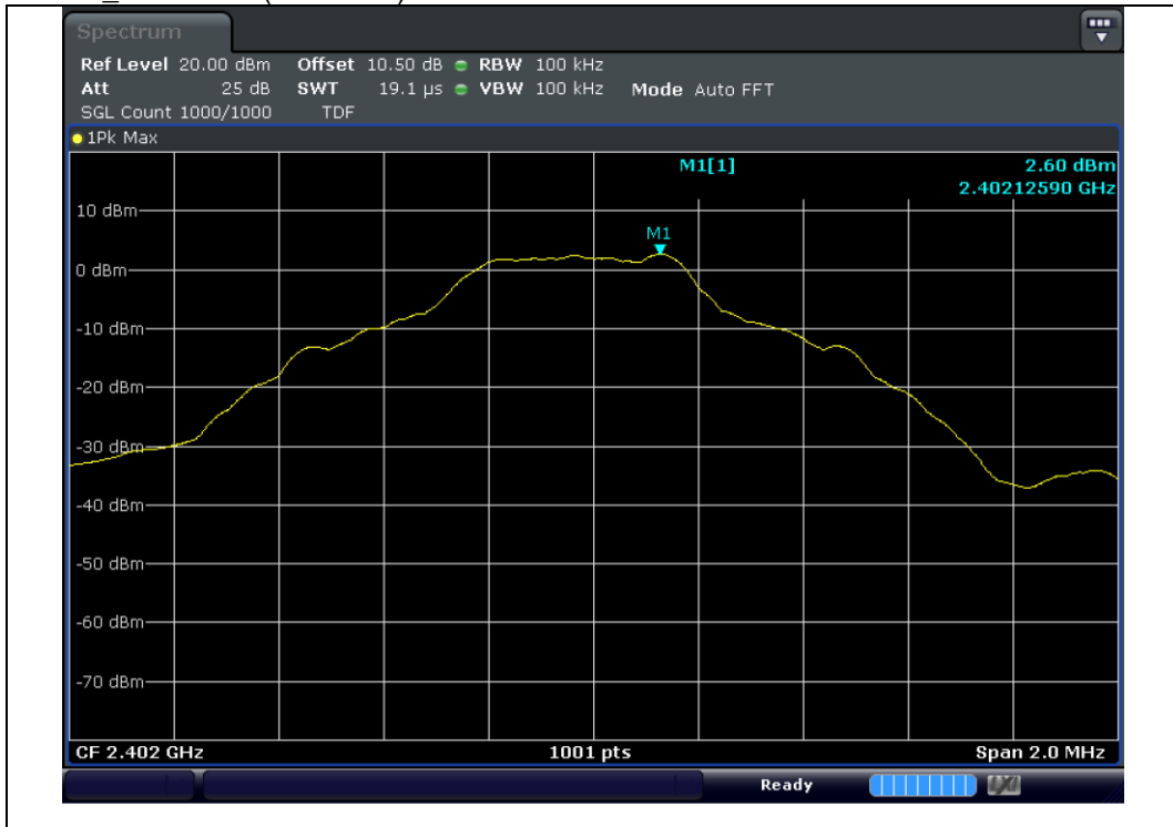
GFSK_2 402 MHz(reference)
