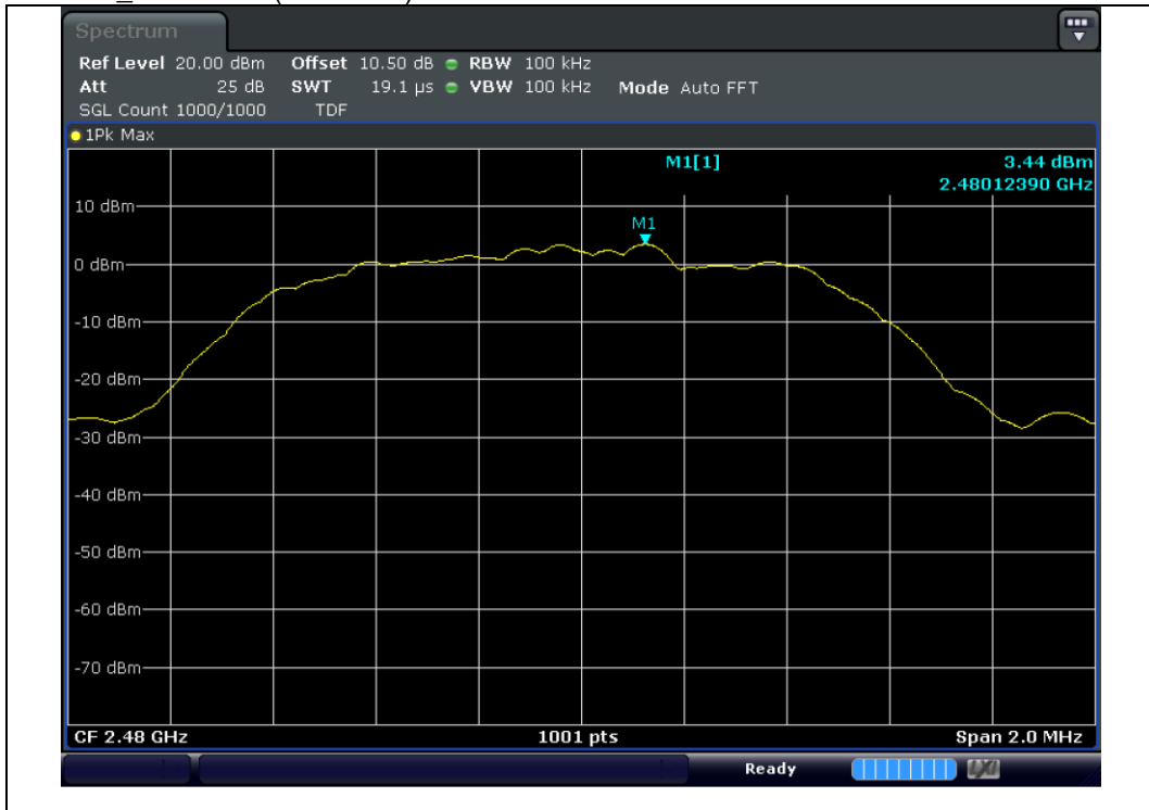
8DPSK_2 480 MHz(reference)
