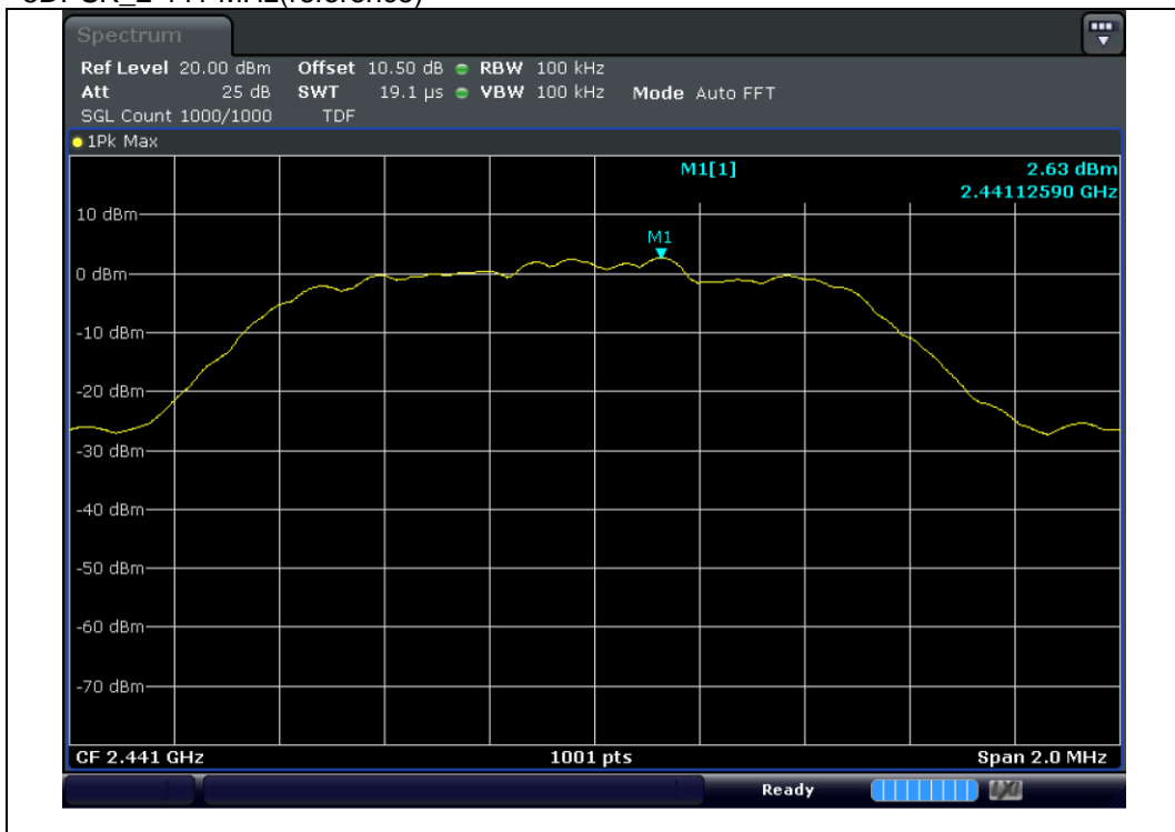
8DPSK_2 441 MHz(reference)
