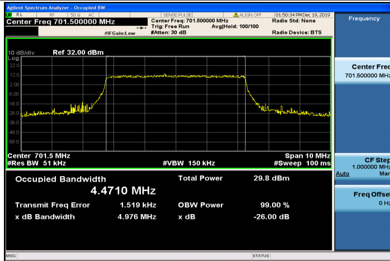
Band12-5MHz-QPSK-23035-25RB#0-4.4710
