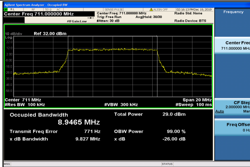
Band12-10MHz-16QAM-23130-50RB#0-8.9465
