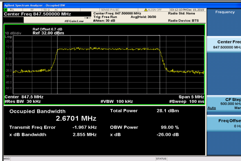
Band5-3MHz-16QAM-20635-15RB#0-2.6701
