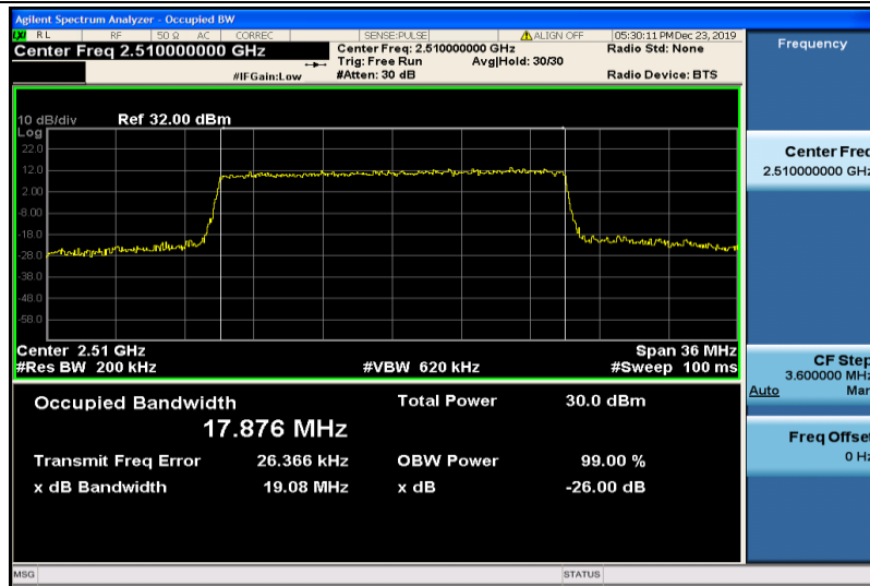
Band7-20MHz-16QAM-20850-100RB#0-17.876
