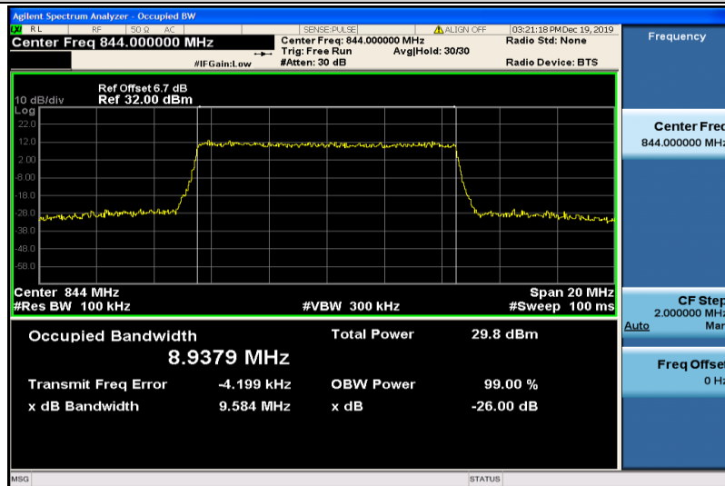
Band5-10MHz-QPSK-20600-50RB#0-8.9379
