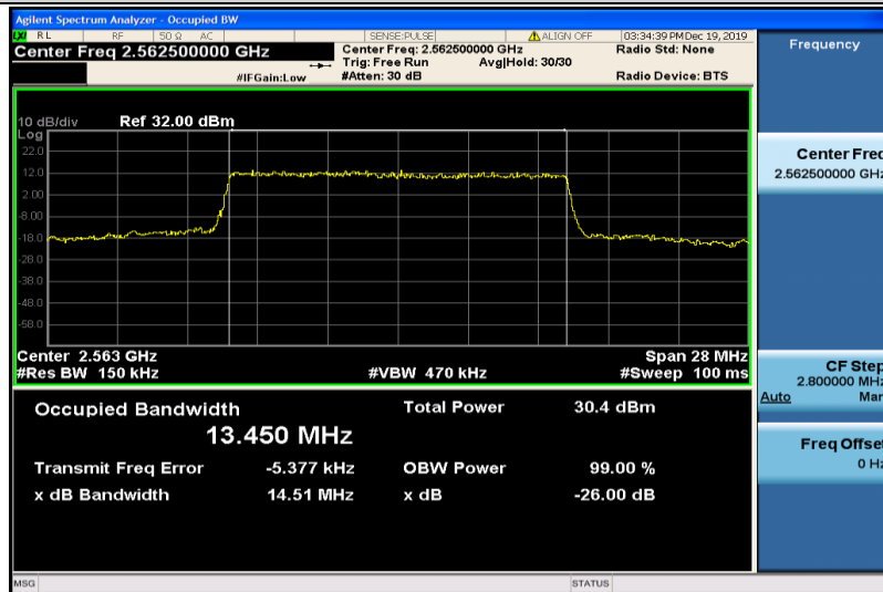
Band7-15MHz-QPSK-21375-75RB#0-13.450
