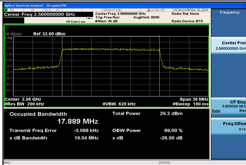
Band7-20MHz-16QAM-21350-100RB#0-17.889
