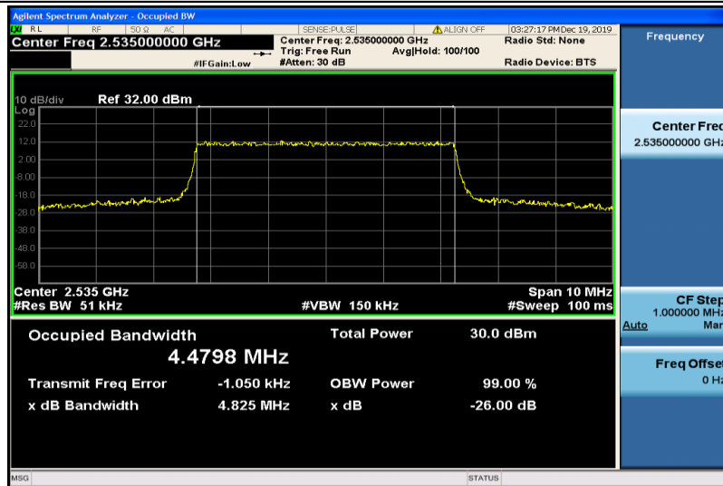
Band7-5MHz-QPSK-21100-25RB#0-4.4798
