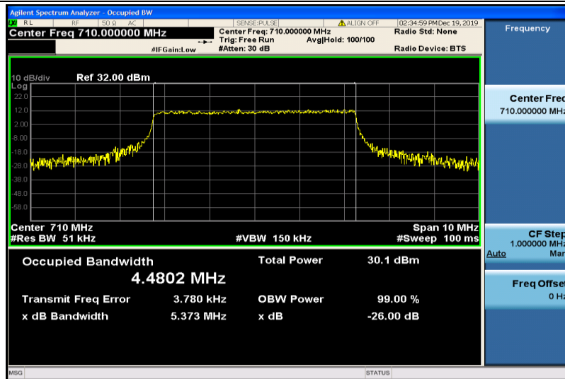
Band17-5MHz-QPSK-23790-25RB#0-4.4802
