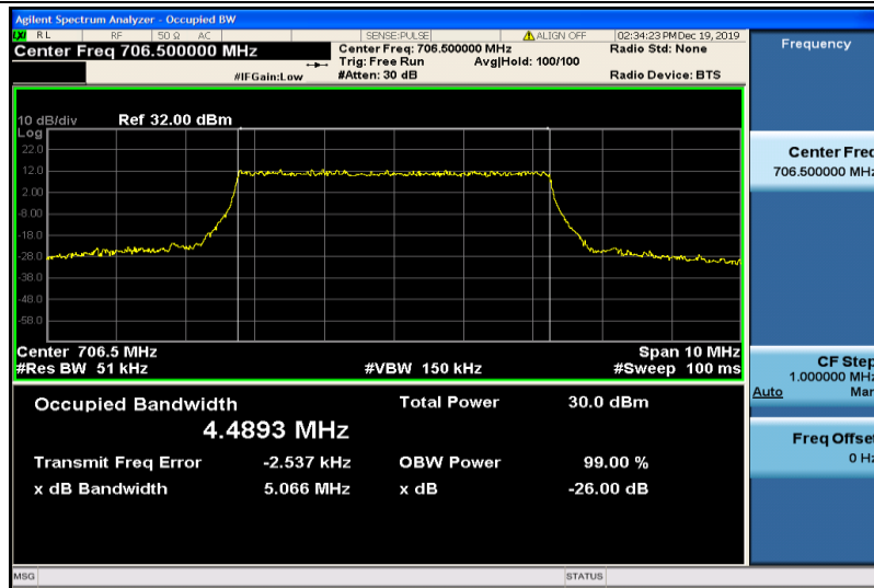
Band17-5MHz-QPSK-23755-25RB#0-4.4893
