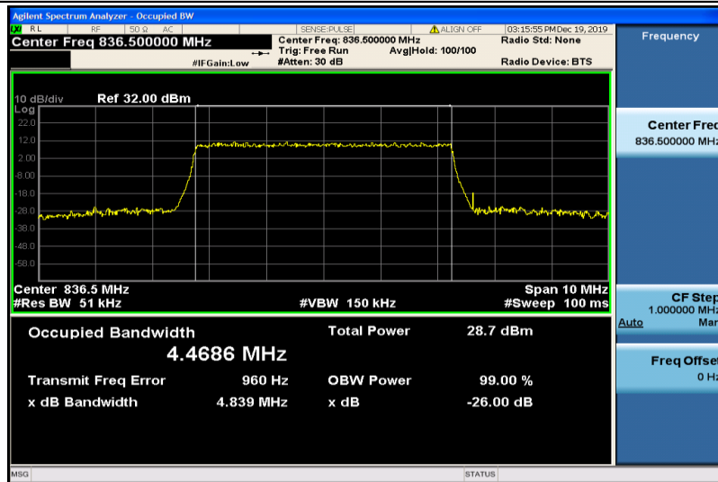
Band5-5MHz-16QAM-20525-25RB#0-4.4686
