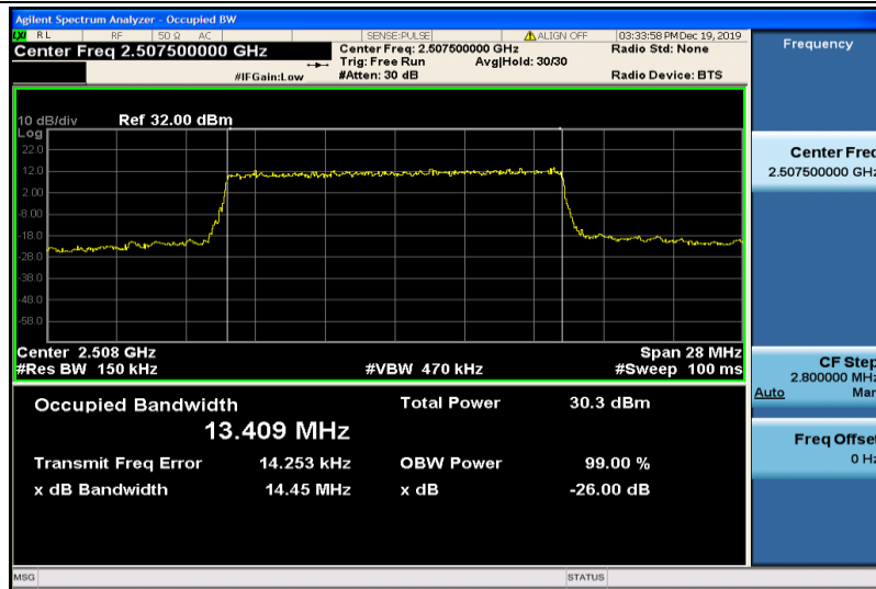
Band7-15MHz-QPSK-20825-75RB#0-13.409
