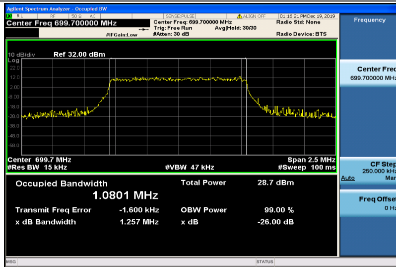
Band12-1.4MHz-QPSK-23017-6RB#0-1.0801
