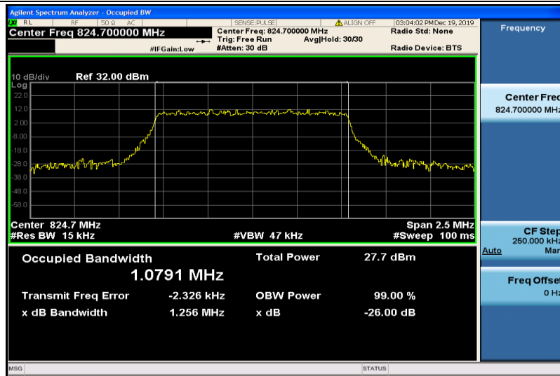
Band5-1.4MHz-16QAM-20407-6RB#0-1.0791
