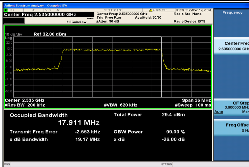
Band7-20MHz-16QAM-21100-100RB#0-17.911
