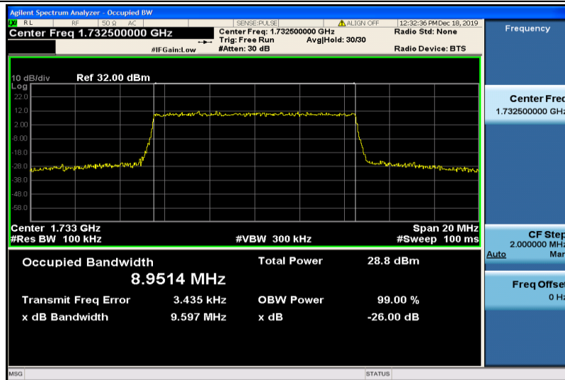
Band4-10MHz-16QAM-20175-50RB#0-8.9514
