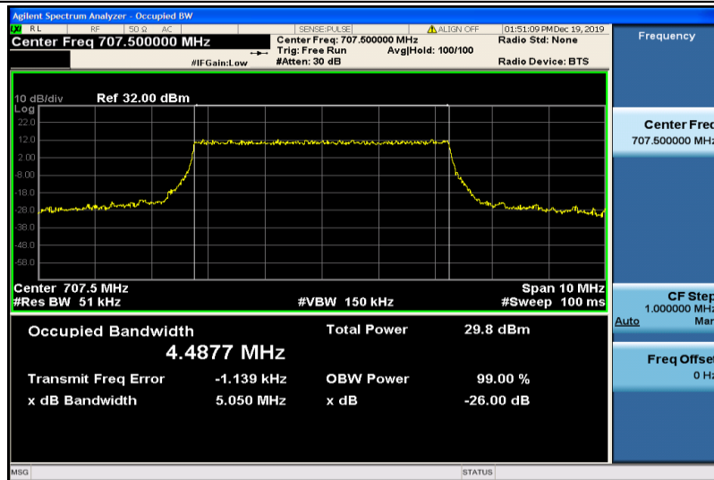
Band12-5MHz-QPSK-23095-25RB#0-4.4877
