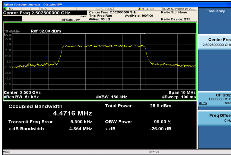
Band7-5MHz-16QAM-20775-25RB#0-4.4716
