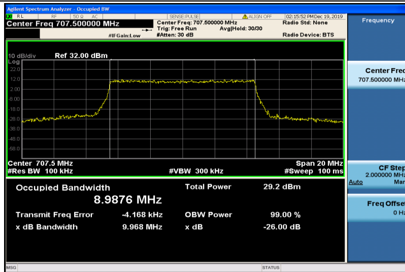
Band12-10MHz-16QAM-23095-50RB#0-8.9876
