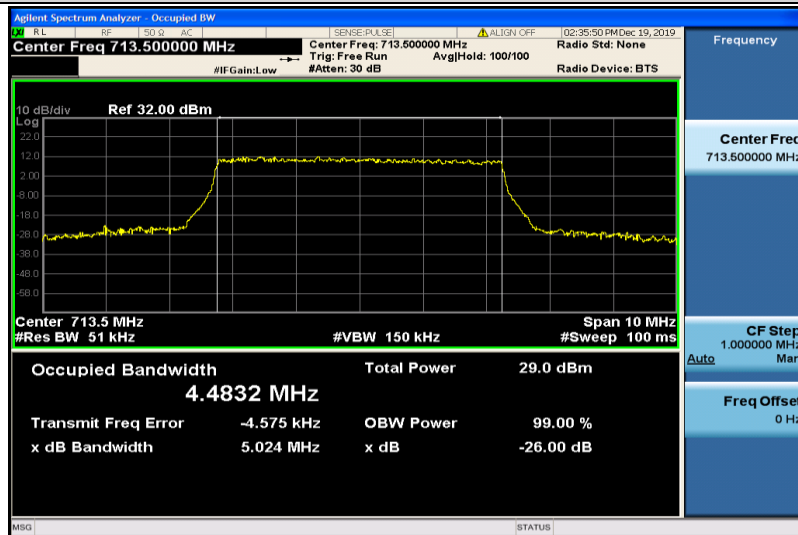
Band17-5MHz-16QAM-23825-25RB#0-4.4832
