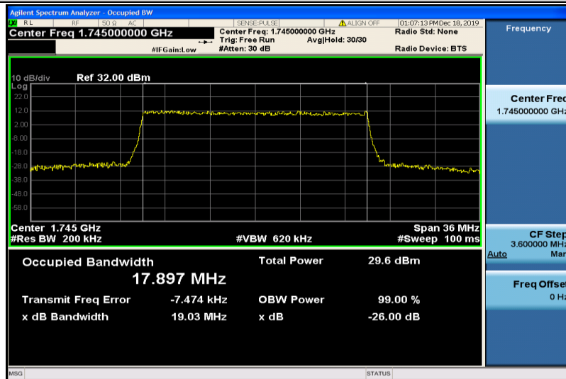
Band4-20MHz-16QAM-20300-100RB#0-17.897
