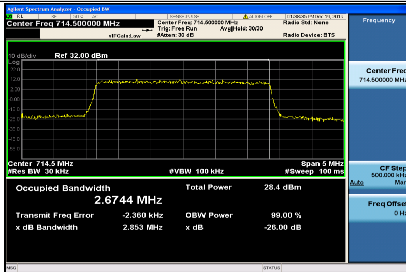
Band12-3MHz-16QAM-23165-15RB#0-2.6744
