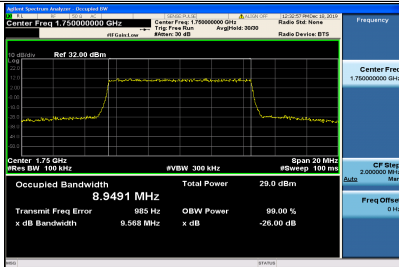
Band4-10MHz-16QAM-20350-50RB#0-8.9491
