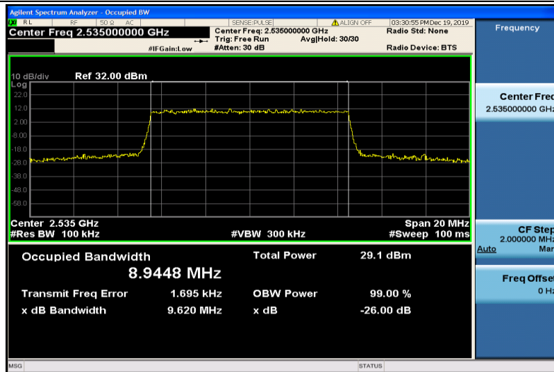
Band7-10MHz-16QAM-21100-50RB#0-8.9448
