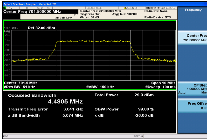
Band12-5MHz-16QAM-23035-25RB#0-4.4805
