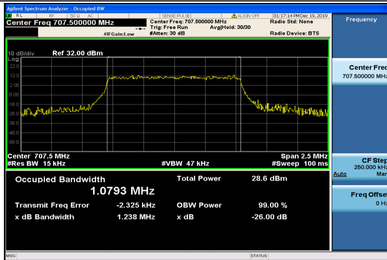
Band12-1.4MHz-QPSK-23095-6RB#0-1.0793
