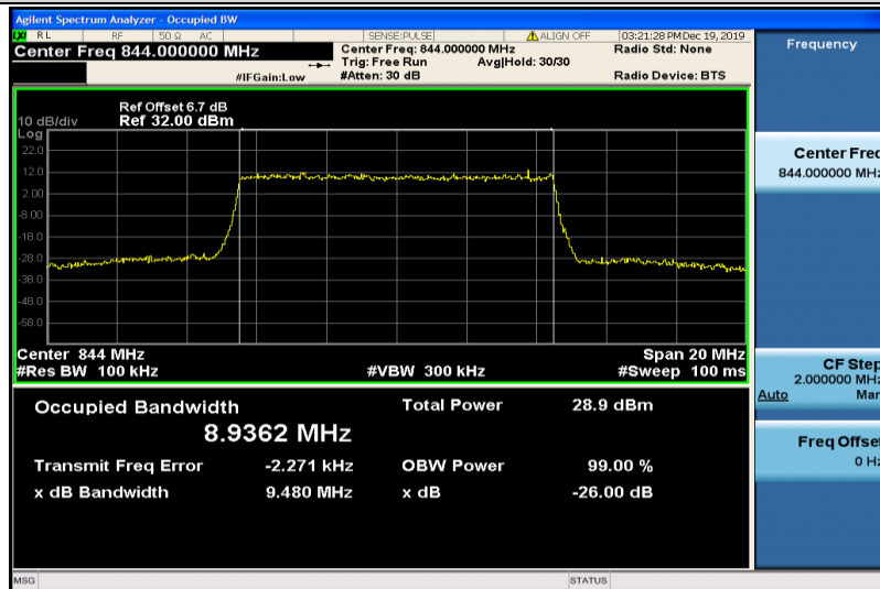
Band5-10MHz-16QAM-20600-50RB#0-8.9362
