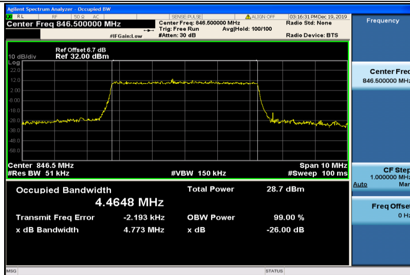
Band5-5MHz-16QAM-20625-25RB#0-4.4648
