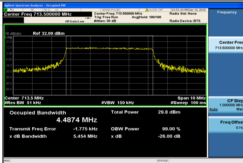
Band12-5MHz-QPSK-23155-25RB#0-4.4874
