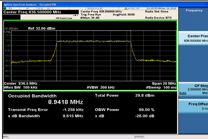
Band5-10MHz-QPSK-20525-50RB#0-8.9418
