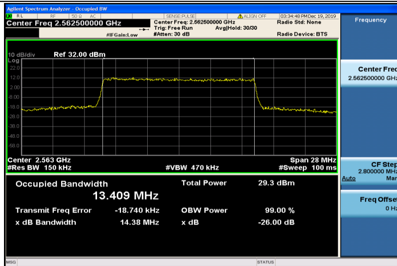
Band7-15MHz-16QAM-21375-75RB#0-13.409
