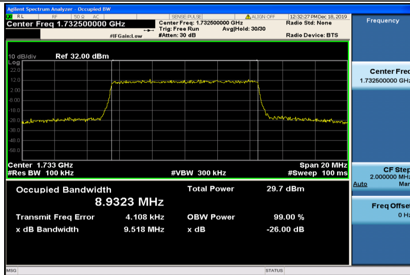
Band4-10MHz-QPSK-20175-50RB#0-8.9323
