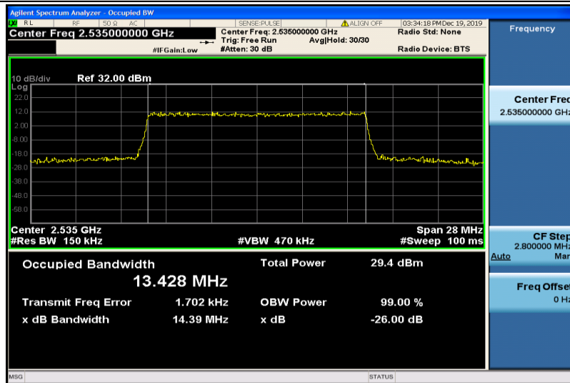
Band7-15MHz-QPSK-21100-75RB#0-13.428
