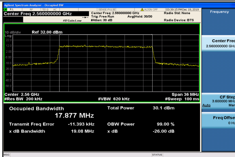
Band7-20MHz-QPSK-21350-100RB#0-17.877
