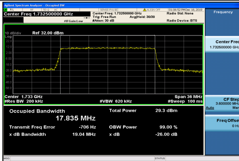
Band4-20MHz-16QAM-20175-100RB#0-17.835
