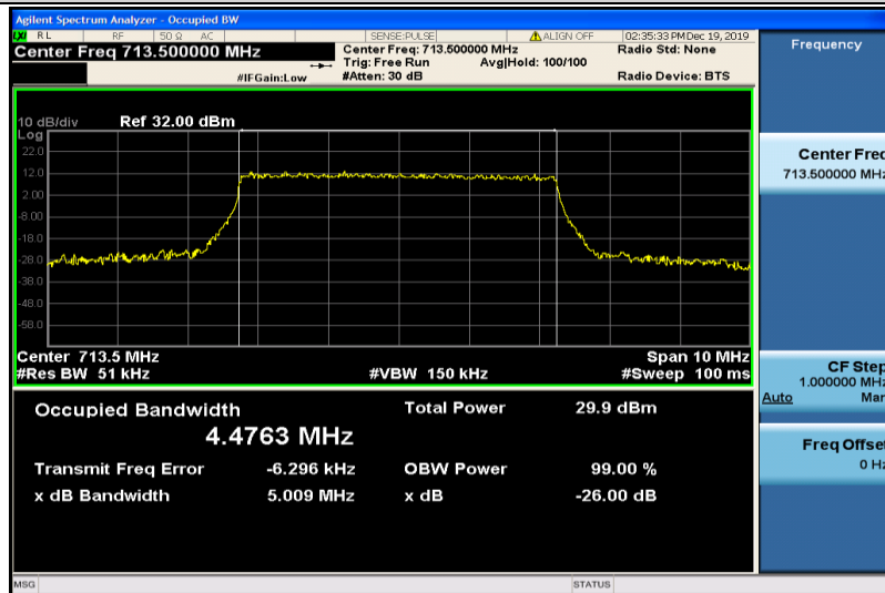
Band17-5MHz-QPSK-23825-25RB#0-4.4763
