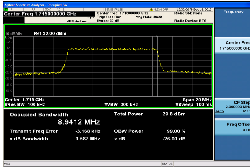
Band4-10MHz-QPSK-20000-50RB#0-8.9412
