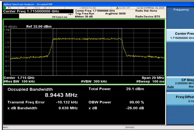
Band4-10MHz-16QAM-20000-50RB#0-8.9443
