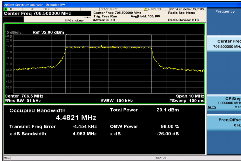
Band17-5MHz-16QAM-23755-25RB#0-4.4821
