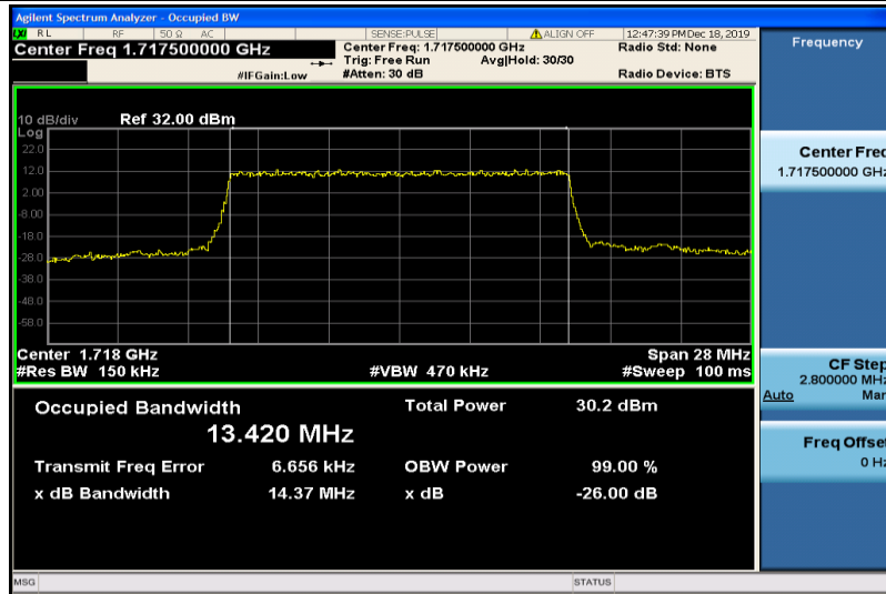
Band4-15MHz-QPSK-20025-75RB#0-13.420
