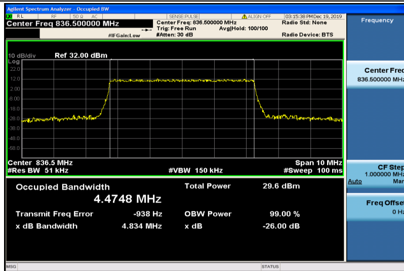
Band5-5MHz-QPSK-20525-25RB#0-4.4748
