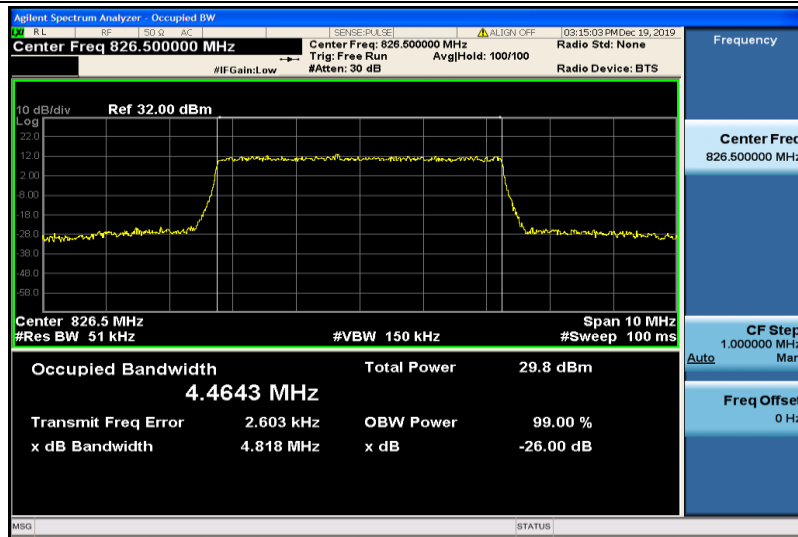
Band5-5MHz-QPSK-20425-25RB#0-4.4643
