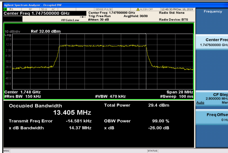
Band4-15MHz-16QAM-20325-75RB#0-13.405
