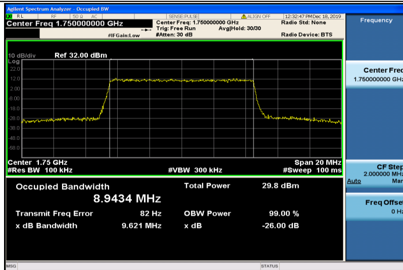
Band4-10MHz-QPSK-20350-50RB#0-8.9434
