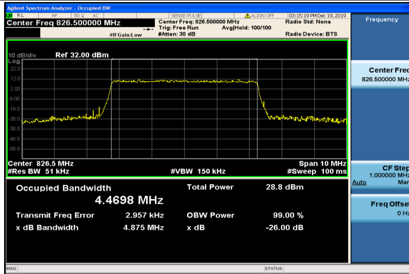
Band5-5MHz-16QAM-20425-25RB#0-4.4698
