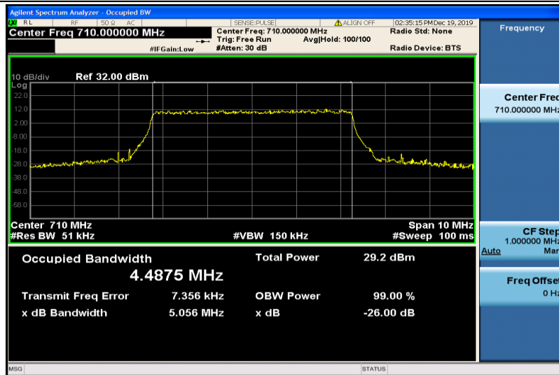
Band17-5MHz-16QAM-23790-25RB#0-4.4875
