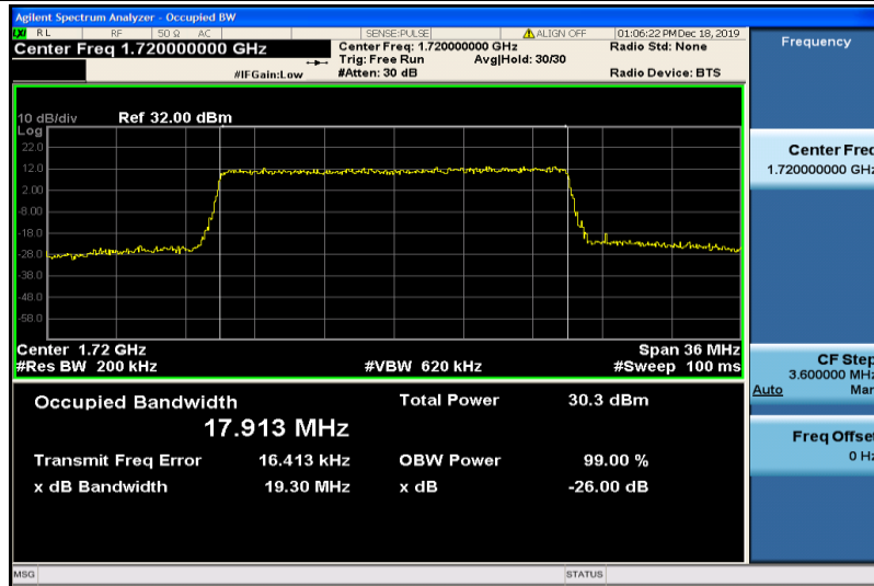
Band4-20MHz-QPSK-20050-100RB#0-17.913
