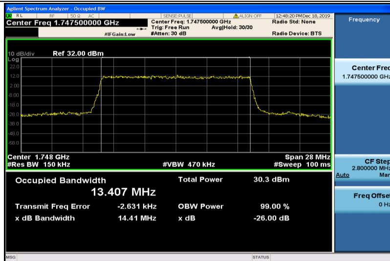
Band4-15MHz-QPSK-20325-75RB#0-13.407
