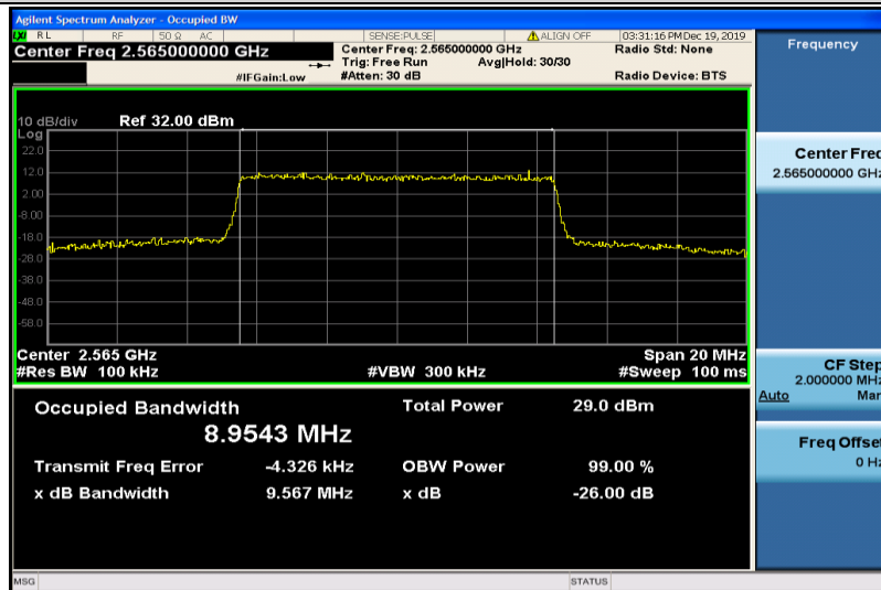
Band7-10MHz-16QAM-21400-50RB#0-8.9543
