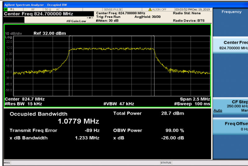
Band5-1.4MHz-QPSK-20407-6RB#0-1.0779
