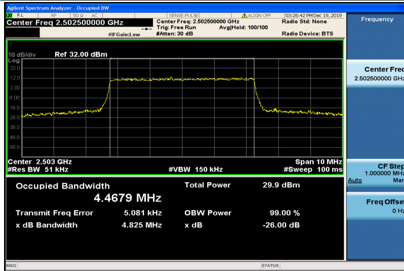
Band7-5MHz-QPSK-20775-25RB#0-4.4679
