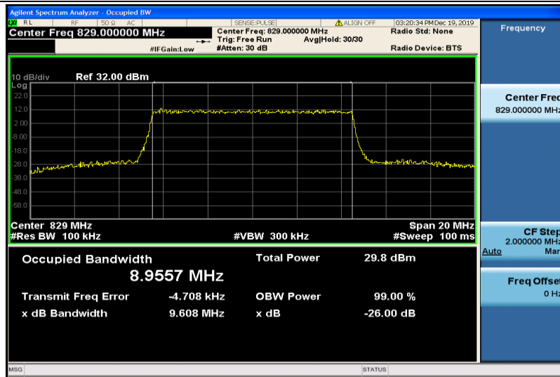
Band5-10MHz-QPSK-20450-50RB#0-8.9557
