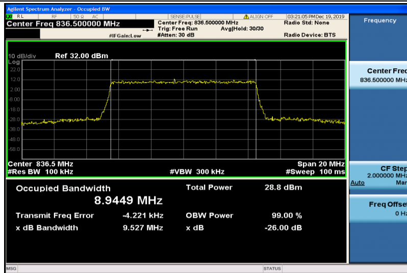
Band5-10MHz-16QAM-20525-50RB#0-8.9449
