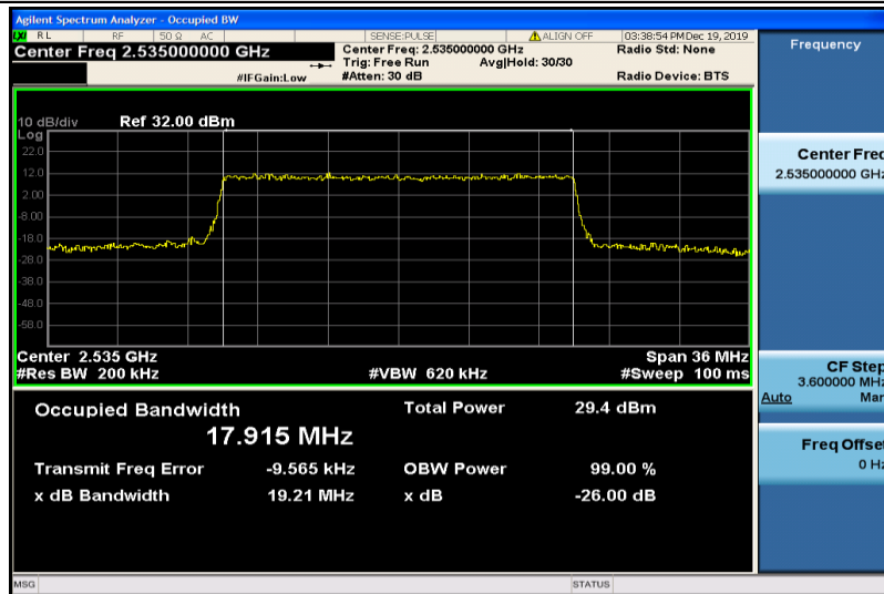
Band7-20MHz-QPSK-21100-100RB#0-17.915
