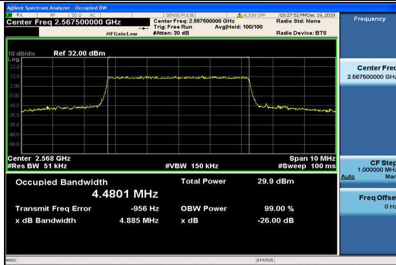
Band7-5MHz-QPSK-21425-25RB#0-4.4801
