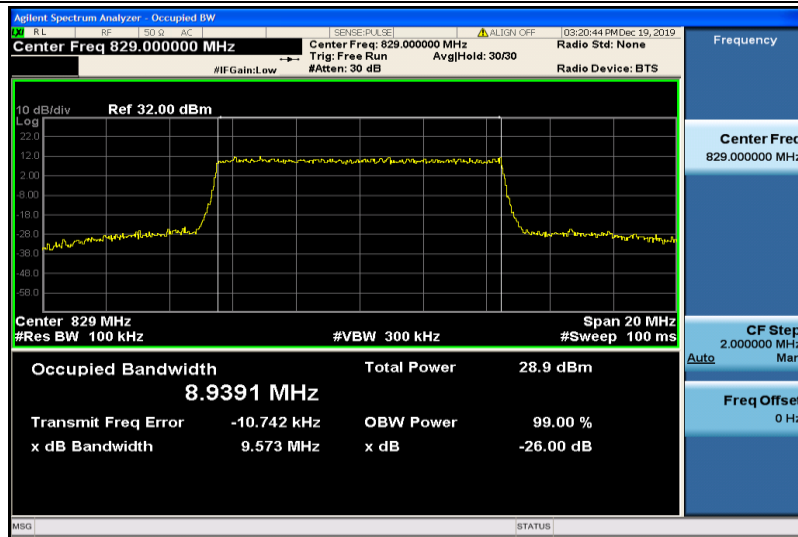
Band5-10MHz-16QAM-20450-50RB#0-8.9391
