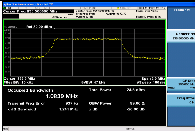
Band5-1.4MHz-QPSK-20525-6RB#0-1.0839
