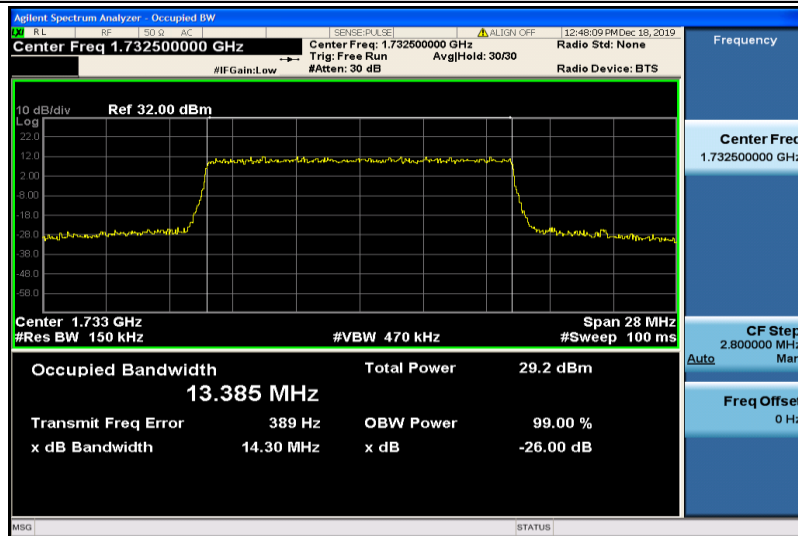
Band4-15MHz-16QAM-20175-75RB#0-13.385
