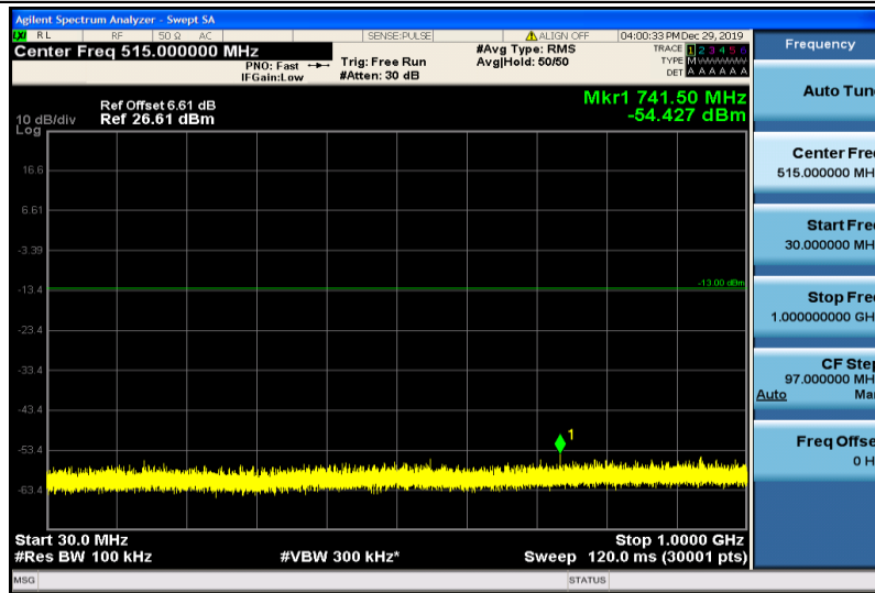
Band2-10MHz-16QAM-18650-1RB#0-30~1000MHz
