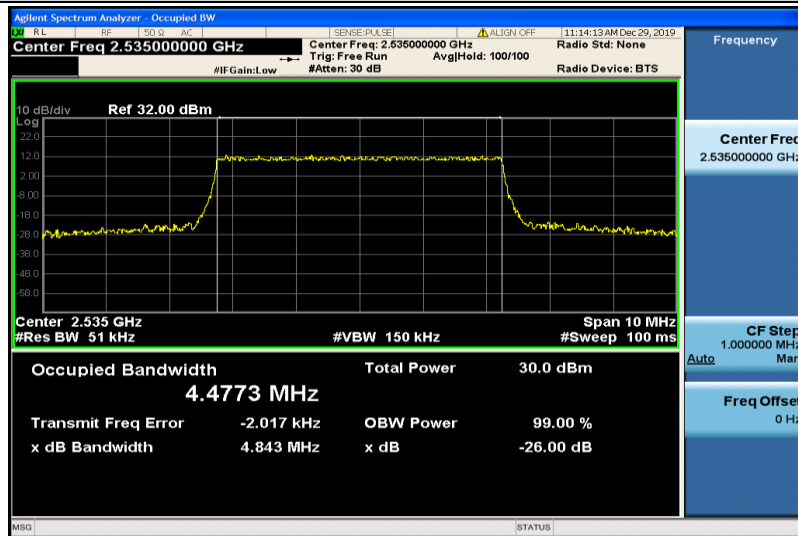
Band7-5MHz-QPSK-21100-25RB#0-4.4773
