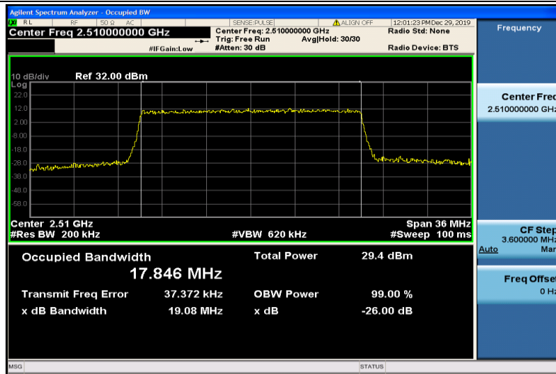
Band7-20MHz-16QAM-20850-100RB#0-17.846
