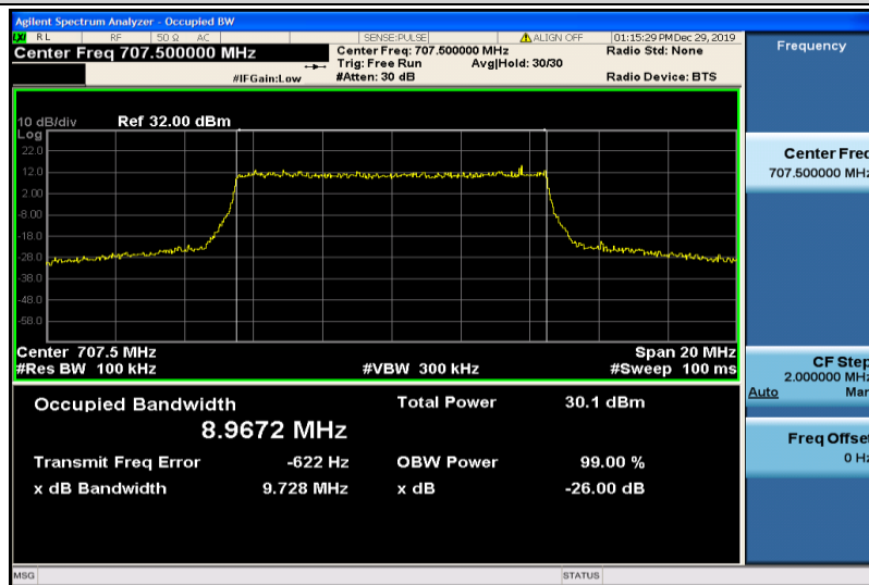
Band12-10MHz-16QAM-23095-50RB#0-8.9672
