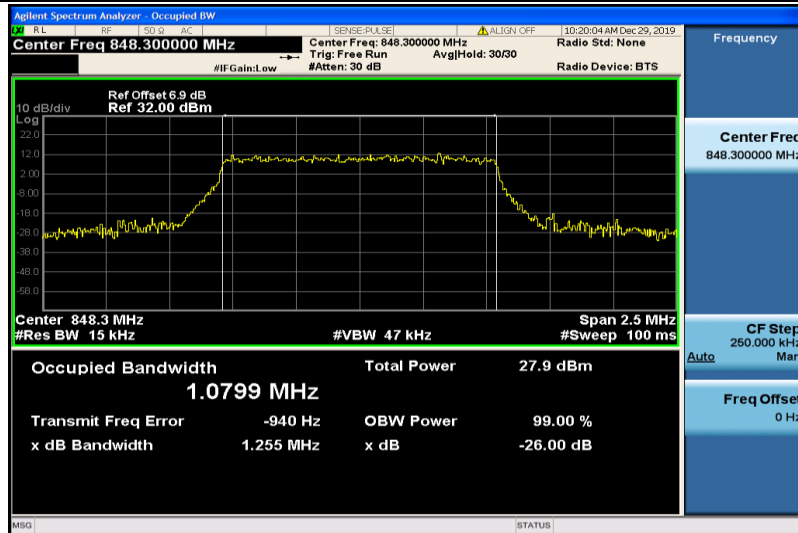
Band5-1.4MHz-16QAM-20643-6RB#0-1.0799
