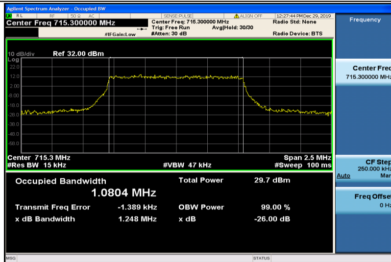
Band12-1.4MHz-QPSK-23173-6RB#0-1.0804
