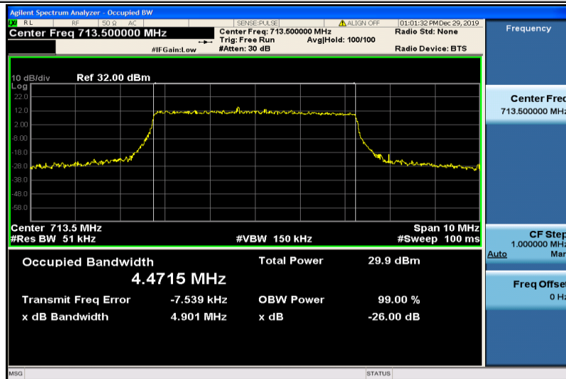
Band12-5MHz-16QAM-23155-25RB#0-4.4715
