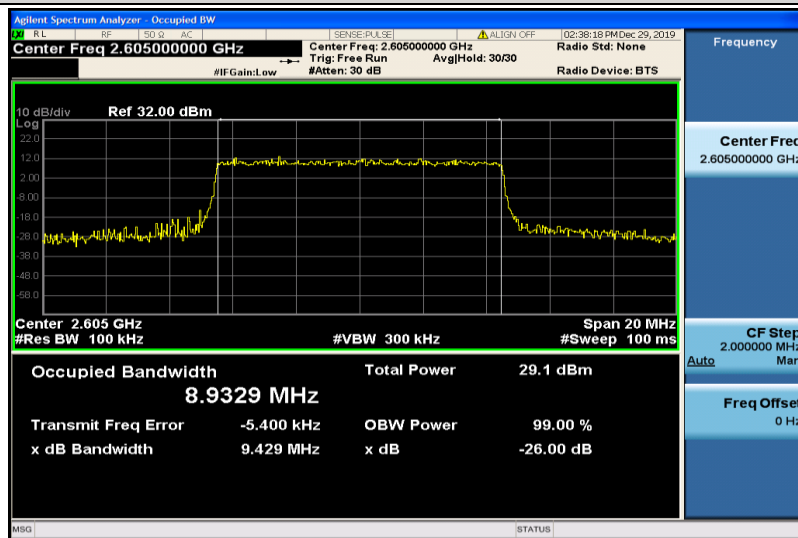
Band41-10MHz-16QAM-40740-50RB#0-8.9329
