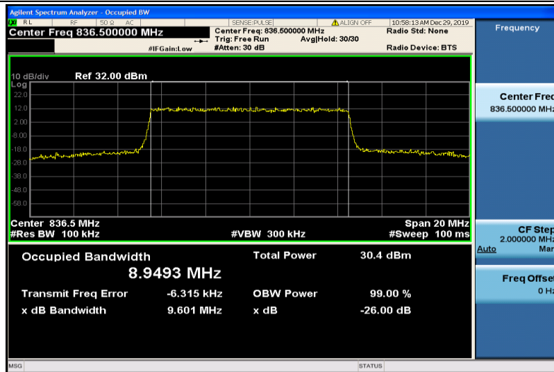
Band5-10MHz-QPSK-20525-50RB#0-8.9493
