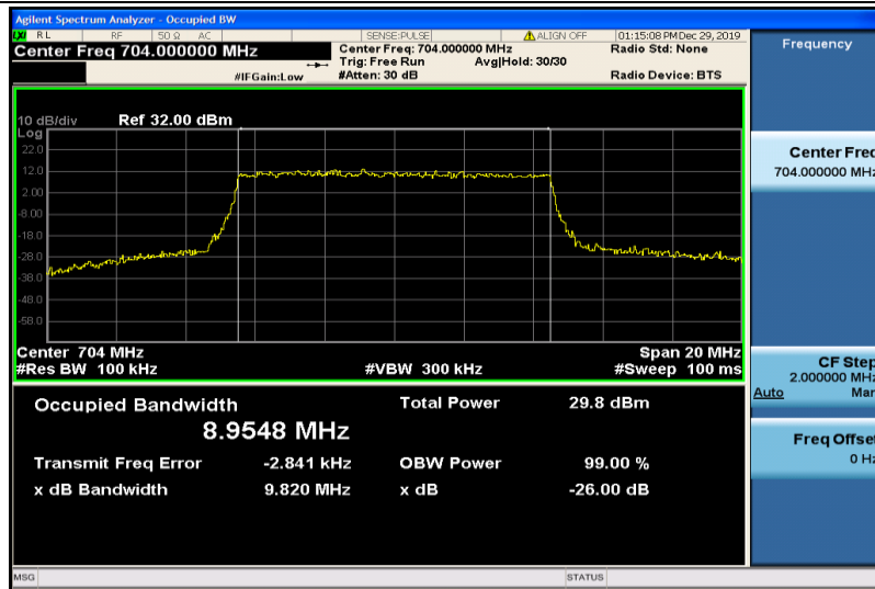
Band12-10MHz-16QAM-23060-50RB#0-8.9548
