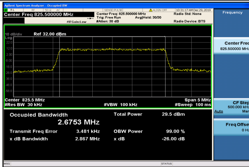
Band5-3MHz-QPSK-20415-15RB#0-2.6753
