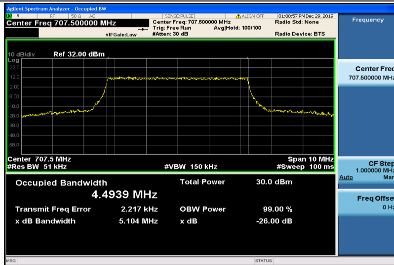
Band12-5MHz-16QAM-23095-25RB#0-4.4939
