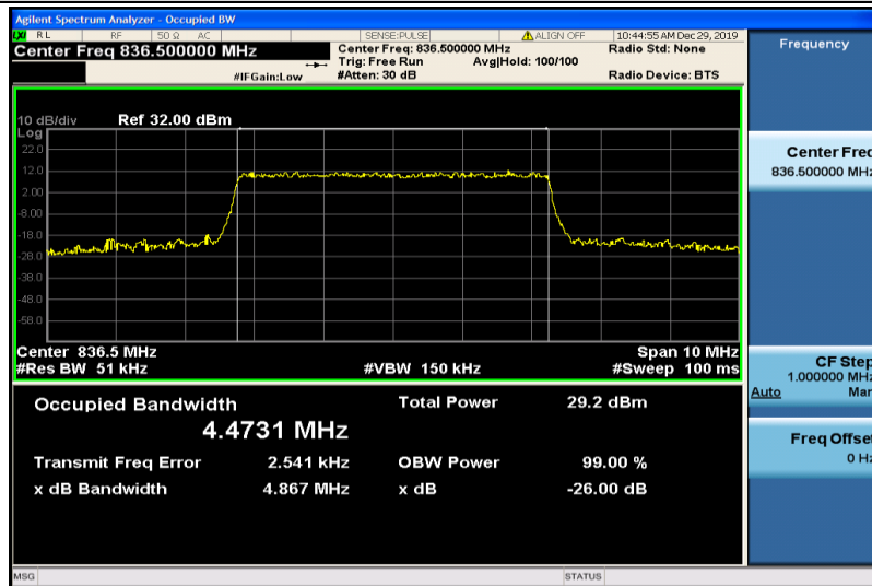
Band5-5MHz-16QAM-20525-25RB#0-4.4731
