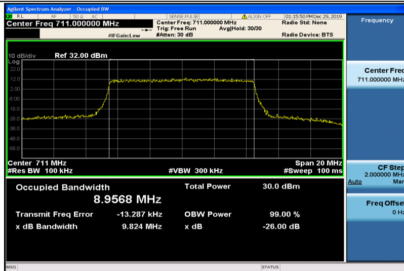
Band12-10MHz-16QAM-23130-50RB#0-8.9568
