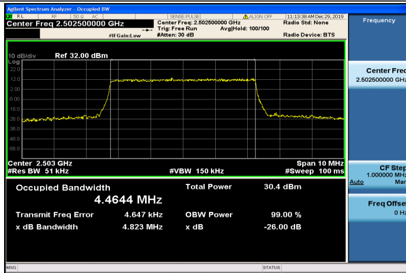
Band7-5MHz-QPSK-20775-25RB#0-4.4644
