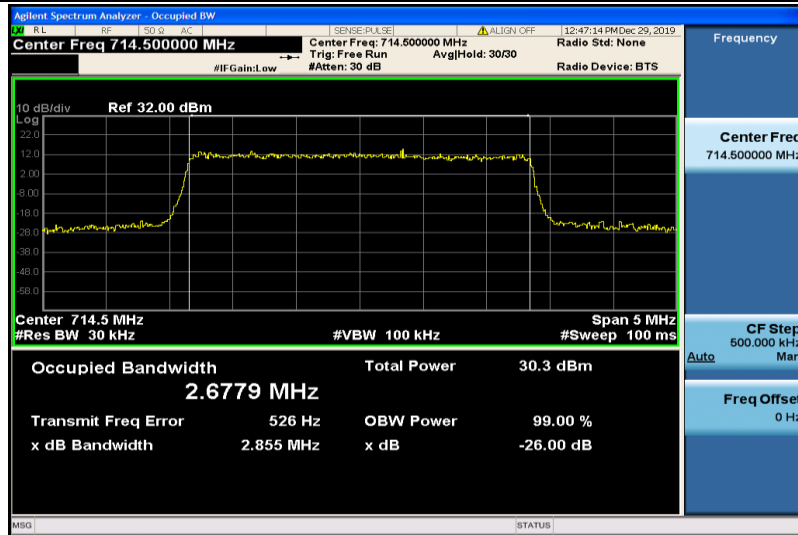
Band12-3MHz-QPSK-23165-15RB#0-2.6779
