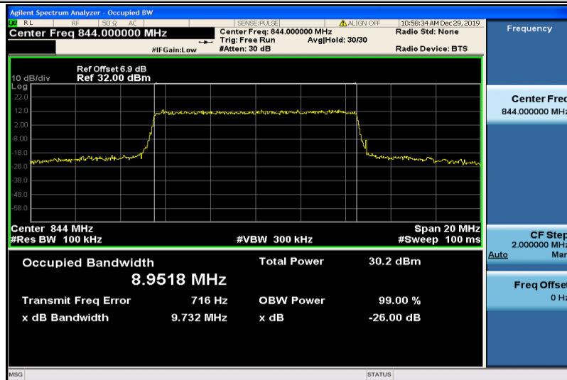
Band5-10MHz-QPSK-20600-50RB#0-8.9518
