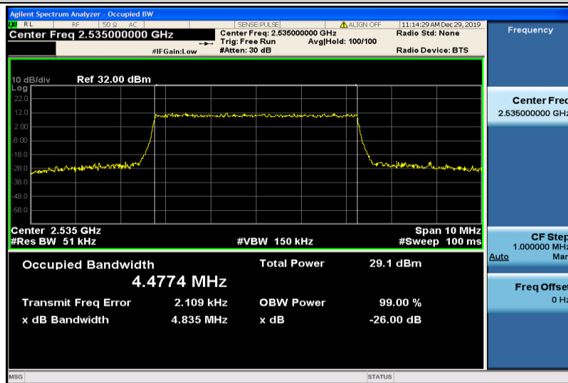
Band7-5MHz-16QAM-21100-25RB#0-4.4774
