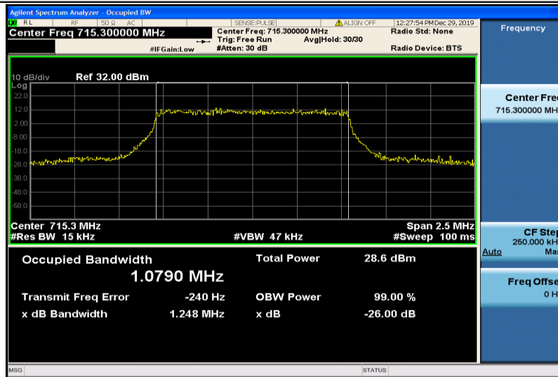
Band12-1.4MHz-16QAM-23173-6RB#0-1.0790
