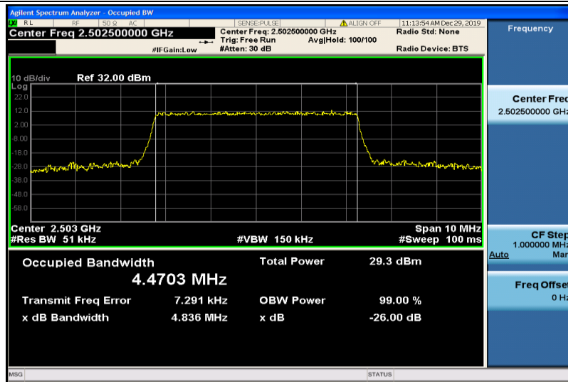
Band7-5MHz-16QAM-20775-25RB#0-4.4703
