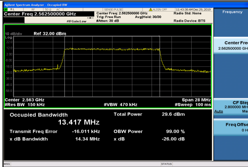
Band7-15MHz-16QAM-21375-75RB#0-13.417
