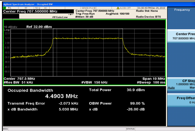
Band12-5MHz-QPSK-23095-25RB#0-4.4903
