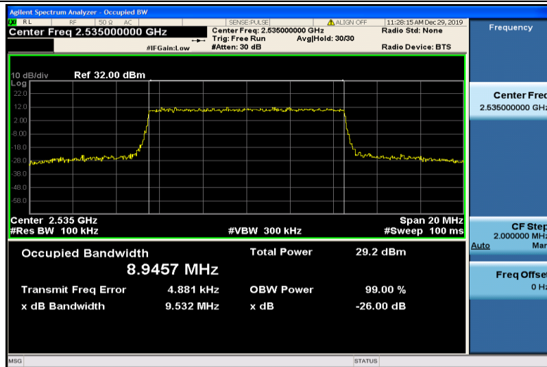
Band7-10MHz-16QAM-21100-50RB#0-8.9457
