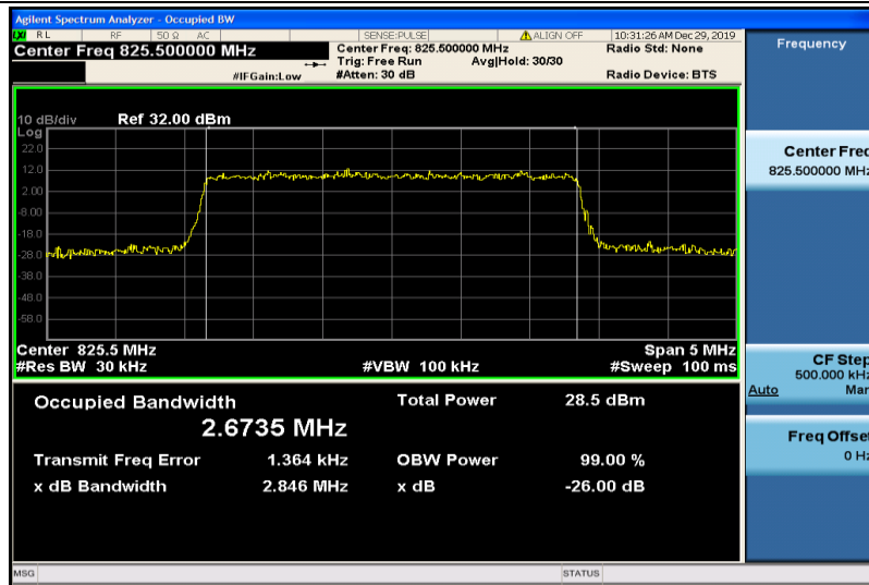
Band5-3MHz-16QAM-20415-15RB#0-2.6735
