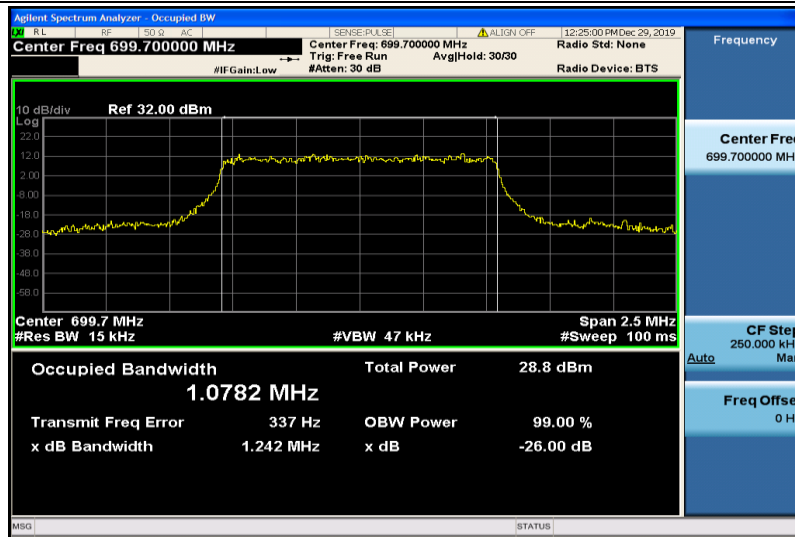
Band12-1.4MHz-16QAM-23017-6RB#0-1.0782
