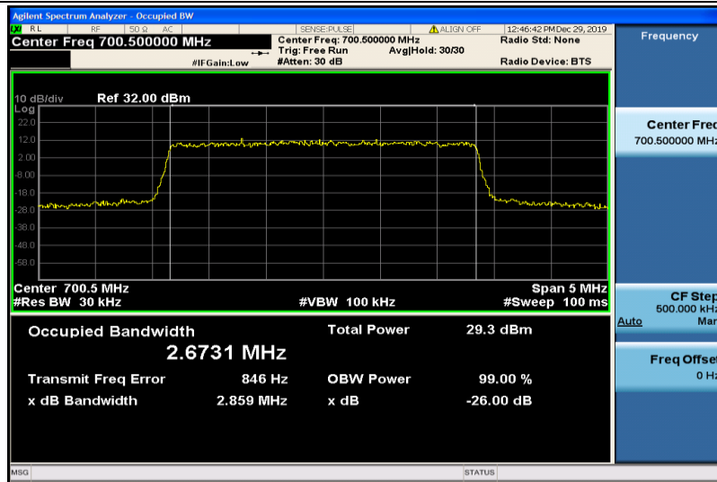
Band12-3MHz-16QAM-23025-15RB#0-2.6731
