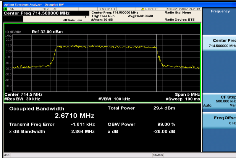
Band12-3MHz-16QAM-23165-15RB#0-2.6710
