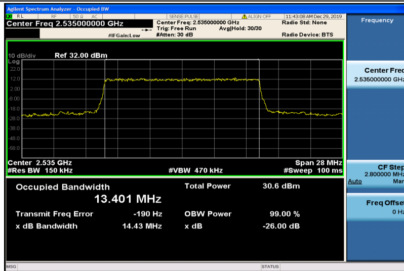
Band7-15MHz-QPSK-21100-75RB#0-13.401
