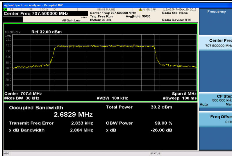
Band12-3MHz-QPSK-23095-15RB#0-2.6829
