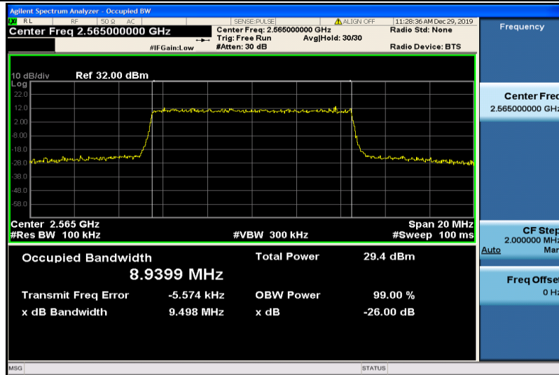
Band7-10MHz-16QAM-21400-50RB#0-8.9399
