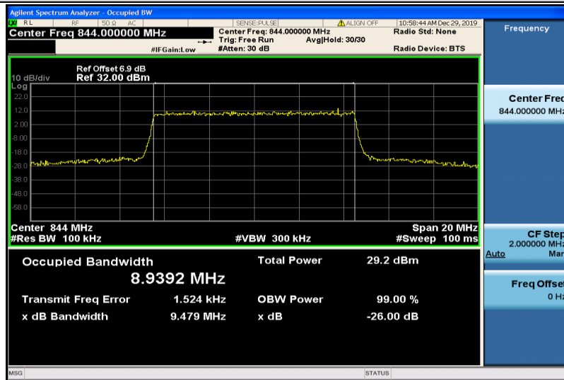
Band5-10MHz-16QAM-20600-50RB#0-8.9392
