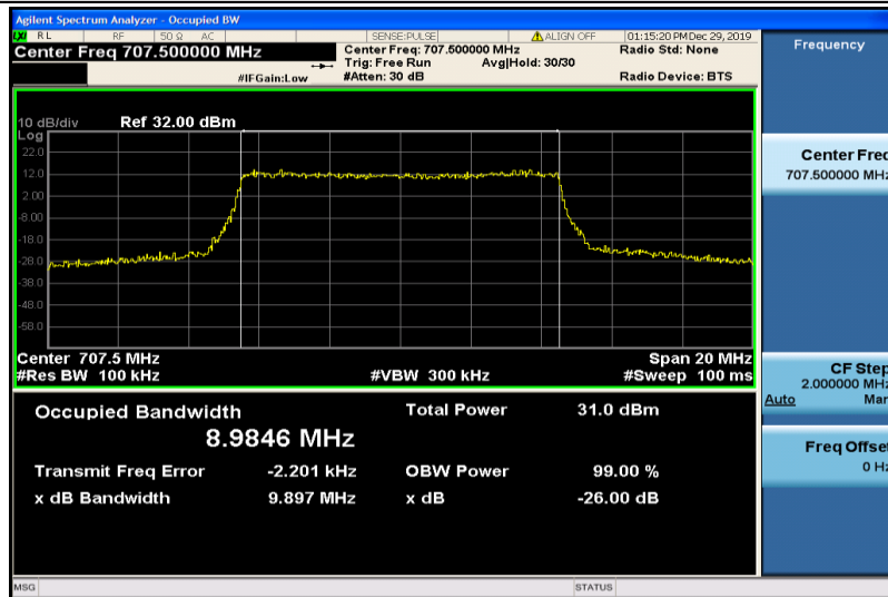
Band12-10MHz-QPSK-23095-50RB#0-8.9846
