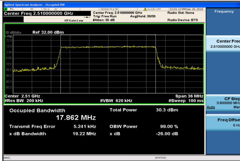
Band7-20MHz-QPSK-20850-100RB#0-17.862
