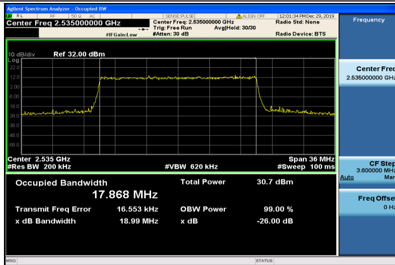
Band7-20MHz-QPSK-21100-100RB#0-17.868
