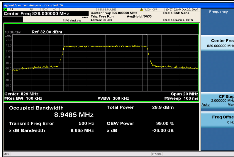
Band5-10MHz-QPSK-20450-50RB#0-8.9485
