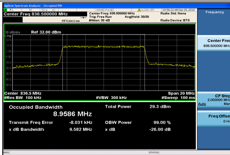
Band5-10MHz-16QAM-20525-50RB#0-8.9586
