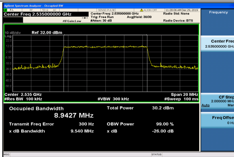
Band7-10MHz-QPSK-21100-50RB#0-8.9427
