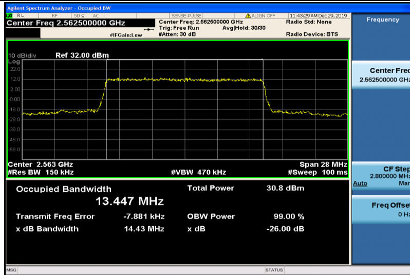
Band7-15MHz-QPSK-21375-75RB#0-13.447
