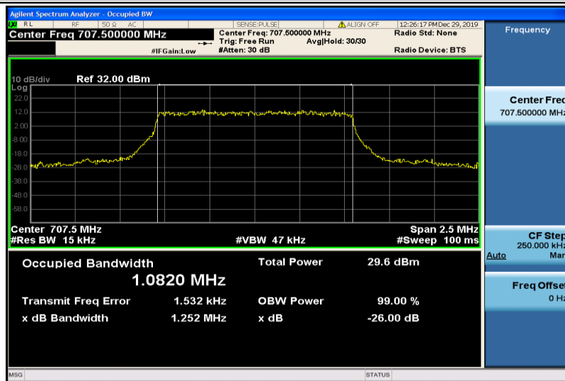
Band12-1.4MHz-QPSK-23095-6RB#0-1.0820
