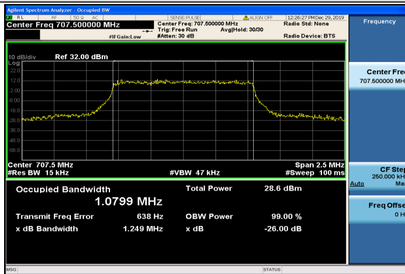
Band12-1.4MHz-16QAM-23095-6RB#0-1.0799
