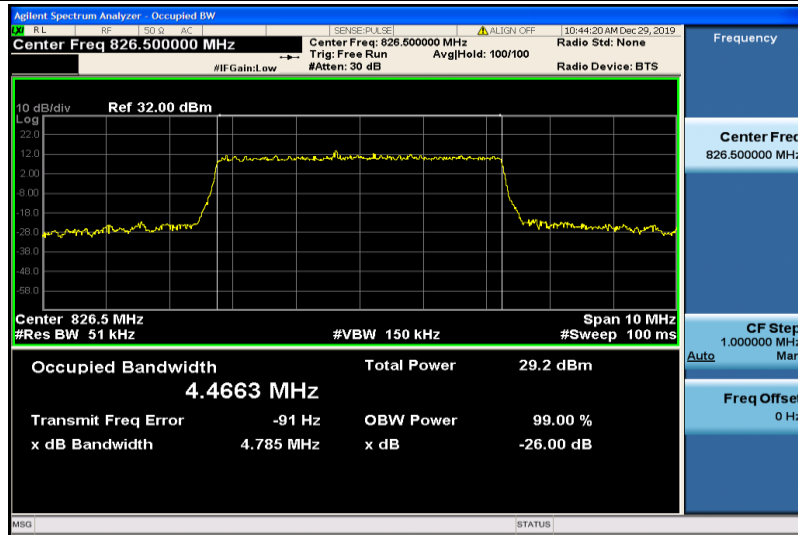
Band5-5MHz-16QAM-20425-25RB#0-4.4663
