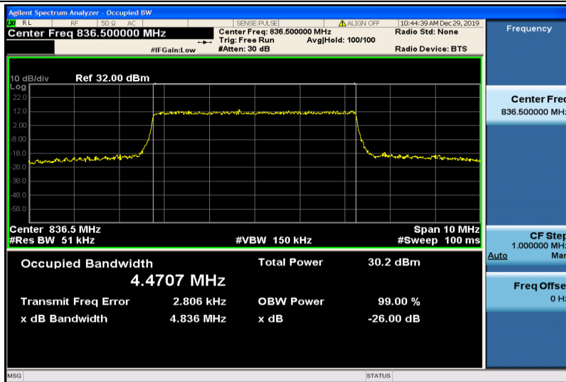
Band5-5MHz-QPSK-20525-25RB#0-4.4707
