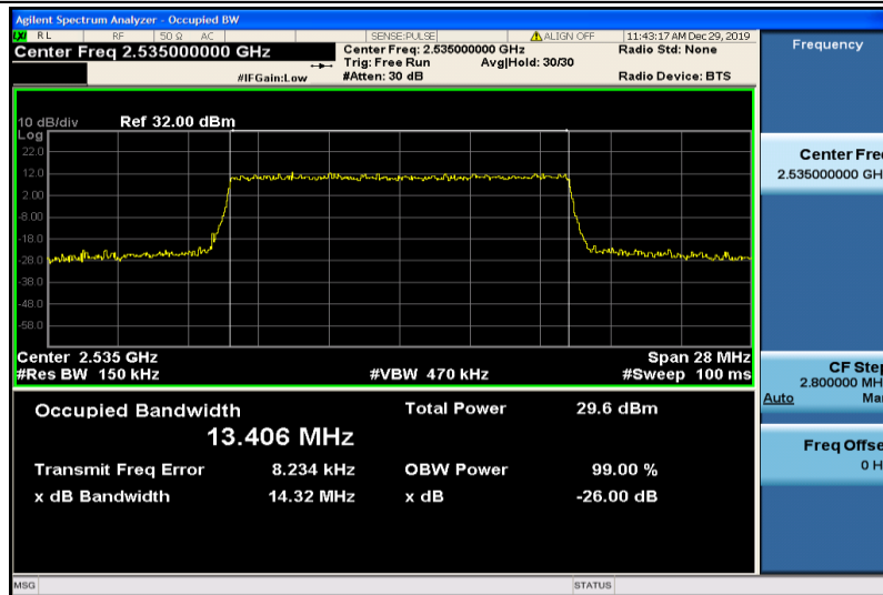
Band7-15MHz-16QAM-21100-75RB#0-13.406
