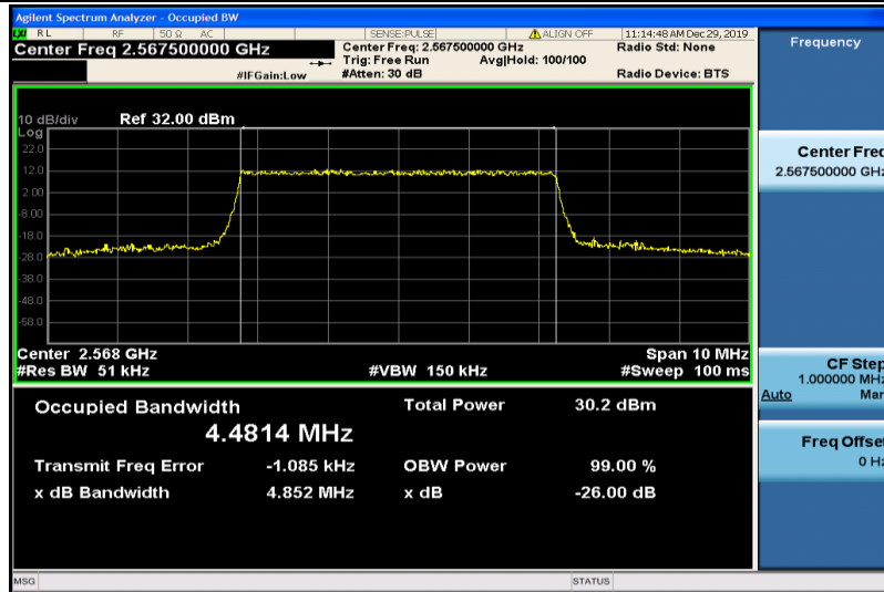
Band7-5MHz-QPSK-21425-25RB#0-4.4814
