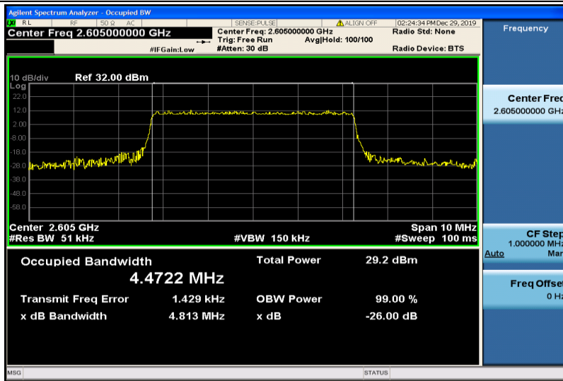
Band41-5MHz-16QAM-40740-25RB#0-4.4722
