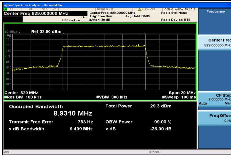
Band5-10MHz-16QAM-20450-50RB#0-8.9310
