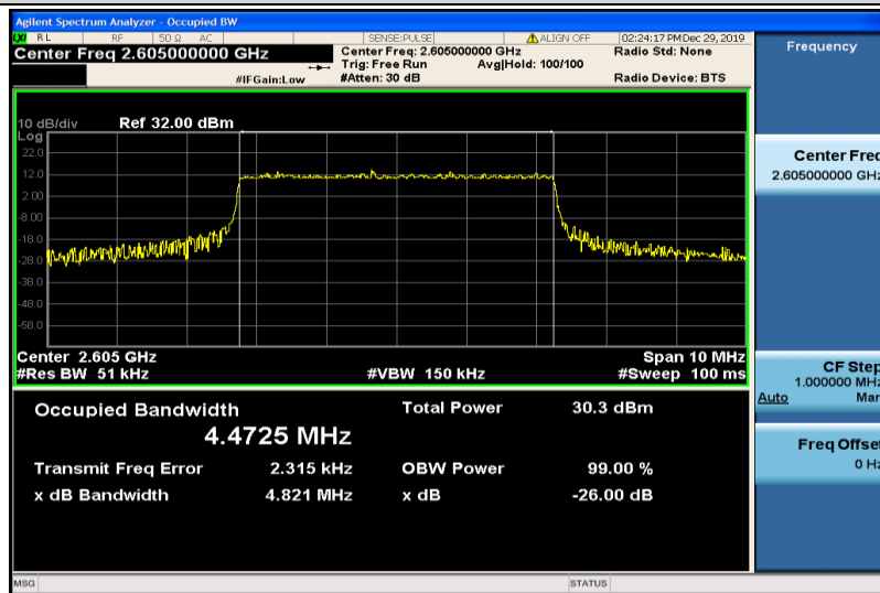
Band41-5MHz-QPSK-40740-25RB#0-4.4725
