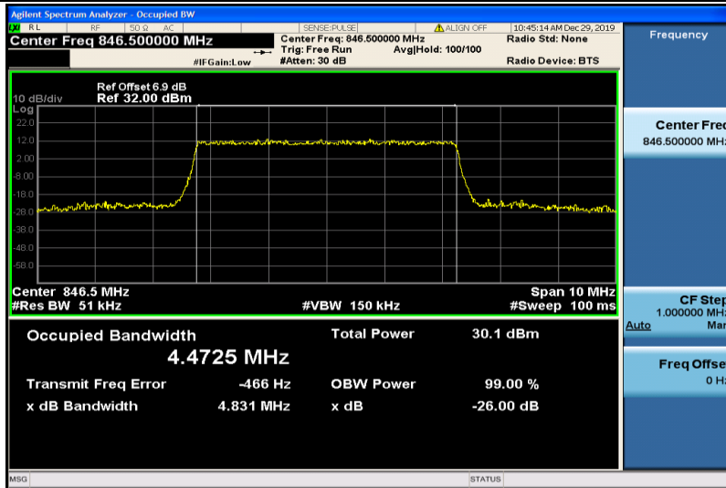
Band5-5MHz-QPSK-20625-25RB#0-4.4725
