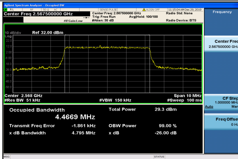
Band7-5MHz-16QAM-21425-25RB#0-4.4669
