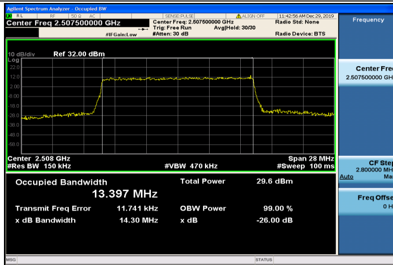
Band7-15MHz-16QAM-20825-75RB#0-13.397
