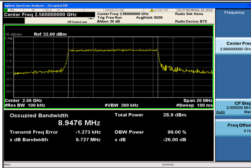
Band41-10MHz-16QAM-40290-50RB#0-8.9476
