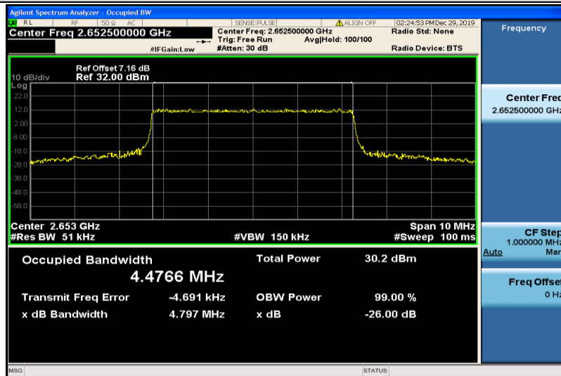
Band41-5MHz-QPSK-41215-25RB#0-4.4766
