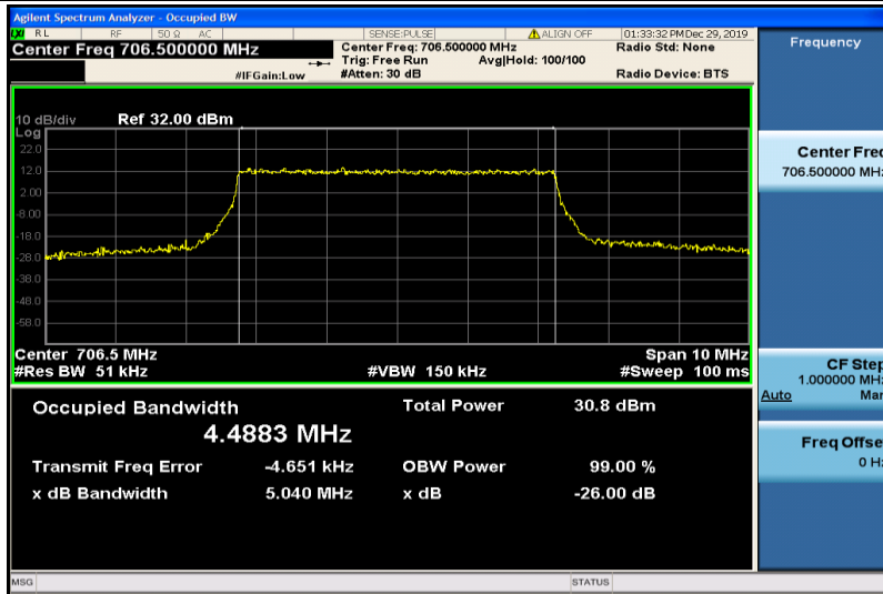
Band17-5MHz-QPSK-23755-25RB#0-4.4883
