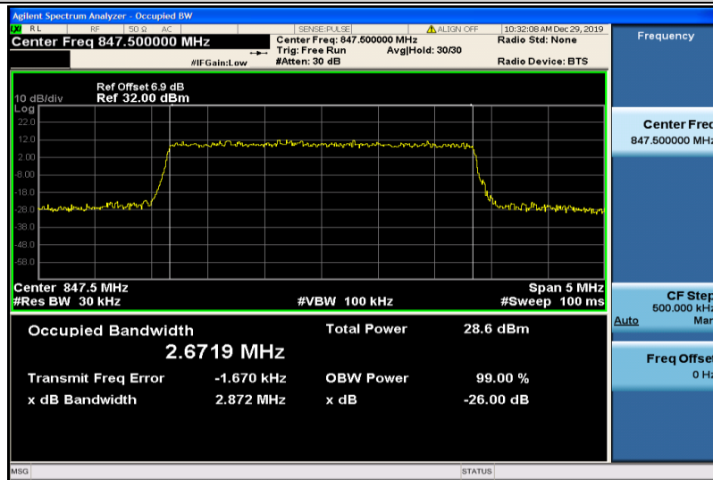
Band5-3MHz-16QAM-20635-15RB#0-2.6719
