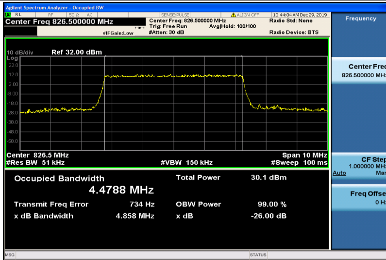
Band5-5MHz-QPSK-20425-25RB#0-4.4788
