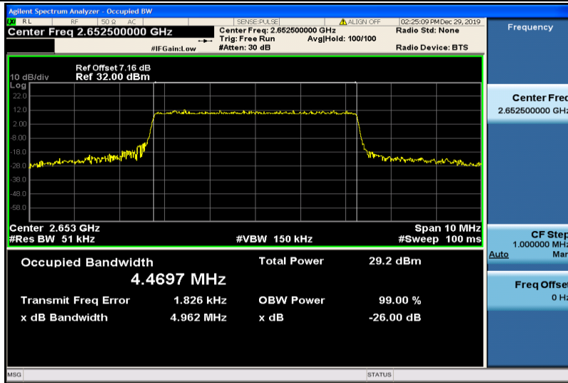
Band41-5MHz-16QAM-41215-25RB#0-4.4697
