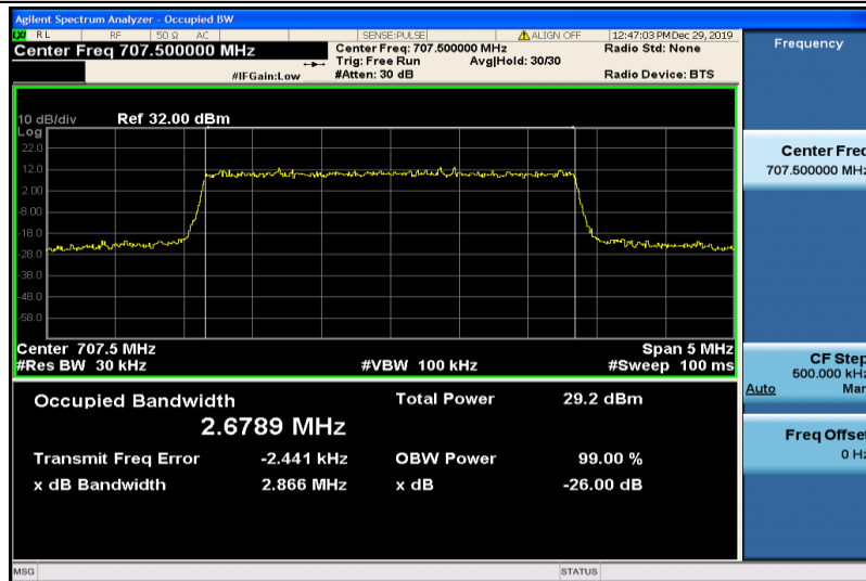
Band12-3MHz-16QAM-23095-15RB#0-2.6789
