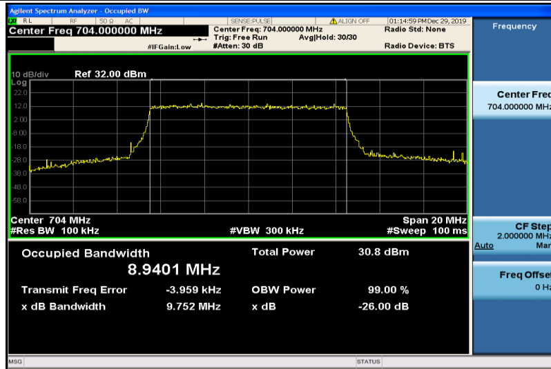
Band12-10MHz-QPSK-23060-50RB#0-8.9401
