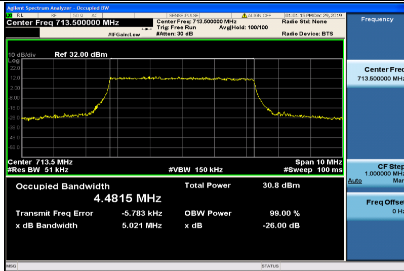
Band12-5MHz-QPSK-23155-25RB#0-4.4815
