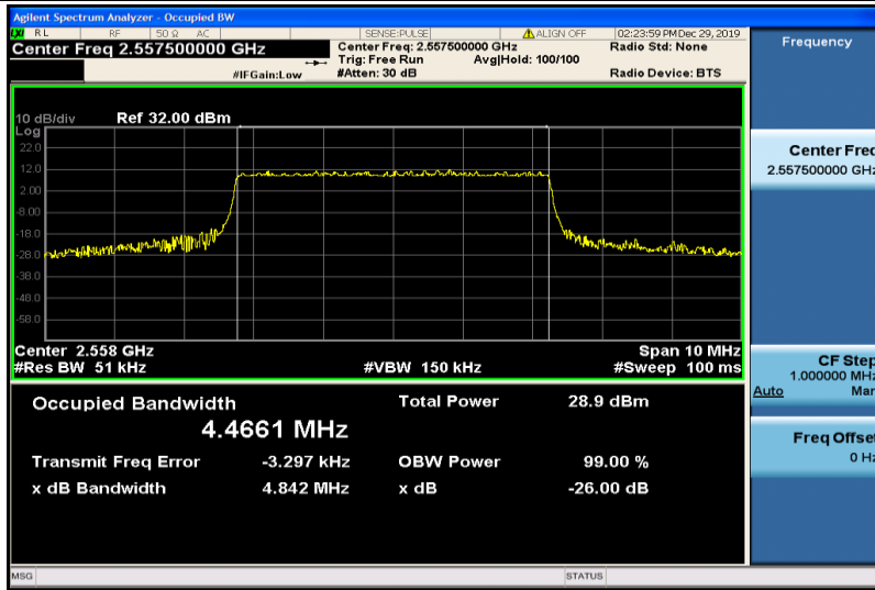
Band41-5MHz-16QAM-40265-25RB#0-4.4661
