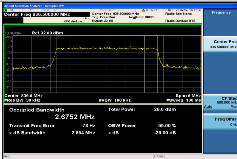
Band5-3MHz-16QAM-20525-15RB#0-2.6752
