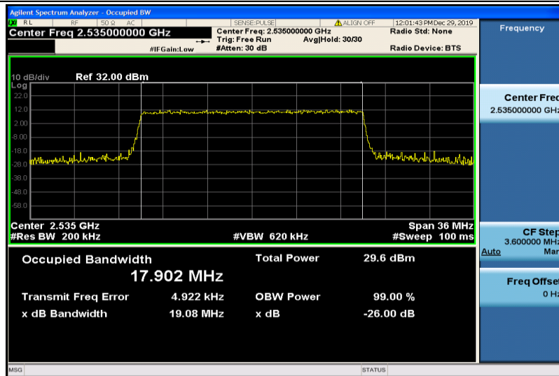
Band7-20MHz-16QAM-21100-100RB#0-17.902
