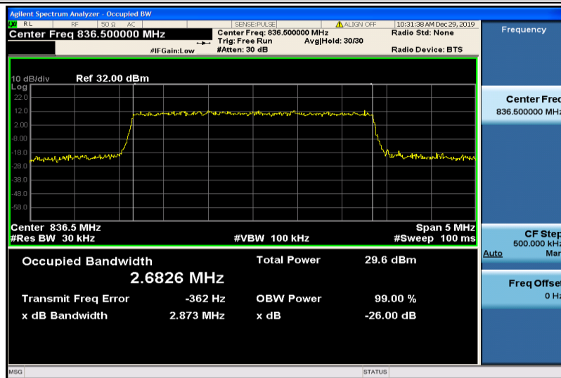
Band5-3MHz-QPSK-20525-15RB#0-2.6826
