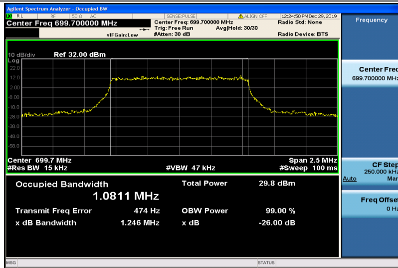
Band12-1.4MHz-QPSK-23017-6RB#0-1.0811
