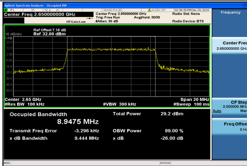
Band41-10MHz-16QAM-41190-50RB#0-8.9475
