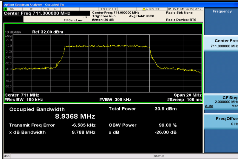
Band12-10MHz-QPSK-23130-50RB#0-8.9368
