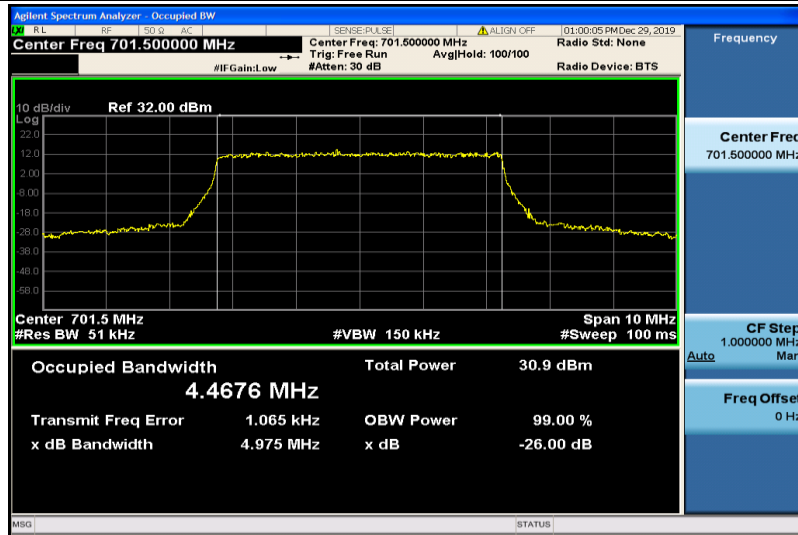
Band12-5MHz-QPSK-23035-25RB#0-4.4676
