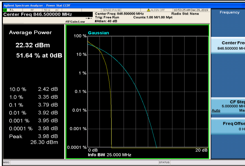
Band5-5MHz-QPSK-20625-1RB#0
