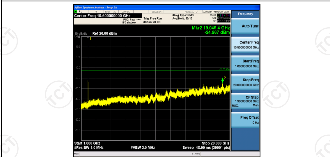
Band2-15MHz-16QAM-18900-1RB#0-Range2:1000~20000MHz
