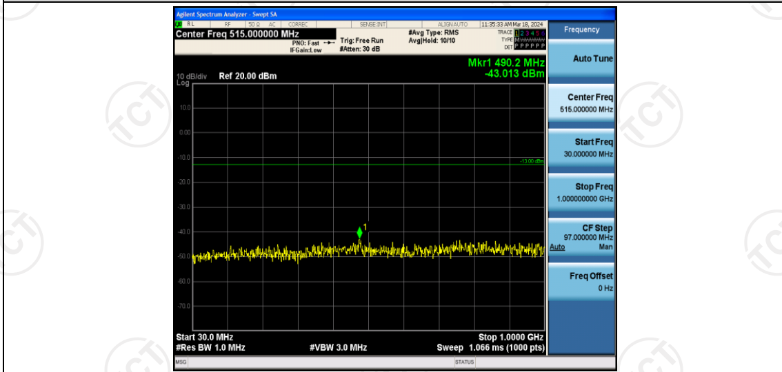
Band2-3MHz-QPSK-18900-1RB#0-Range1:30~1000MHz
