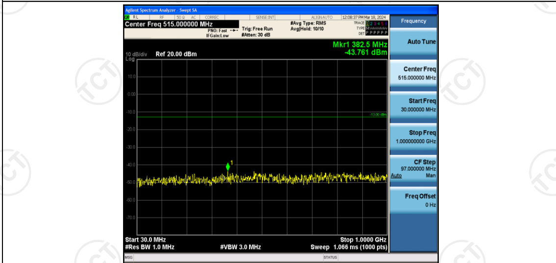
Band2-15MHz-16QAM-18900-1RB#0-Range1:30~1000MHz
