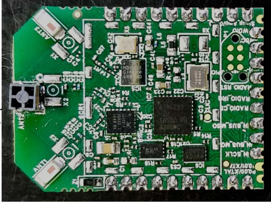
Internal, top without shield
