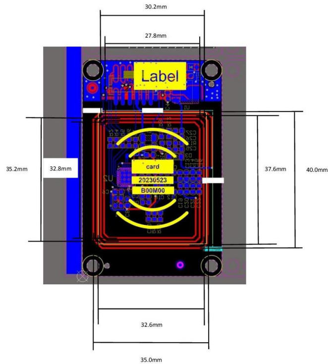
Antenna dimension design
