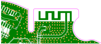
Antenna Location
