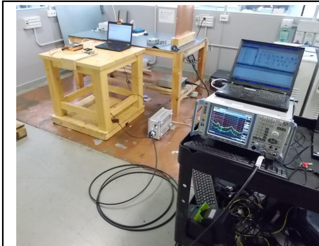
Set-up conducted emission test on ACPort
