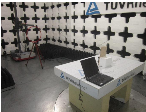
Set-up radiated emission test
