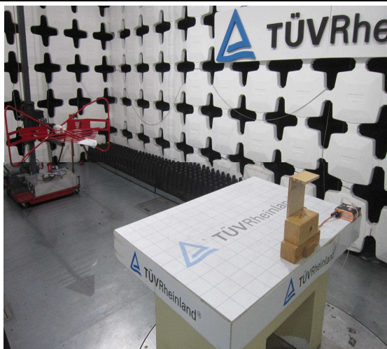
Set-up radiated emission test
