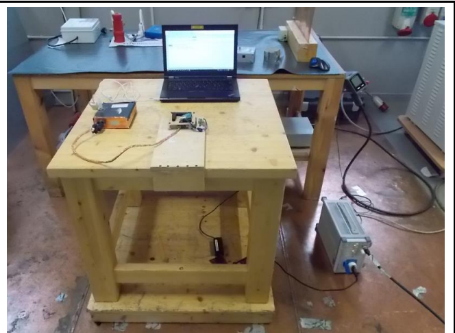
Set-up conducted emission test on ACPort
