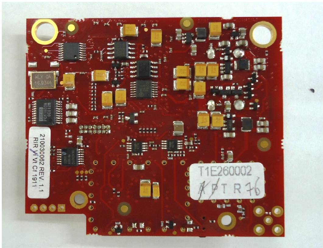
MOVING D Body-pack PCB - (bottom)
