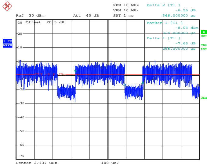
Figure 7.7.2-2: Duty Cycle 802.11g
