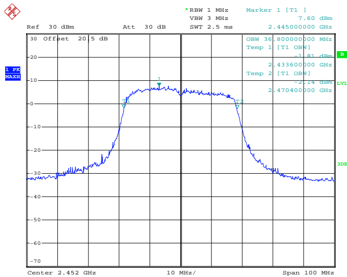
Figure 7.2.2-23: 99% OBW - Middle Channel – 802.11n 40 MHz
