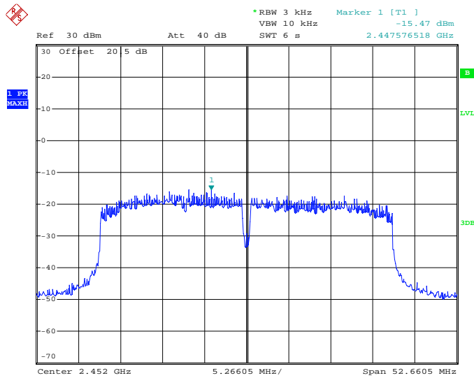
Figure 7.5.2-11: Power Spectral Density - Middle Channel – 802.11n 40 MHz
