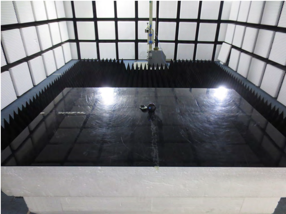
WLAN_Horn Ant_18~25GHz
