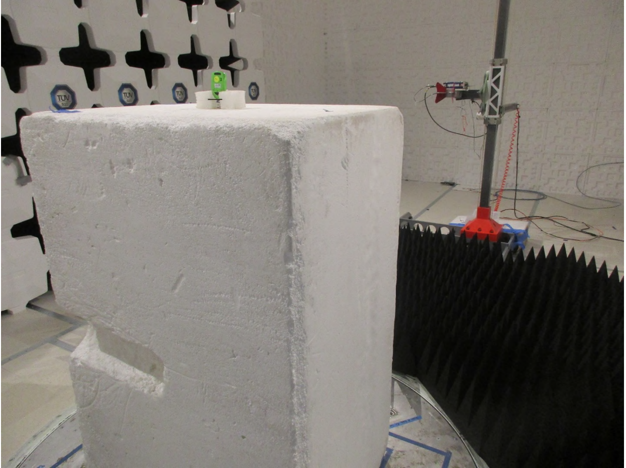
Figure 5: Radiated Emissions – Back View – above 1 GHz – EUT Standing
