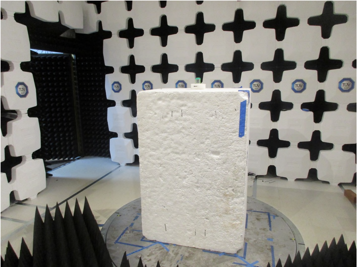
Figure 4: Radiated Emissions – Front View – above 1 GHz – EUT Standing
