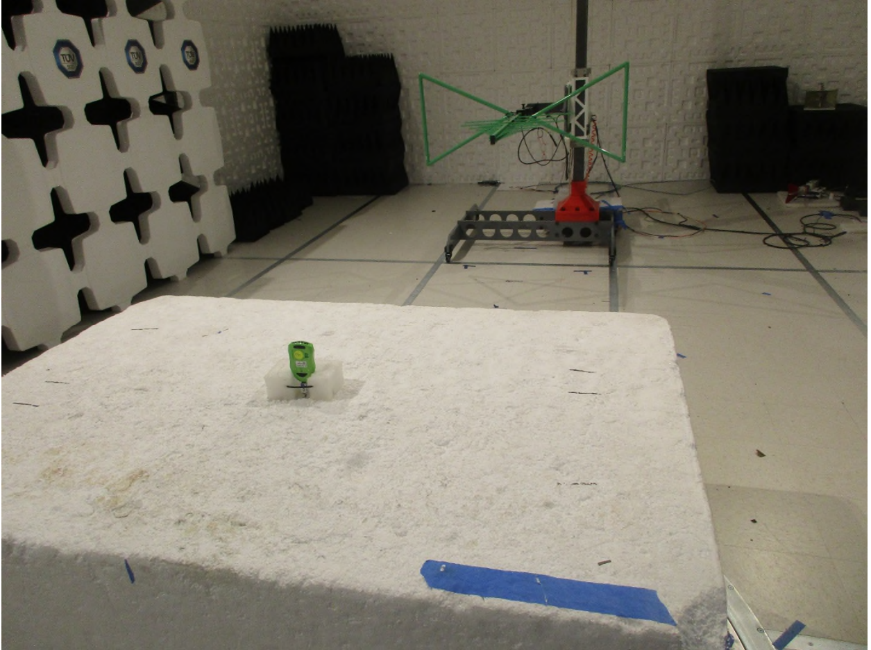
Figure 3: Radiated Emissions – Back View – 30 MHz – 1 GHz – EUT Standing
