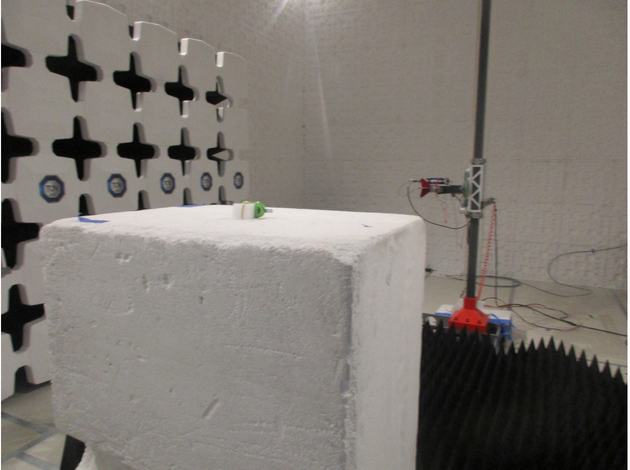
Figure 7: Radiated Emissions – Back View – above 1 GHz – EUT on Side (Band-Edge Measurements)
