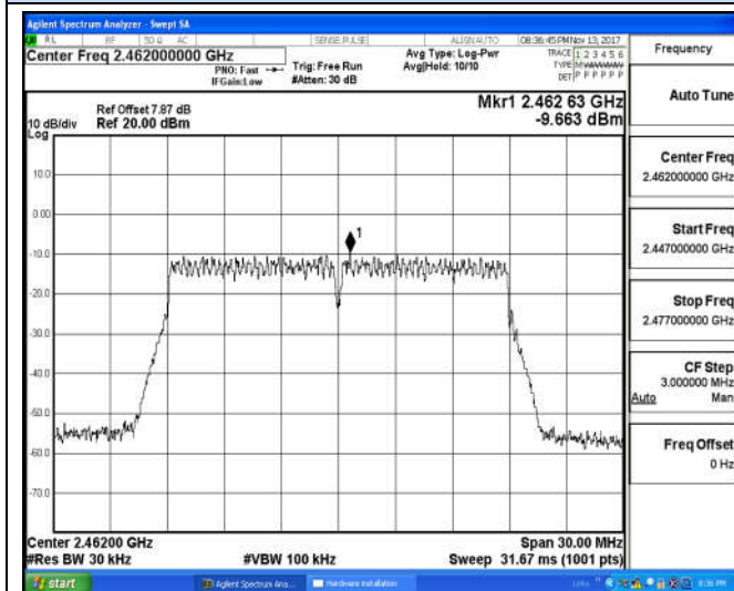
Channel 11 / 2462 MHz
