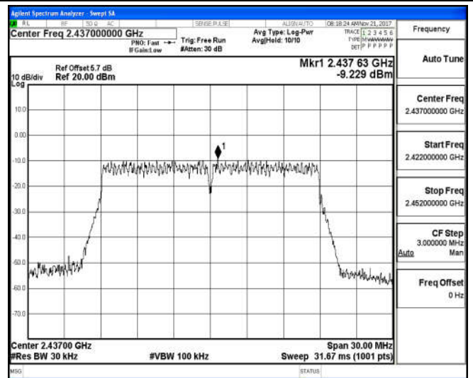
Channel 6 / 2437 MHz
