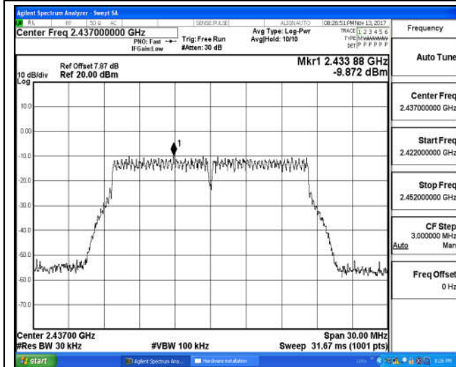
Channel 6 / 2437 MHz
