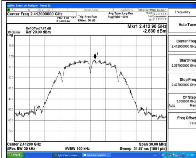
Channel 1 / 2412 MHz
