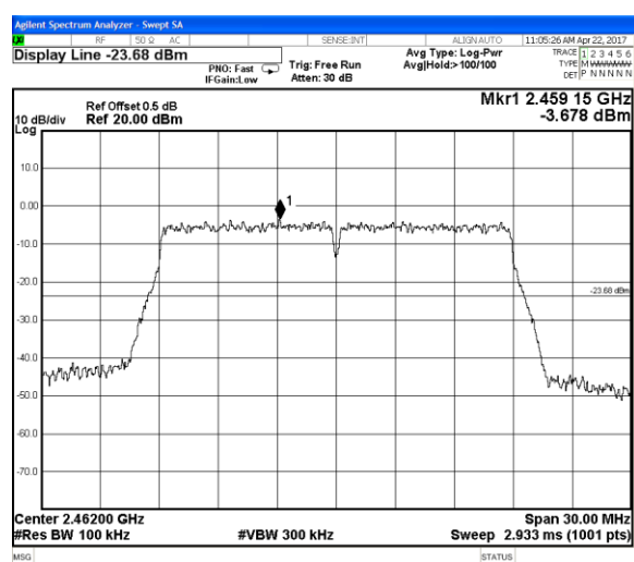
Chain 1-Channel 11 / 2462 MHz
