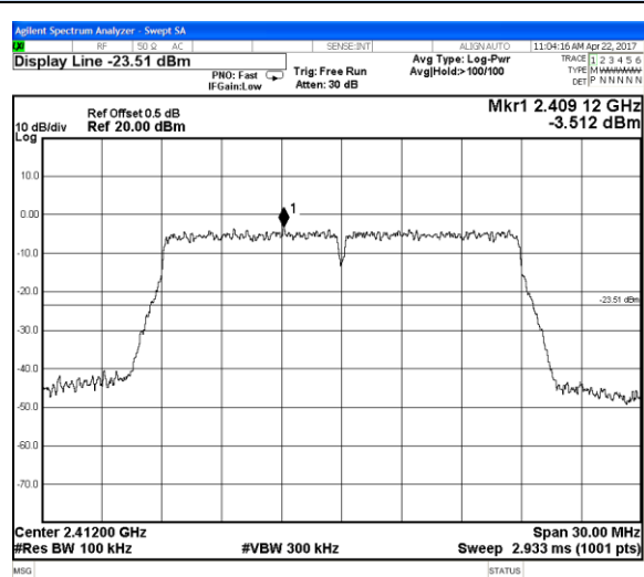
Chain 1-Channel 1 / 2412 MHz
