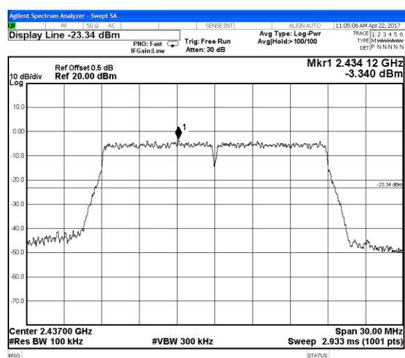
Chain 1-Channel 6 / 2437 MHz
