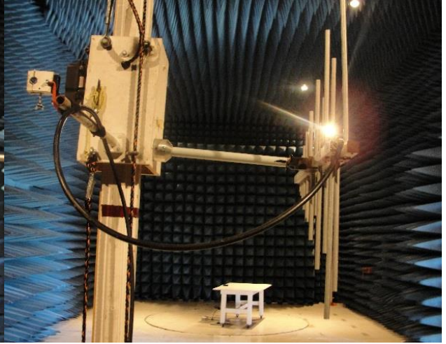
FIGURE 7:RE Test Setup-Log Periodic Vertical
