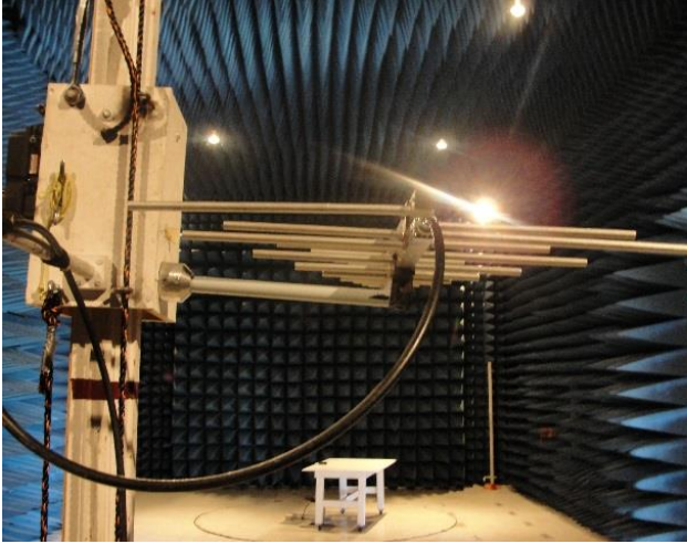
FIGURE 6:RE Test Setup- Log Periodic Horizontal
