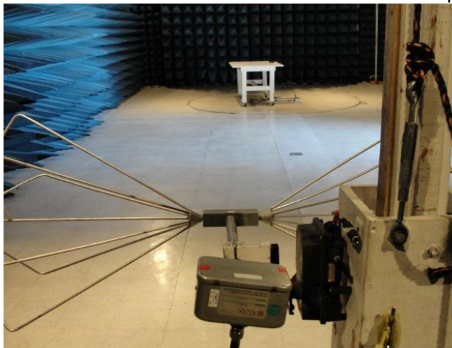
FIGURE 4: RE Test Setup – Biconical Horizontal Vertical
