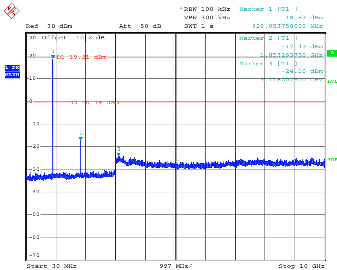
Figure 7.4.2-2: 30 MHz – 10 GHz – Middle Channel
