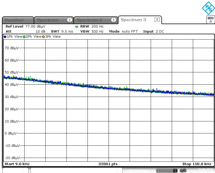
Figure A-1: 9kHz-150kHz1GHz – Radiated Emissions
