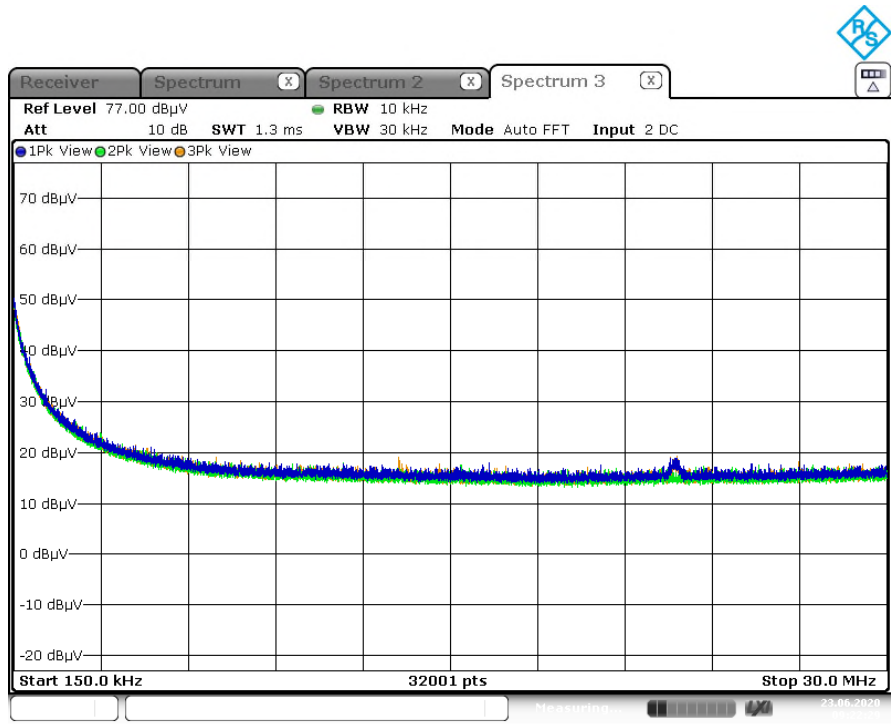
Figure A-2: 150kHz-30MHz1GHz – Radiated Emissions
