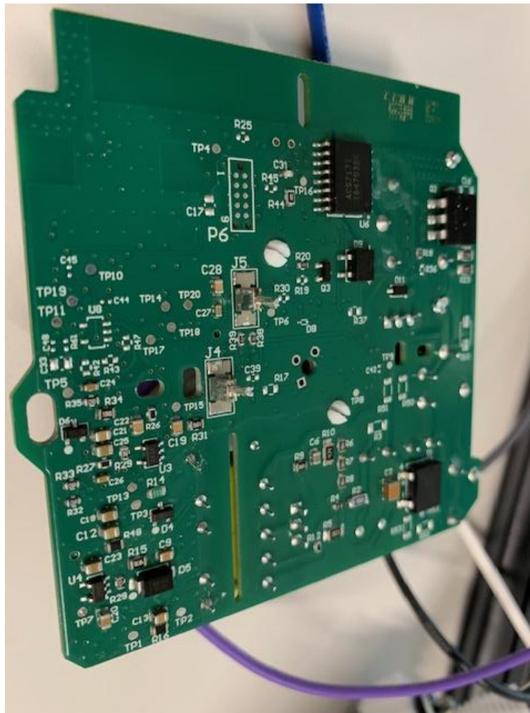
PCBA (Bottom)
