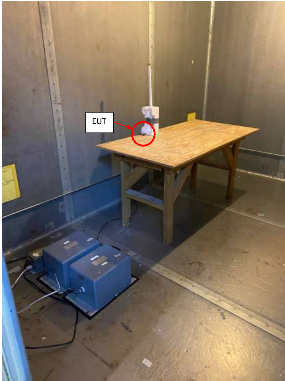
Figure 3. Power Lines Conducted Emissions Test Configuration
