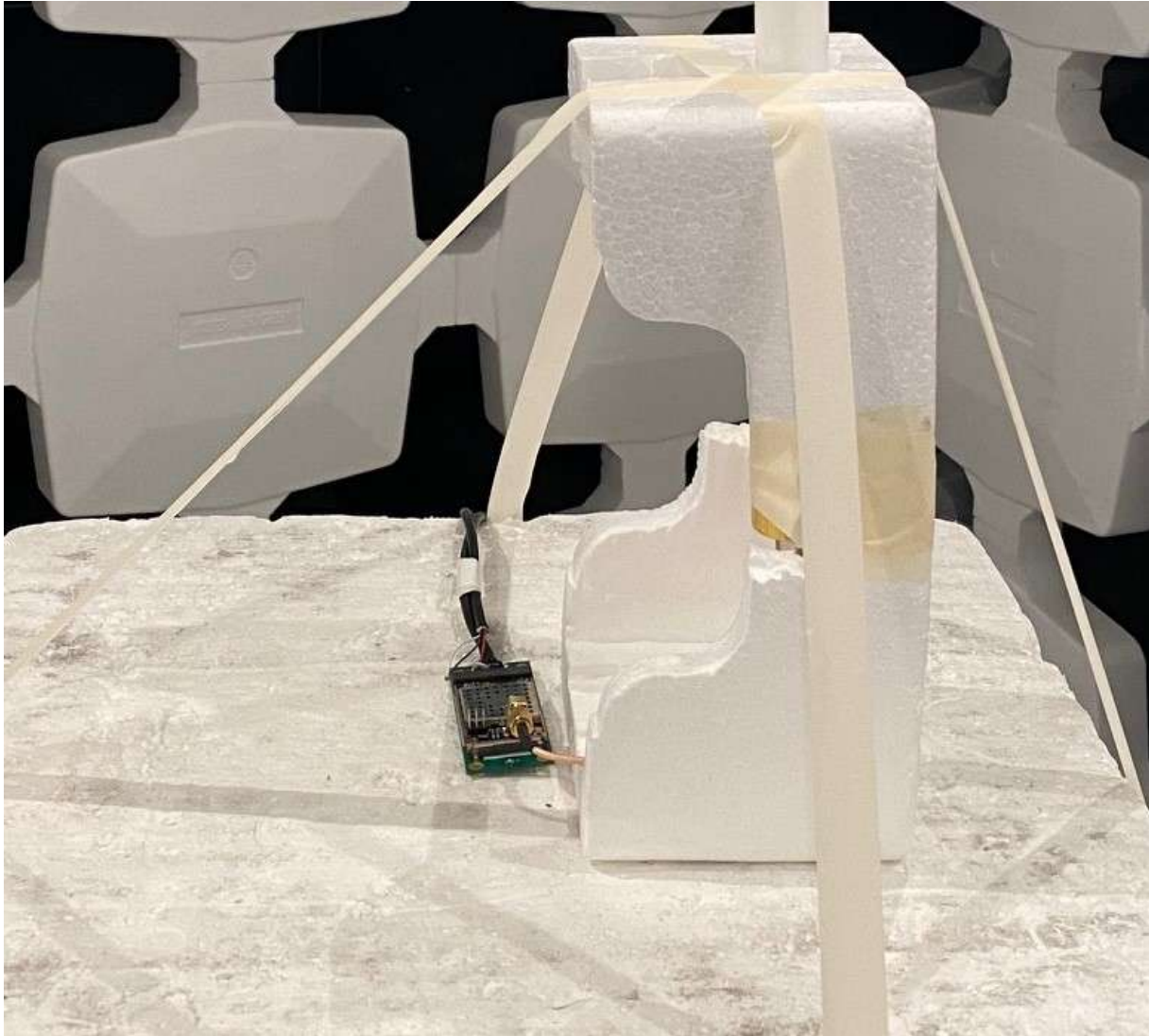
Figure 3. Close-up of EUT Test Setup on Foam Block
