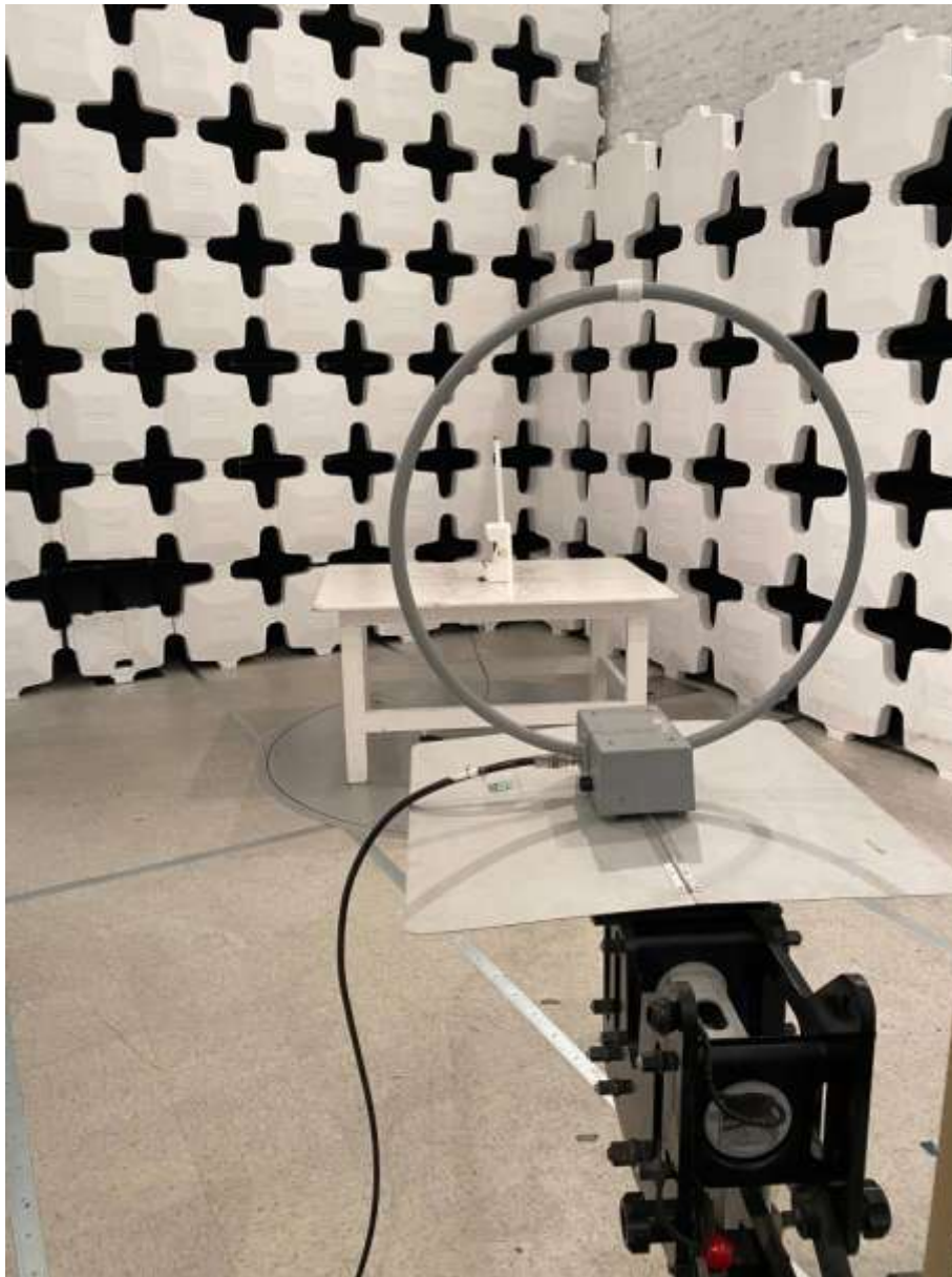
Figure 4. Radiated Emissions Test Configuration (9 kHz – 30 MHz)
