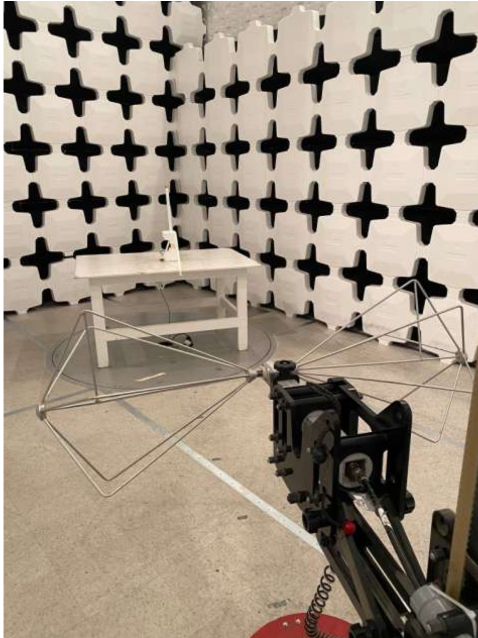
Figure 5. Radiated Emissions Test Configuration (30 MHz – 200 MHz)
