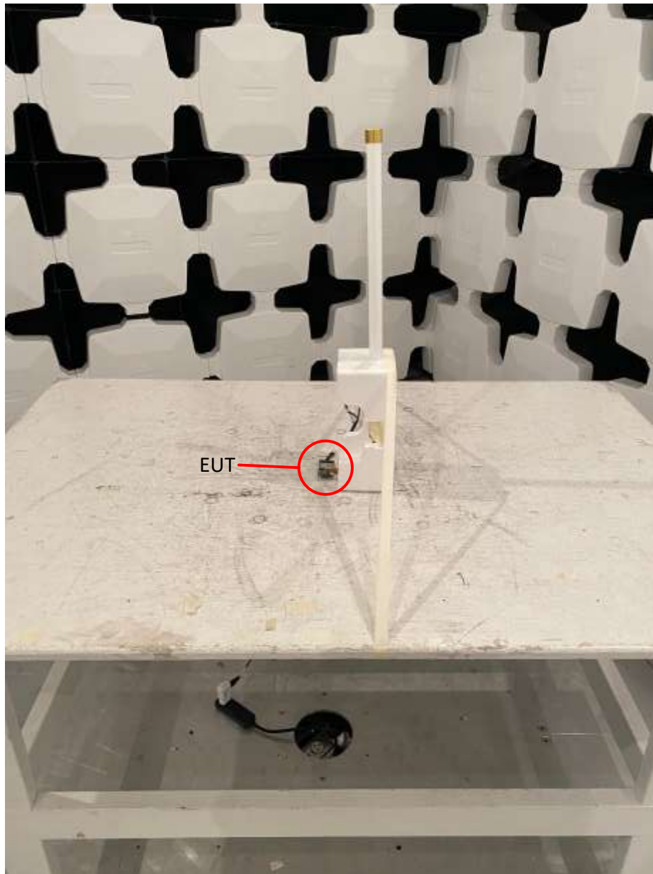
Figure 1. Radiated Emissions EUT Test Setup (Below 1000 MHz)
