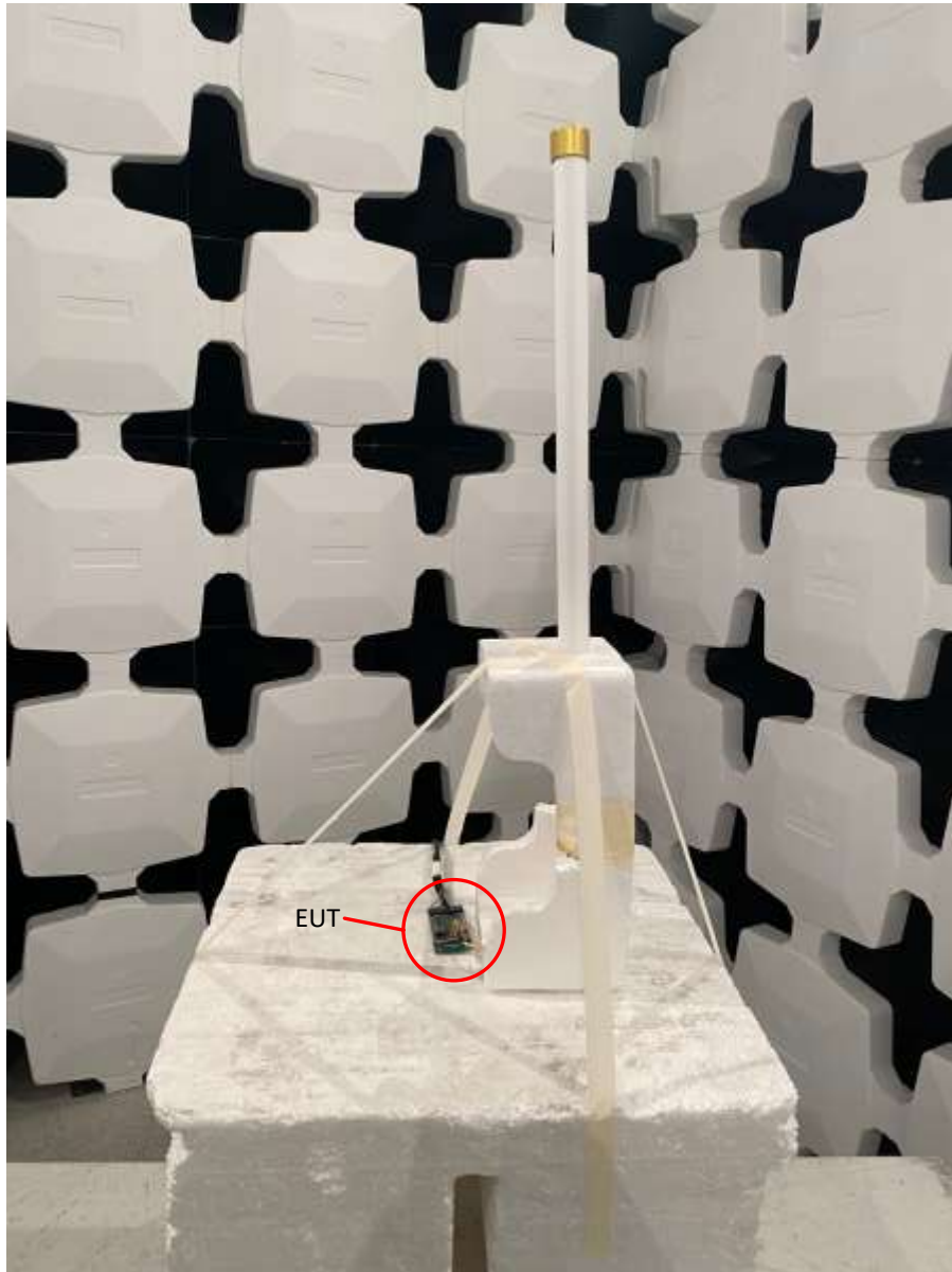
Figure 2. Radiated Emissions EUT Test Setup (Above 1000 MHz)
