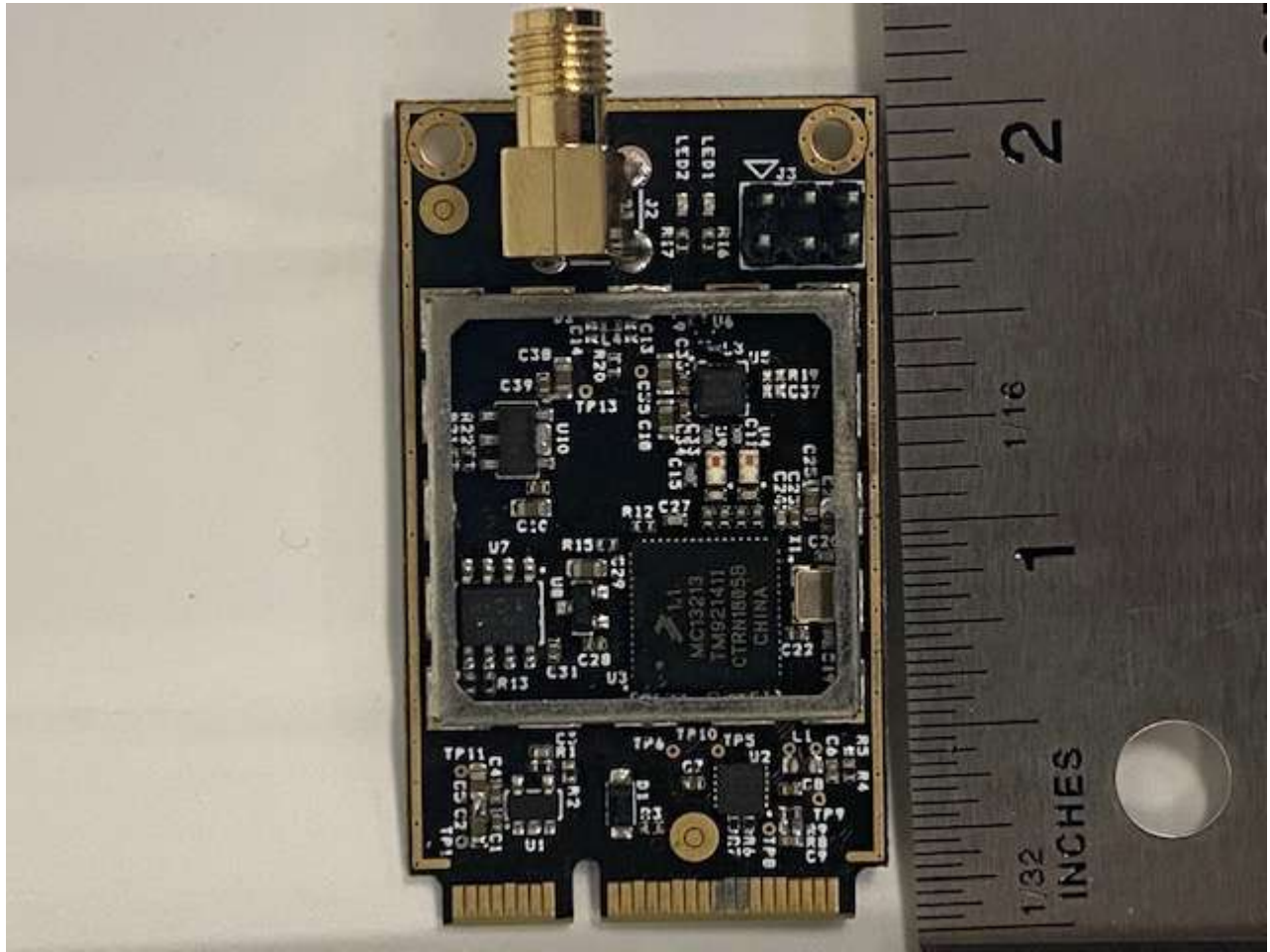
Figure 1. Radio Module with Shield Removed
