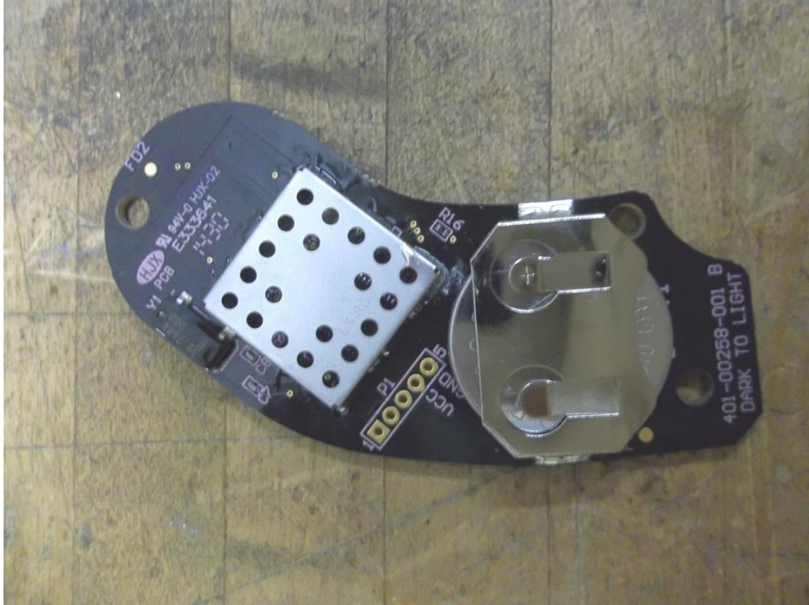
Figure 3. Back of EUT with External Cases Removed
