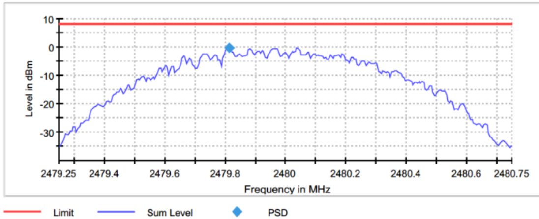
Figure 2.5.6-3: PSD – HCH
