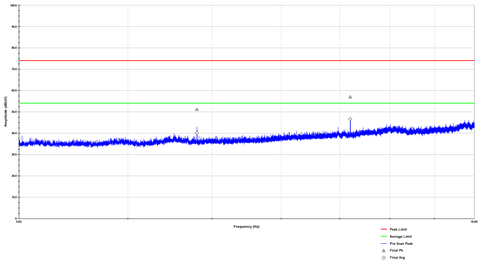
Figure 2.8.6-10: Reference plot for Radiated Spurious Emissions – 3 GHz – 10 GHz – V Polarity
