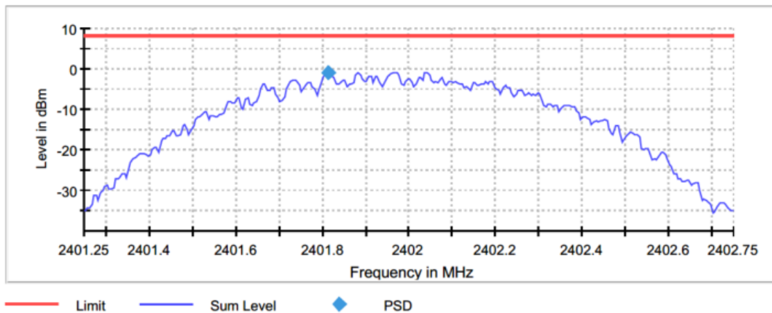
Figure 2.5.6-1: PSD – LCH
