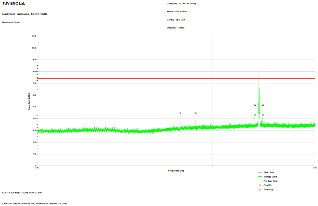
Figure 2.8.6-7: Reference plot for Radiated Spurious Emissions – 1 GHz – 3 GHz – H Polarity
