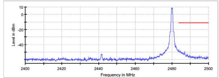
Figure 2.6.6-2: Upper Band-edge
