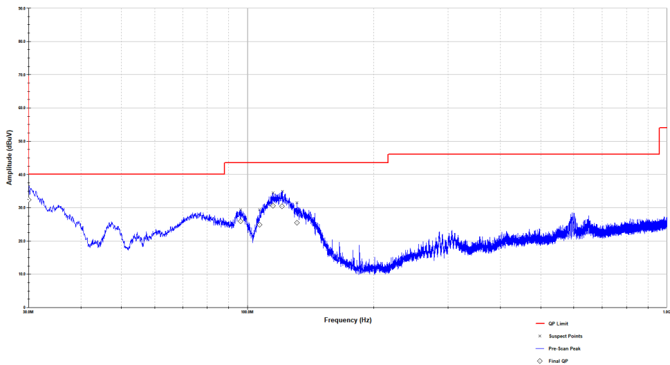
Figure 2.8.6-6: Reference plot for Radiated Spurious Emissions – 30 MHz – 1 GHz – V Polarity
