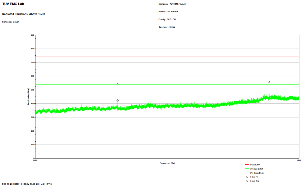
Figure 2.8.6-11: Reference plot for Radiated Spurious Emissions – 10 GHz – 18 GHz – H Polarity
