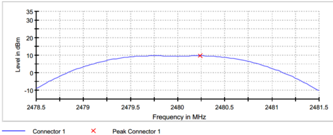
Figure 2.3.6-3: Output Power - HCH
