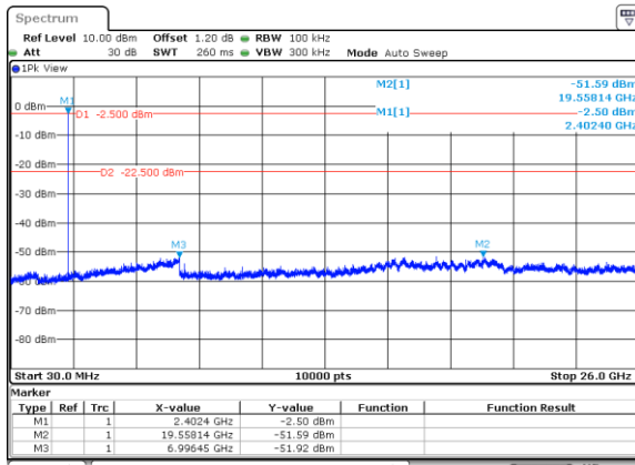
Figure 2.7.6-1: 30MHz – 26GHz – LCH
