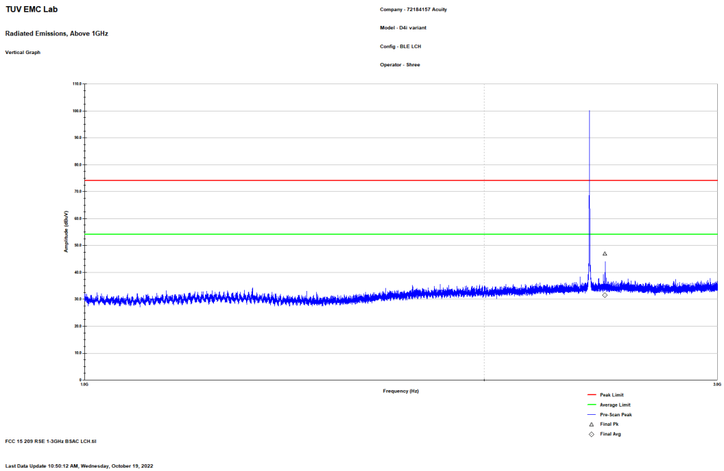
Figure 2.8.6-8: Reference plot for Radiated Spurious Emissions – 1 GHz – 3 GHz – V Polarity
