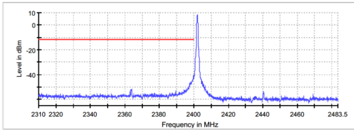
Figure 2.6.6-1: Lower Band-edge
