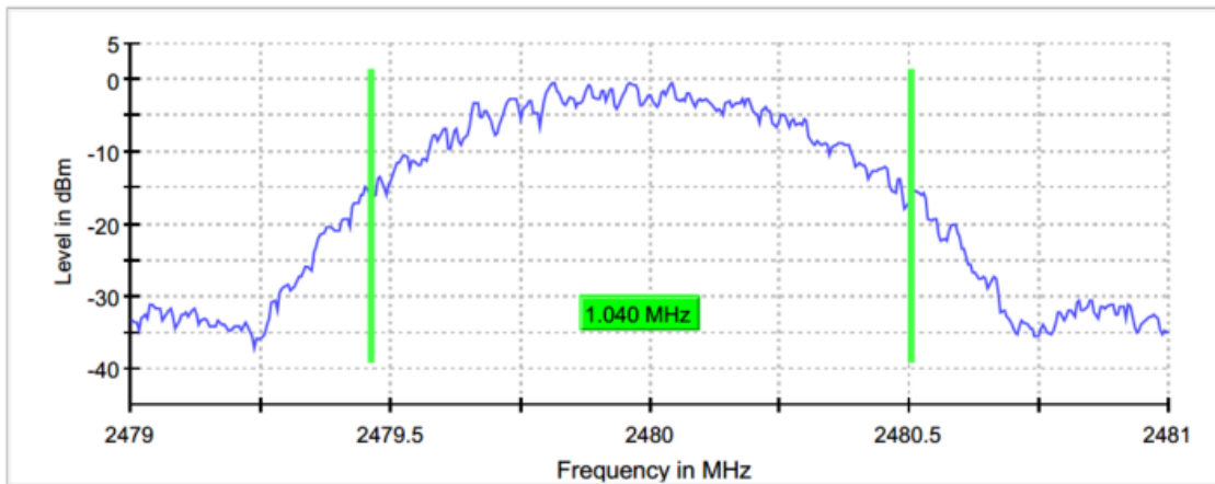
Figure 2.4.6-6: 99% BW - HCH
