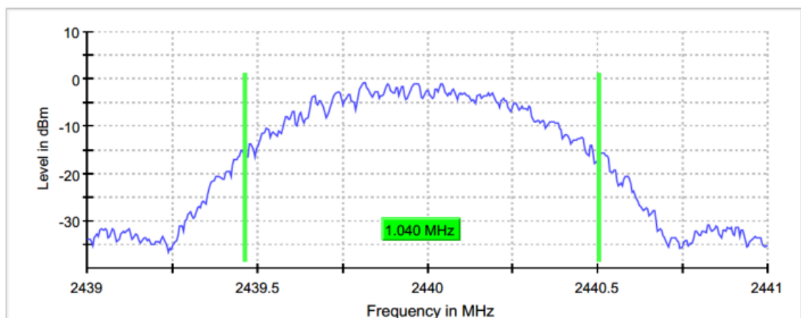
Figure 2.4.6-5: 99% BW - MCH
