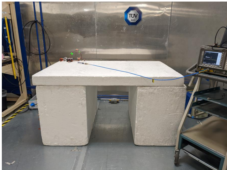
Figure 6: Test Setup – Conducted Emissions
