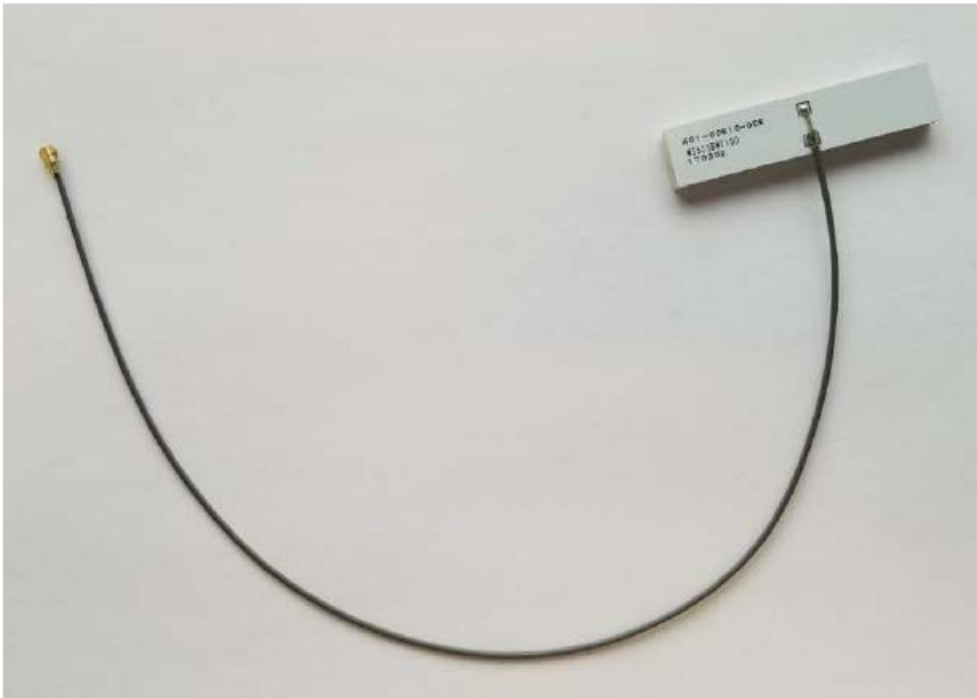
Figure 2: Flag Antenna
