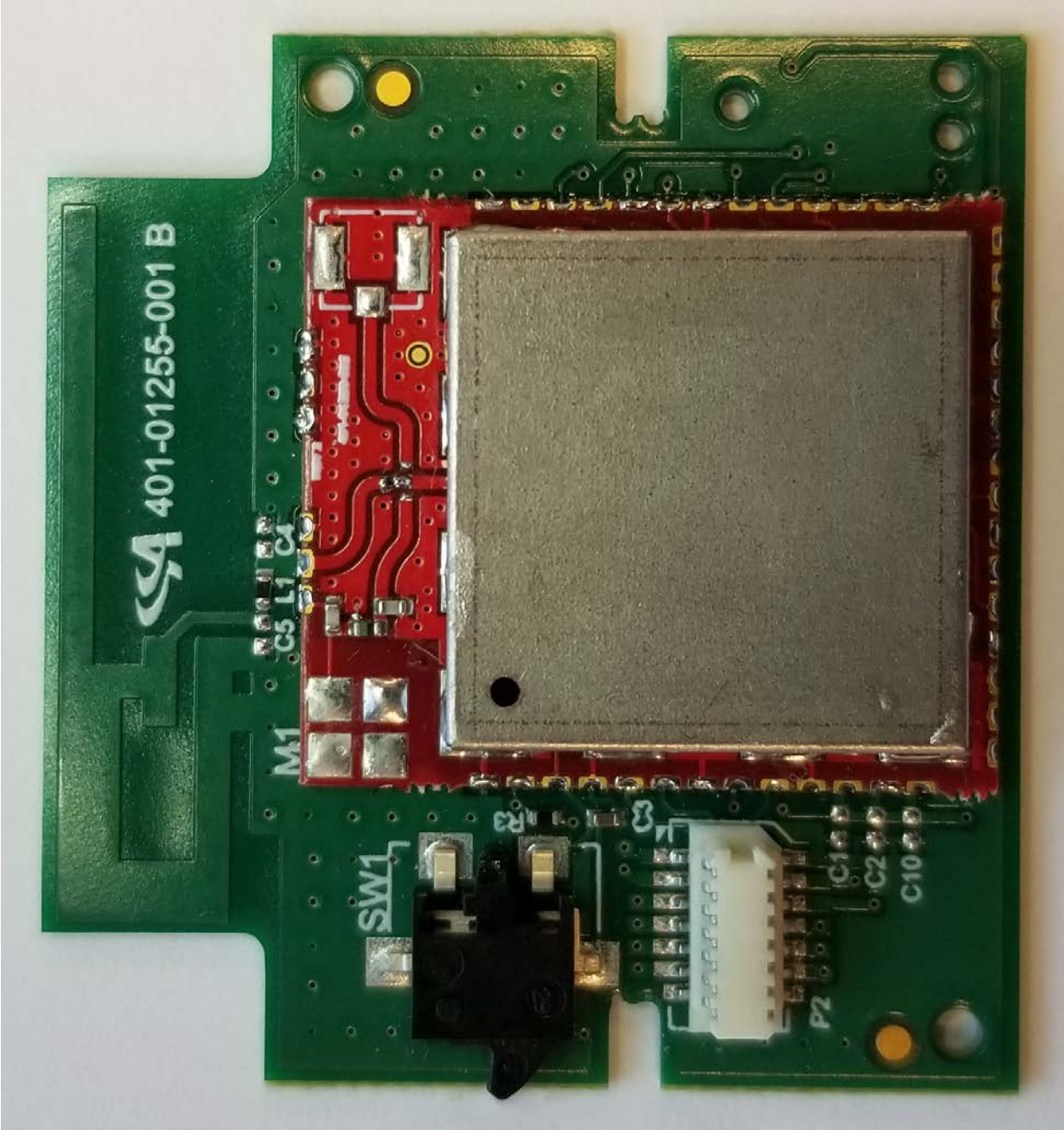
Figure 1: BMODIT Module with PIFA Antenna
