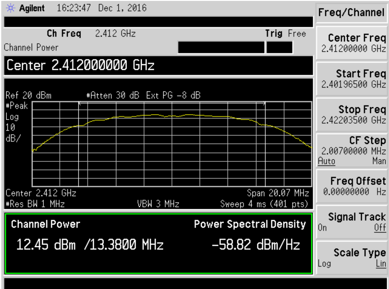
Figure 9. 802.11b, 1 Mbps Ch 1
