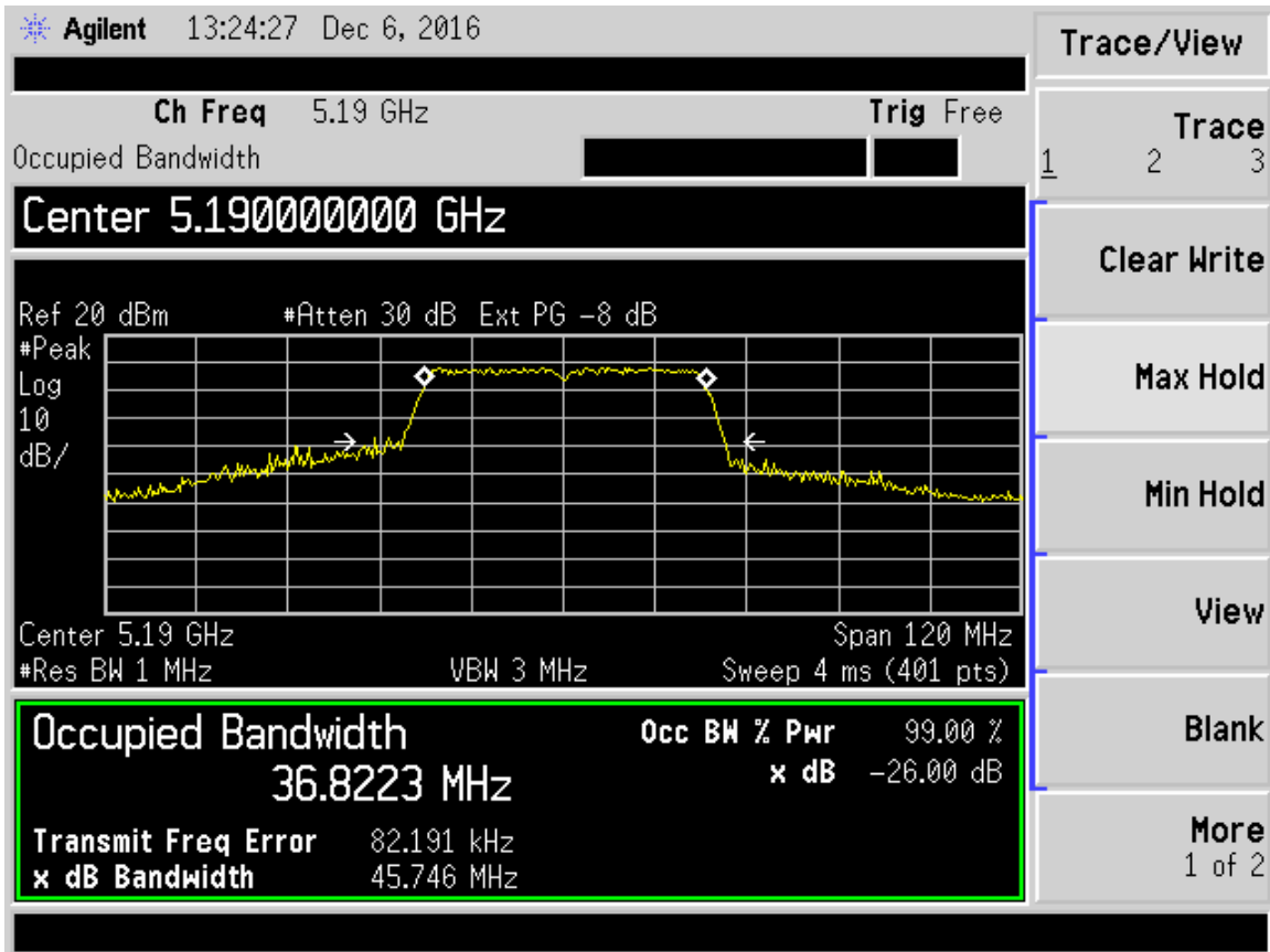
Figure 28. 802.11n(40) Ch 38, MCS0
