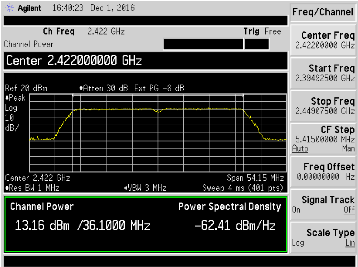
Figure 15. 802.11n(40), MCS0 Ch 1
