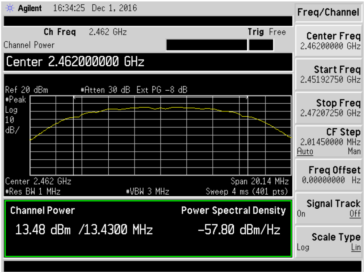
Figure 10. 802.11b, 1 Mbps Ch 11
