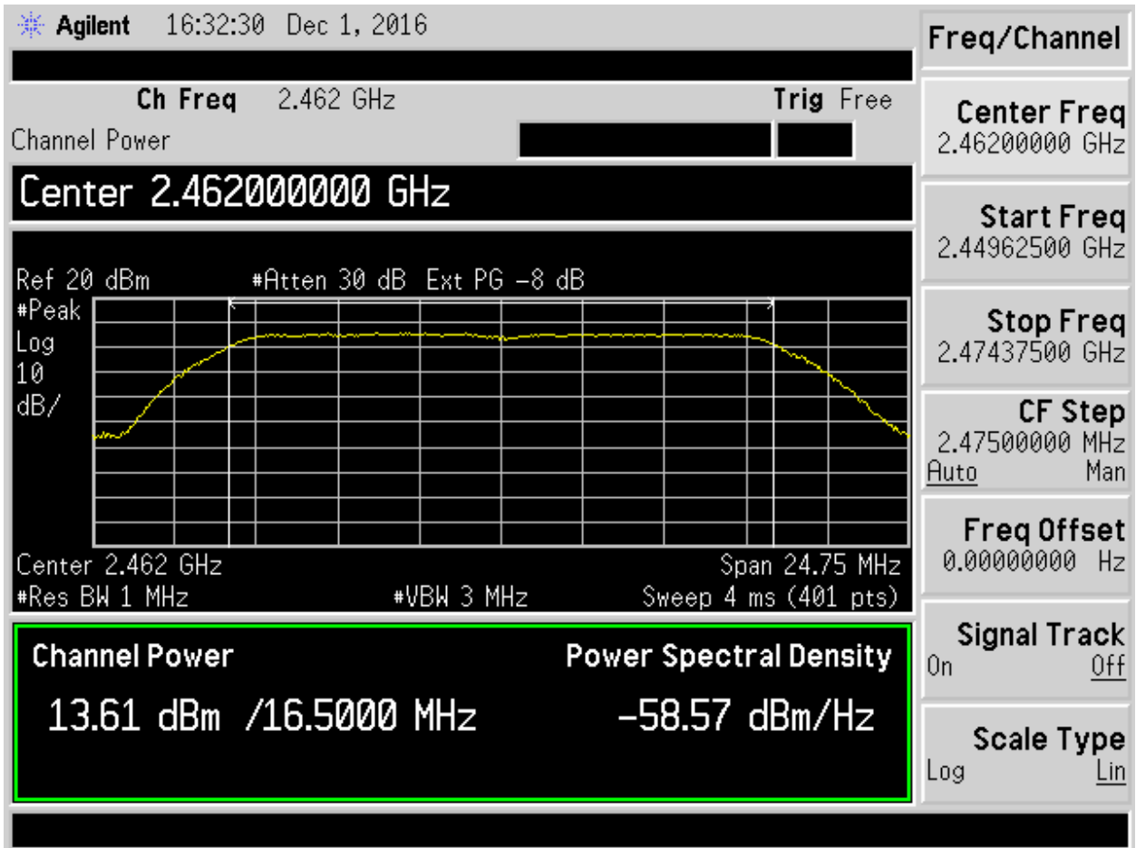
Figure 12. 802.11g, 6 Mbps Ch 11
