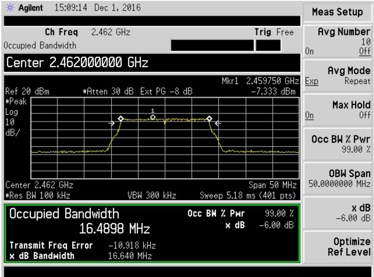
Figure 4. 802.11g, 6 Mbps Ch 11
