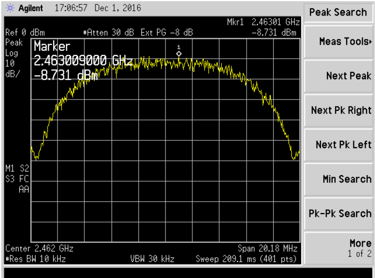
Figure 18. 802.11b, 1 Mbps Ch 11
