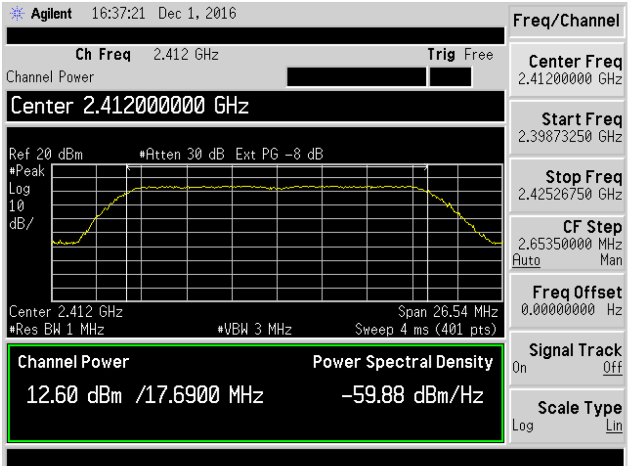
Figure 13. 802.11n, MCS0 Ch 1
