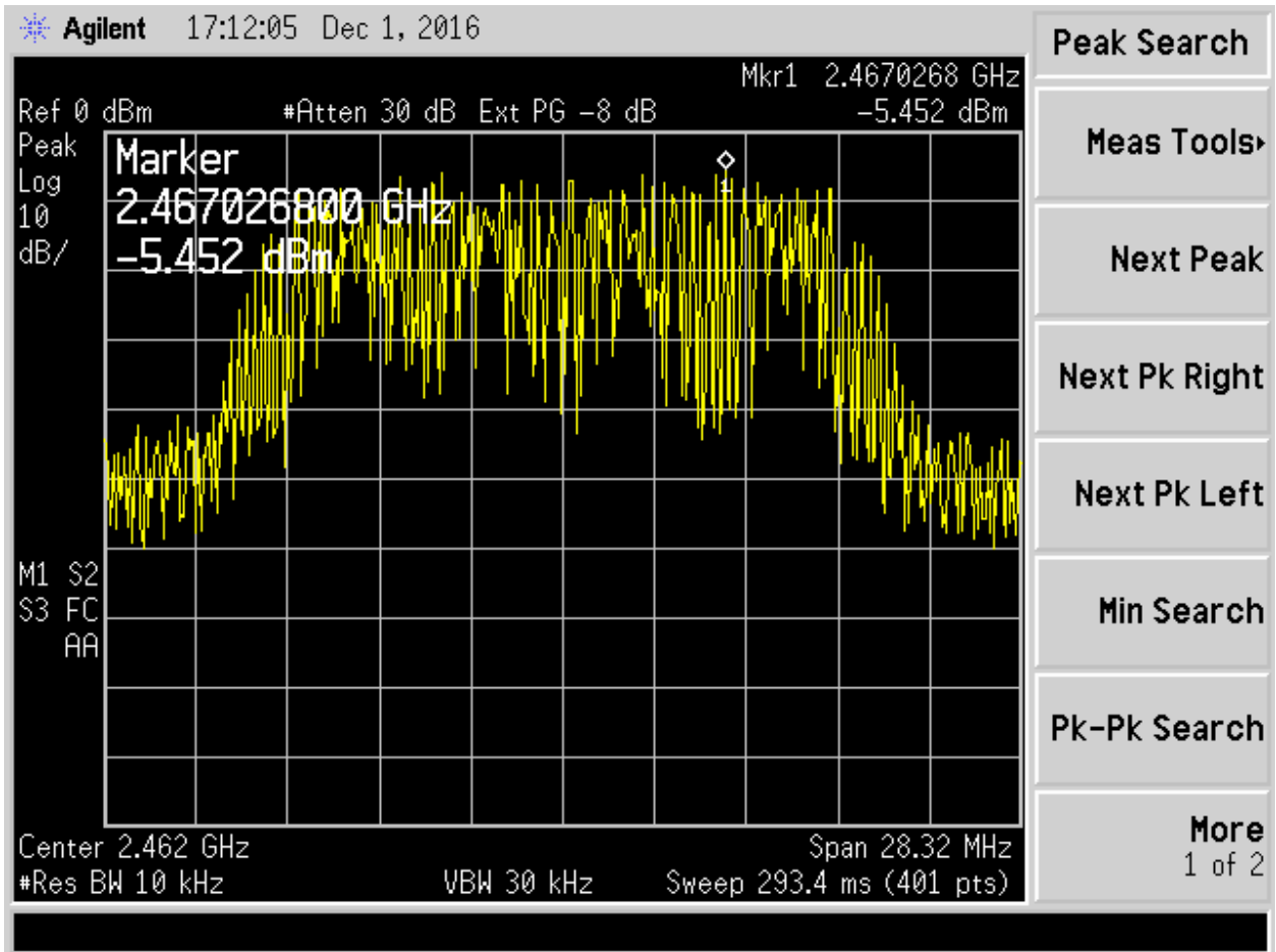
Figure 20. 802.11g, 6 Mbps Ch 11
