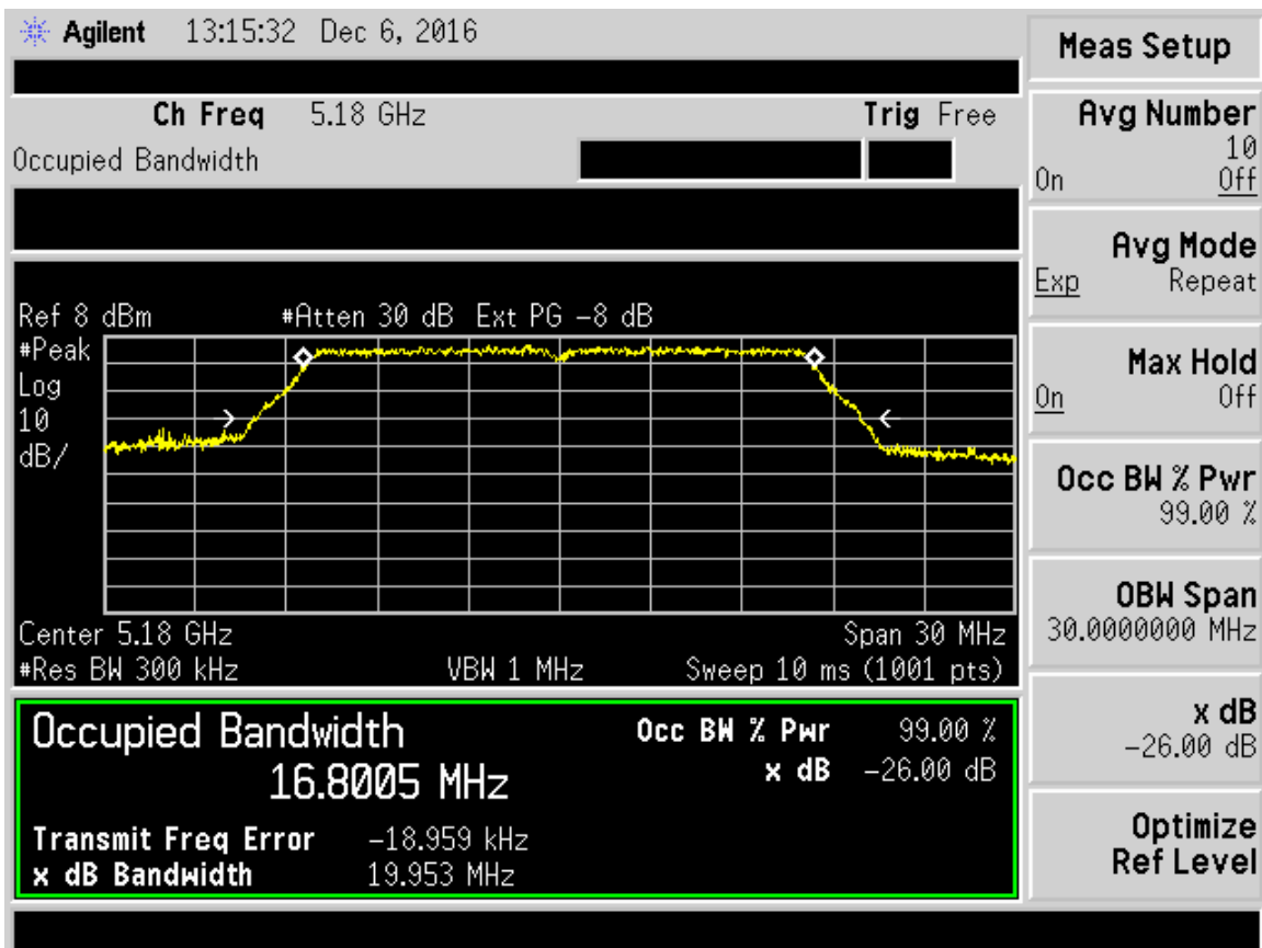
Figure 25. 802.11a(20), Ch 36, 6 Mbps
