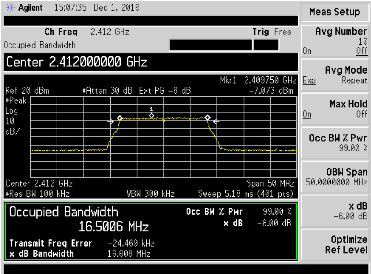
Figure 3. 802.11g, 6 Mbps Ch 1
