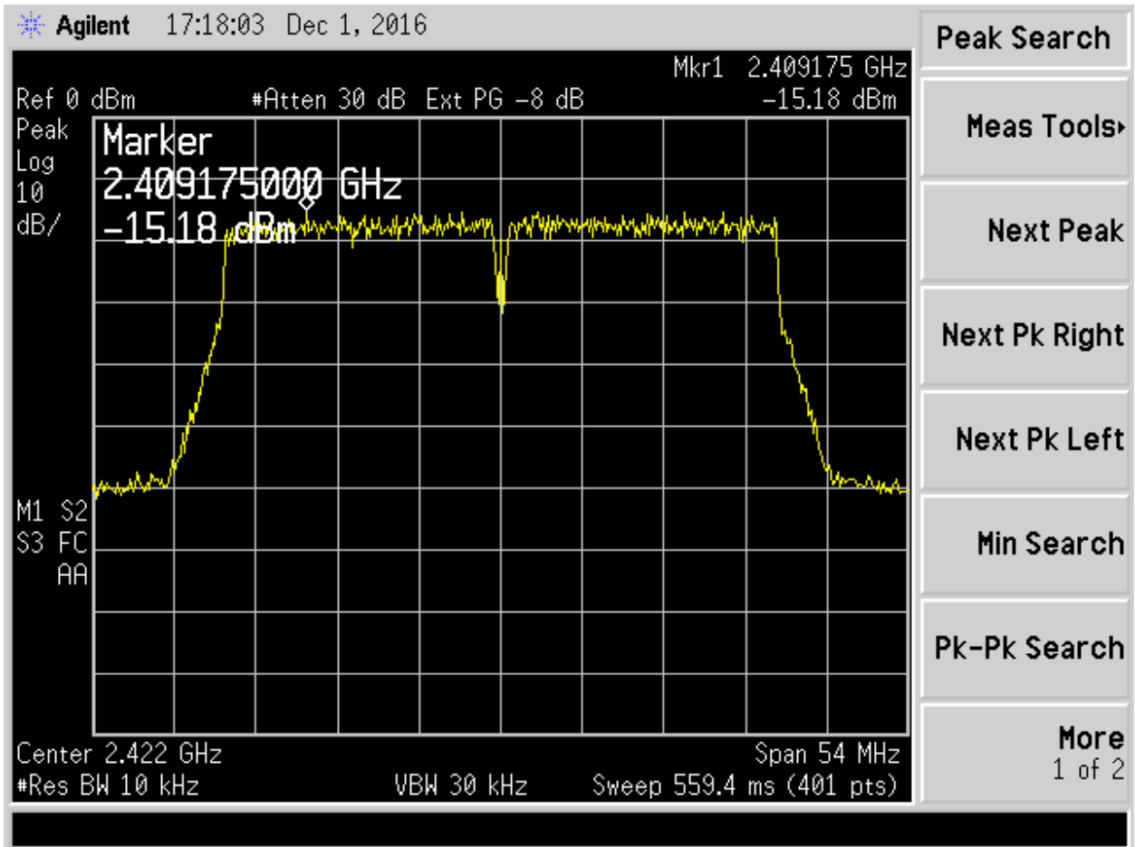
Figure 23. 802.11n(40), MCS0 Ch 3
