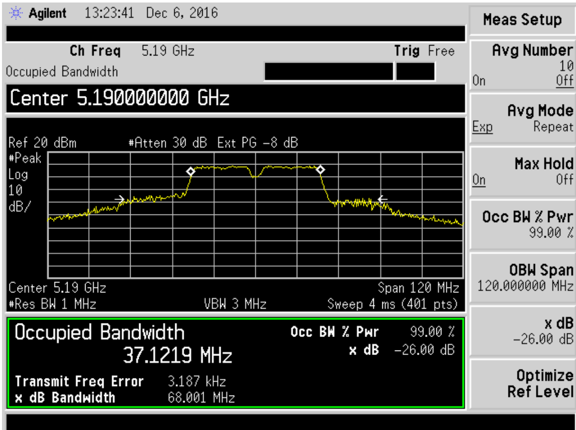
Figure 27. 802.11a(40), Ch 38, 6 Mbps
