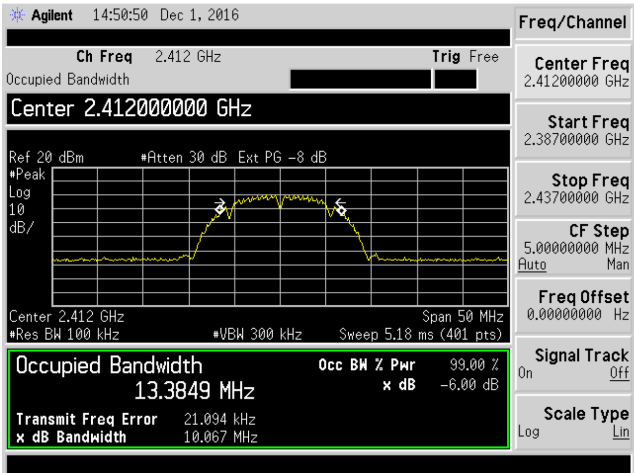
Figure 1. 802.11b, 1 Mbps Ch 1
