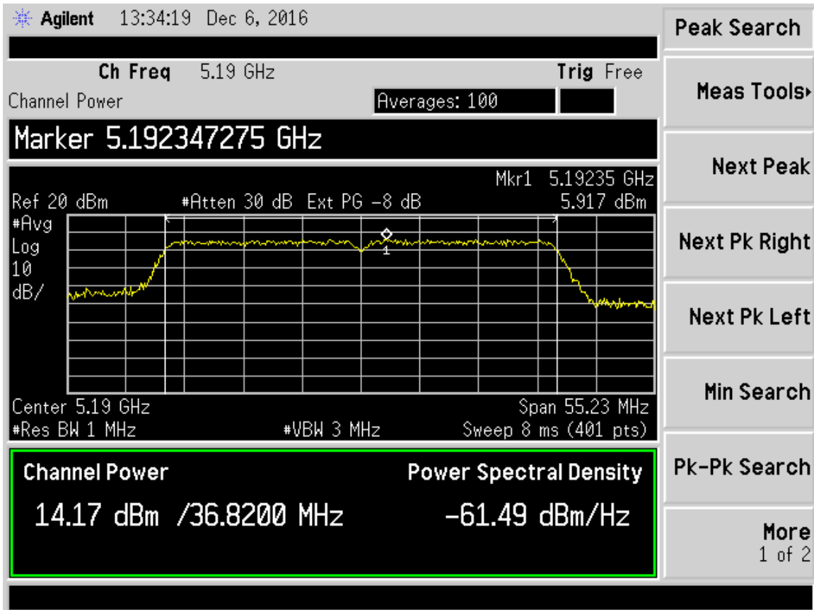
Figure 32. 802.11n(40) Ch 38, MCS0 Output Power and PSD
