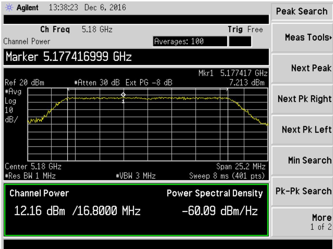
Figure 30. 802.11n Ch 36, MCS0 Output Power and PSD
