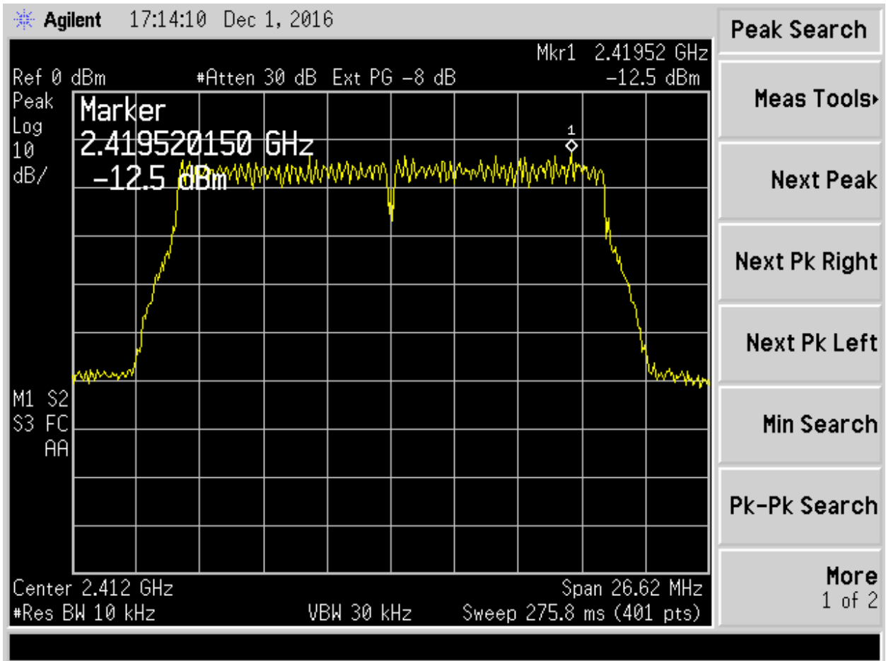
Figure 21. 802.11n, MCS0 Ch 1
