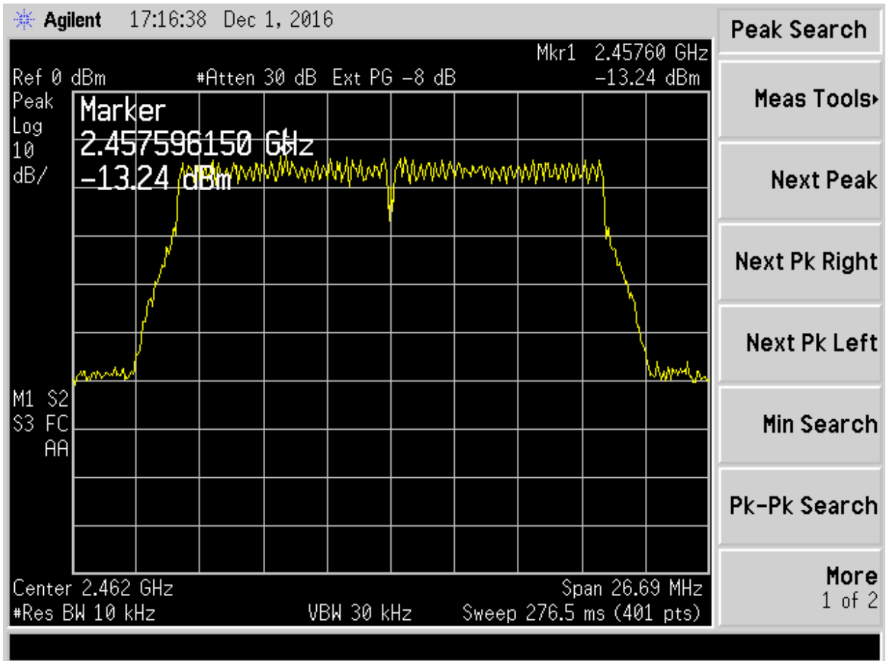
Figure 22. 802.11n, MCS0 Ch 11
