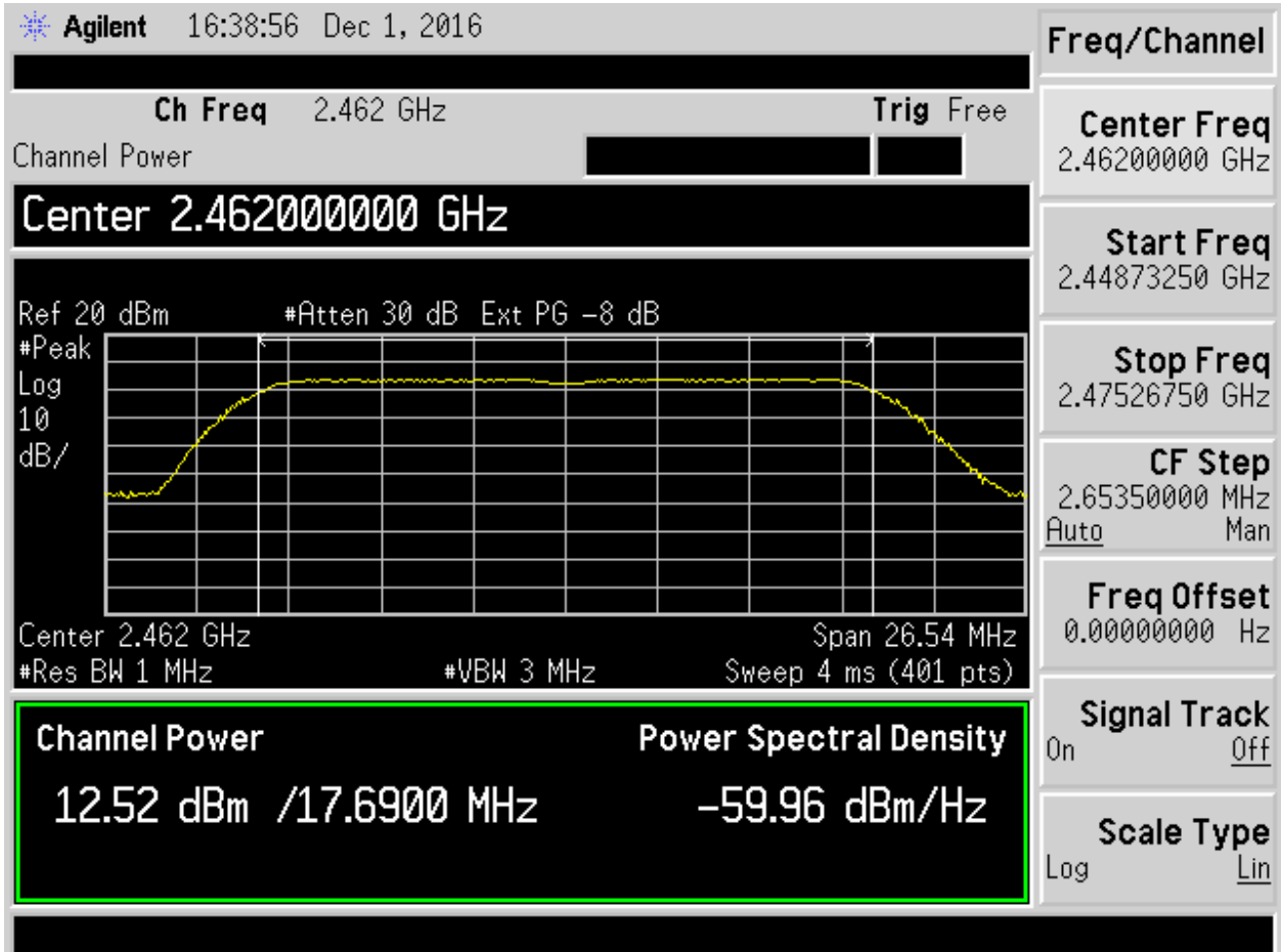
Figure 14. 802.11n, MCS7 Ch 11
