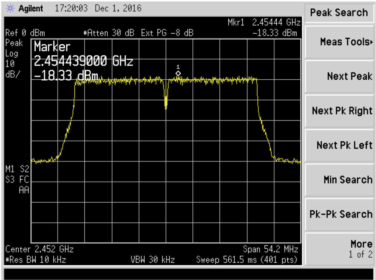
Figure 24. 802.11n(40), MCS0 Ch 11
