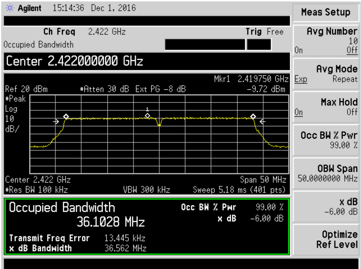
Figure 7. 802.11n(40), MCS0 Ch 3
