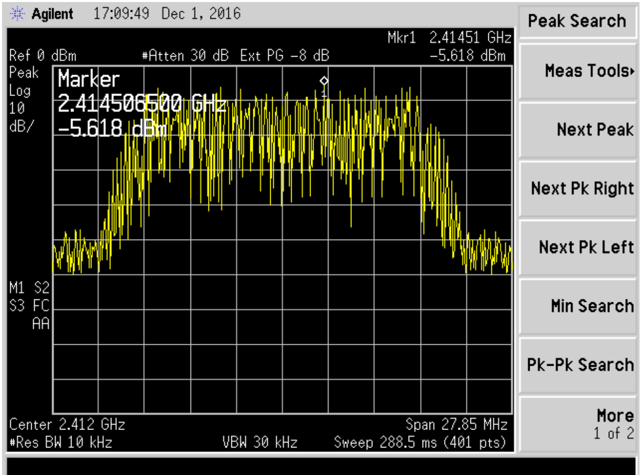
Figure 19. 802.11g, 6 Mbps Ch 1
