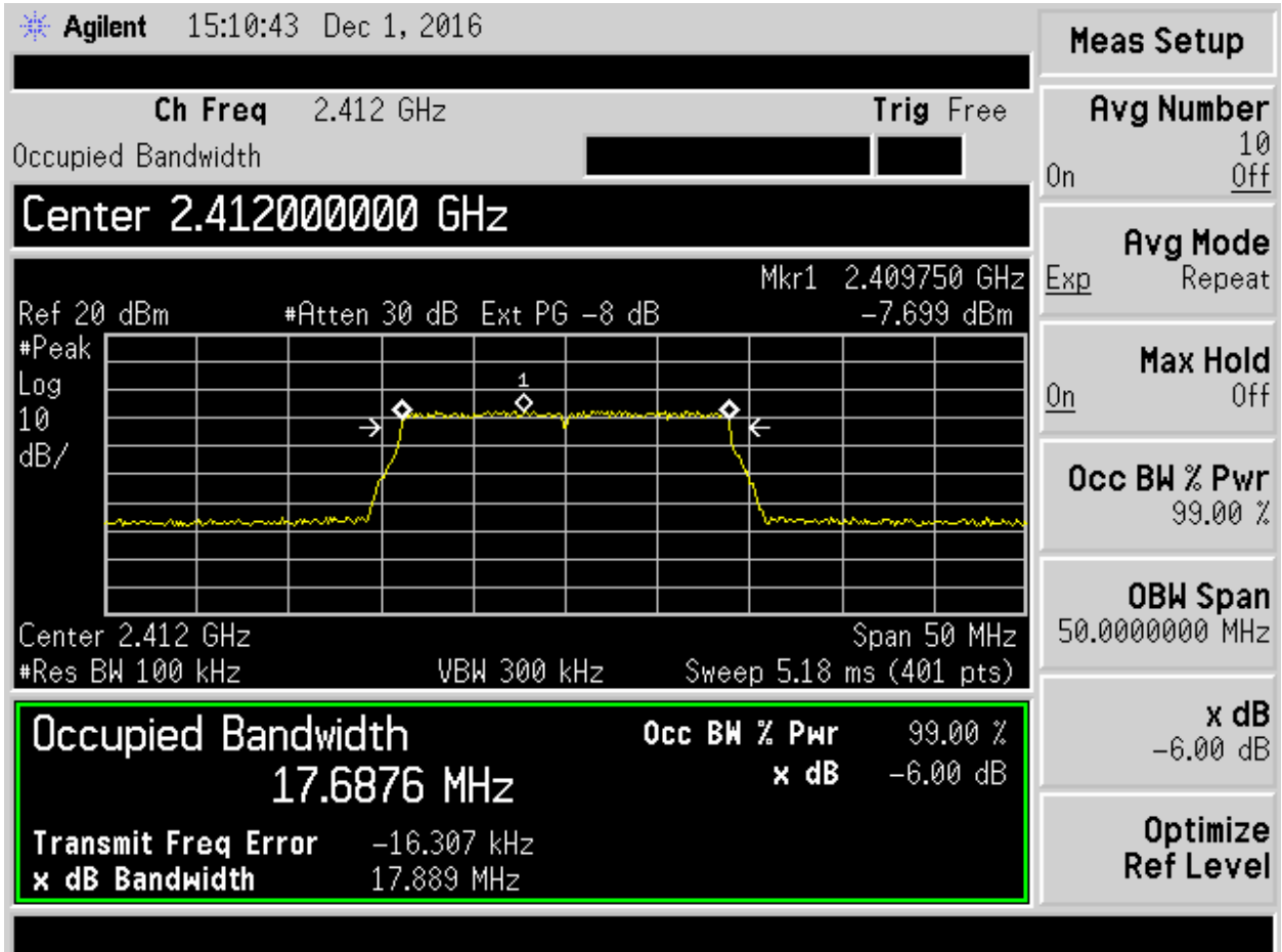
Figure 5. 802.11n, MCS0 Ch 1
