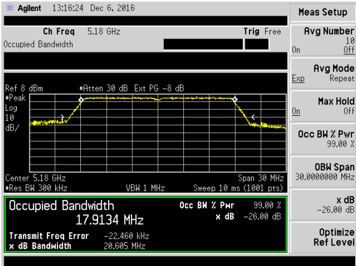
Figure 26. 802.11 Ch 36, MCS0
