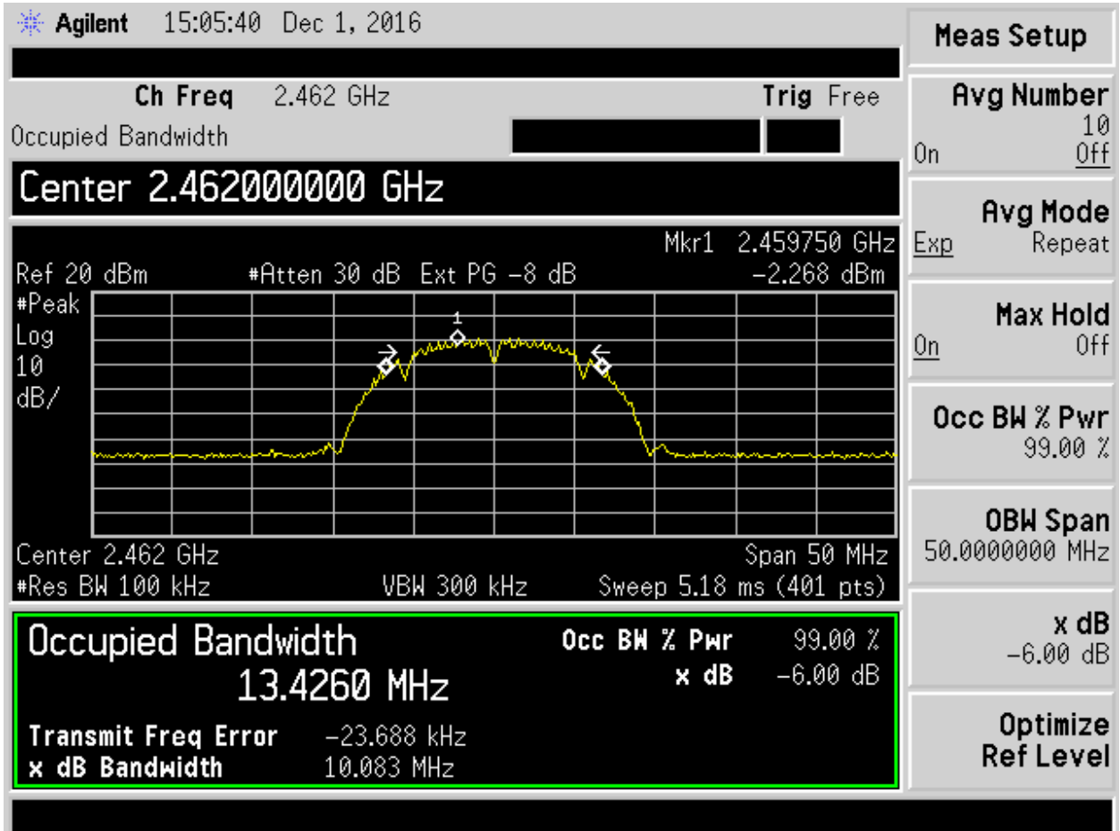
Figure 2. 802.11b, 1 Mbps Ch 11
