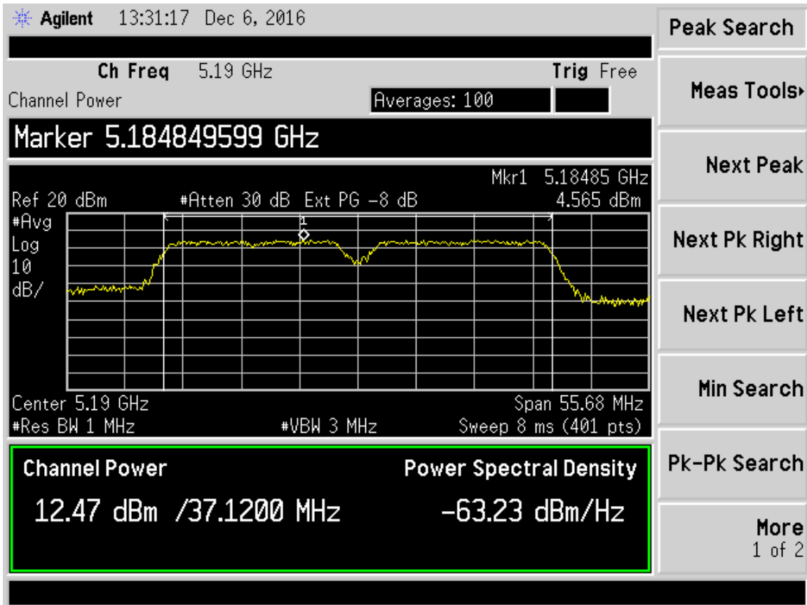
Figure 31. 802.11a(40), Ch 38 MCS0 Output Power and PSD
