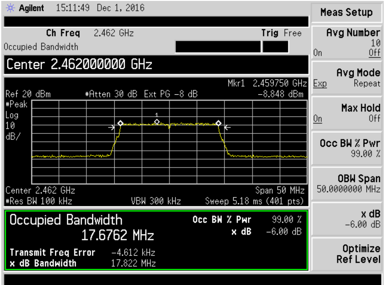
Figure 6. 802.11n, MCS0 Ch 11
