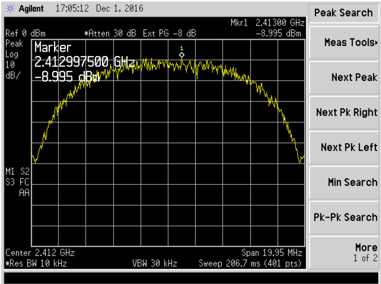
Figure 17. 802.11b, 1 Mbps Ch 1
