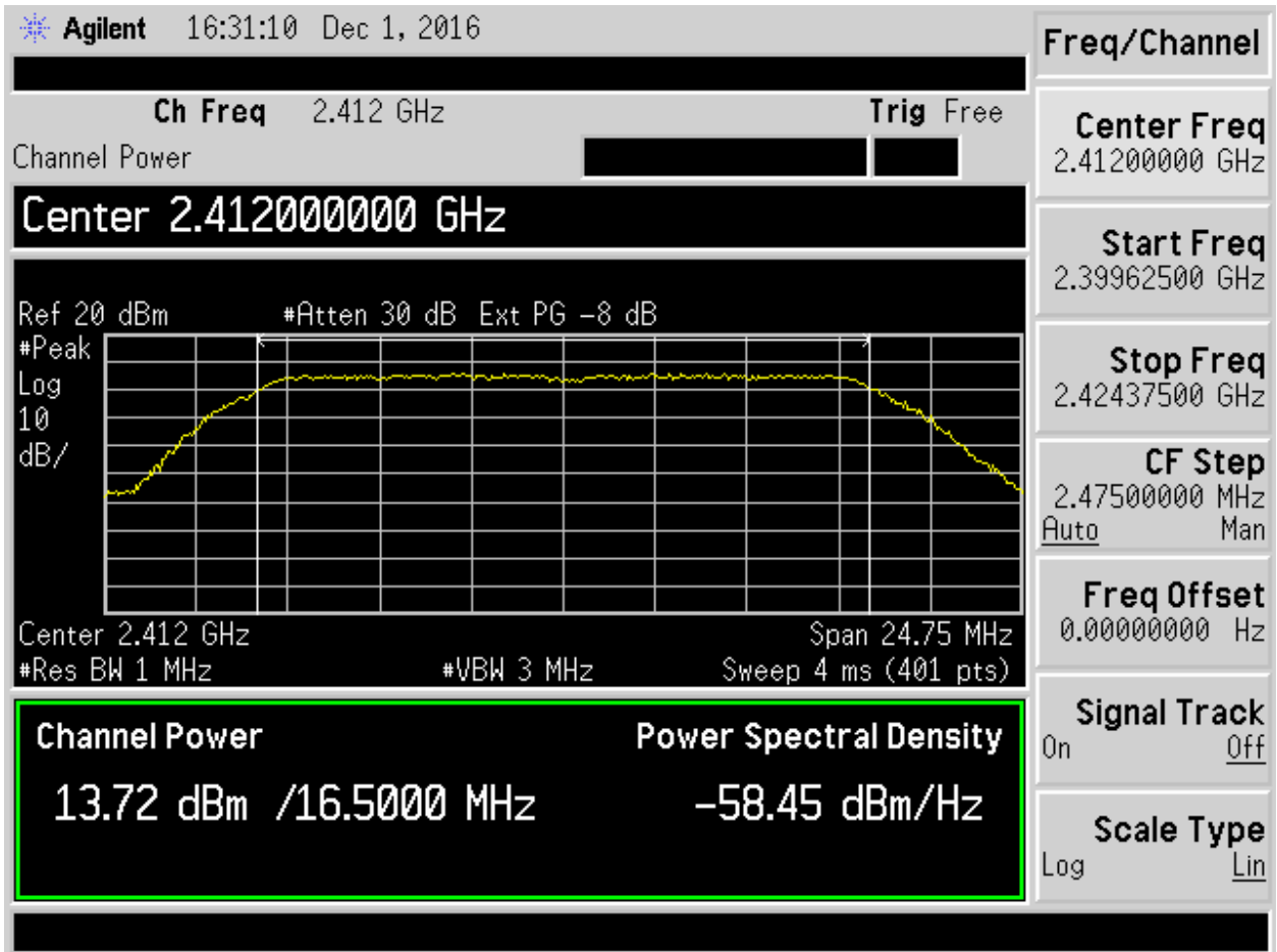
Figure 11. 802.11g, 6 Mbps Ch 1
