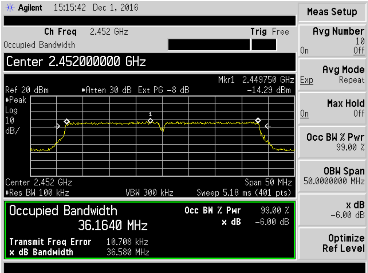
Figure 8. 802.11n(40), MCS0 Ch 9
