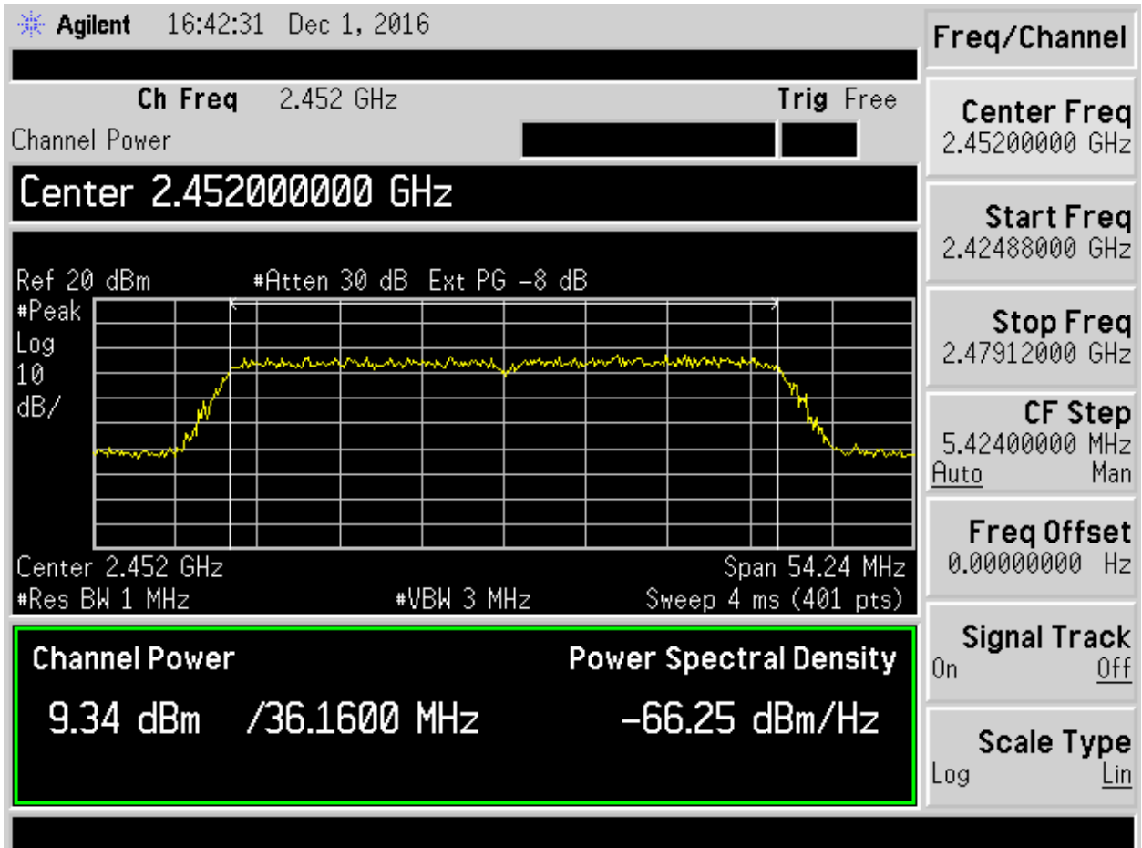
Figure 16. 802.11n(40), MCS7 Ch 11
