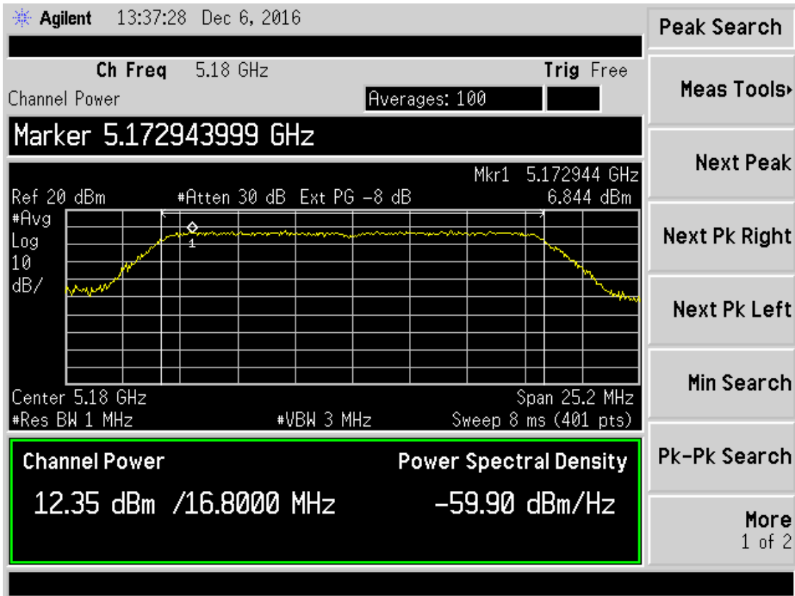
Figure 29. 802.11a Ch 36, 6 Mbps Output Power and PSD
