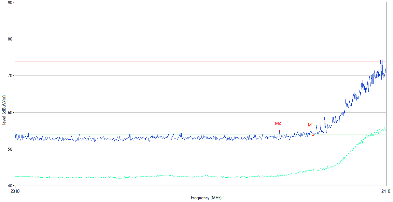
Bandedge_2.4G_Left
