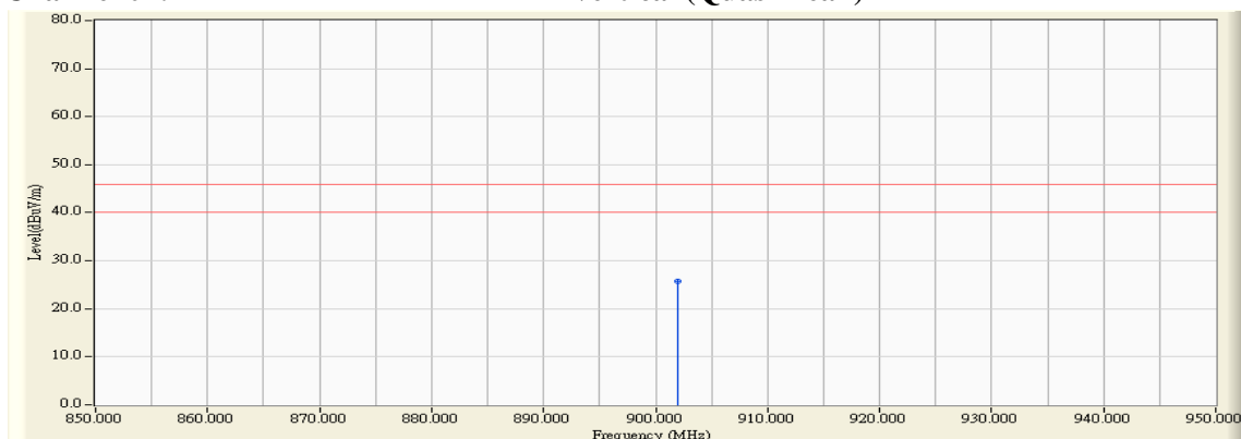
Figure Channel 01: Vertical (Quasi-Peak)
