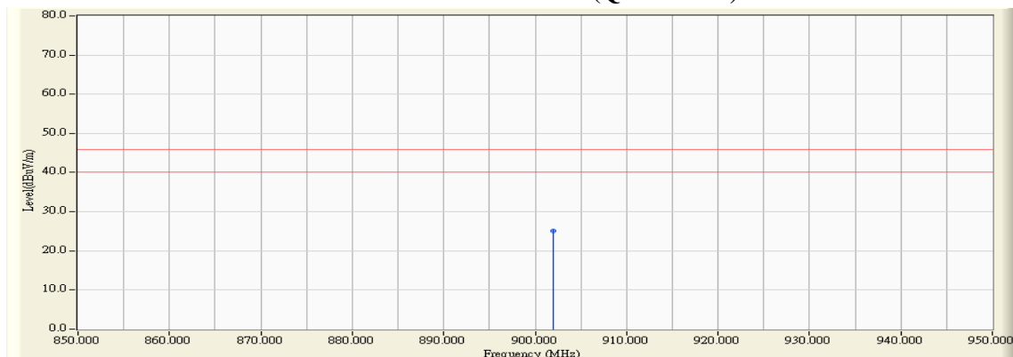
Figure Channel 01: Horizontal (Quasi-Peak)
