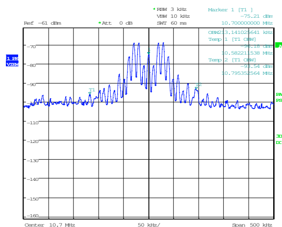
Plot carrier 10.7 MHz
