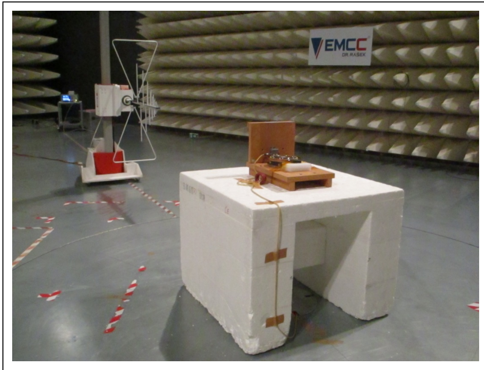
Photograph A1-3: Radiated emissions 30 - 150 MHz at 3 m distance
