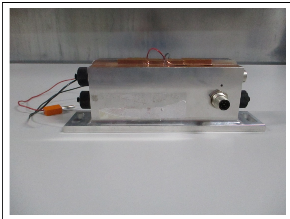
Photograph A3-2: Data cable termination box, view 2
