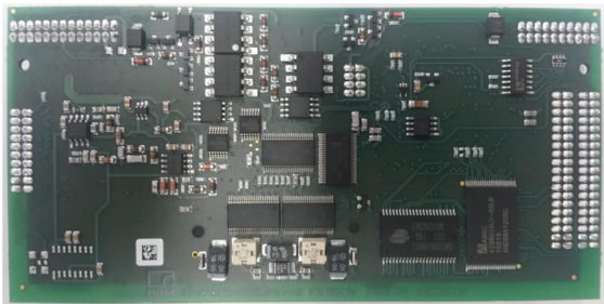
Rear
