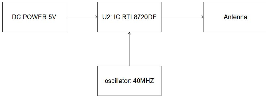
Figure1. Circuit Diagram
