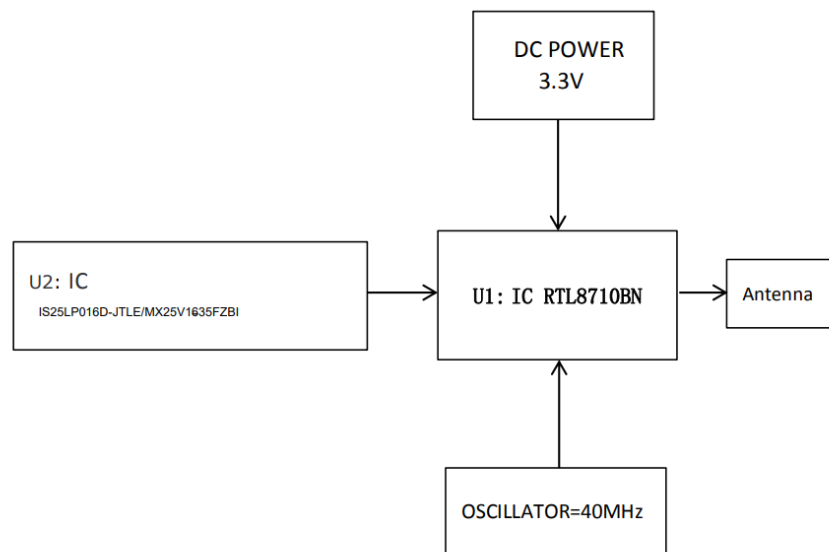
Figure1. Circuit Diagram
