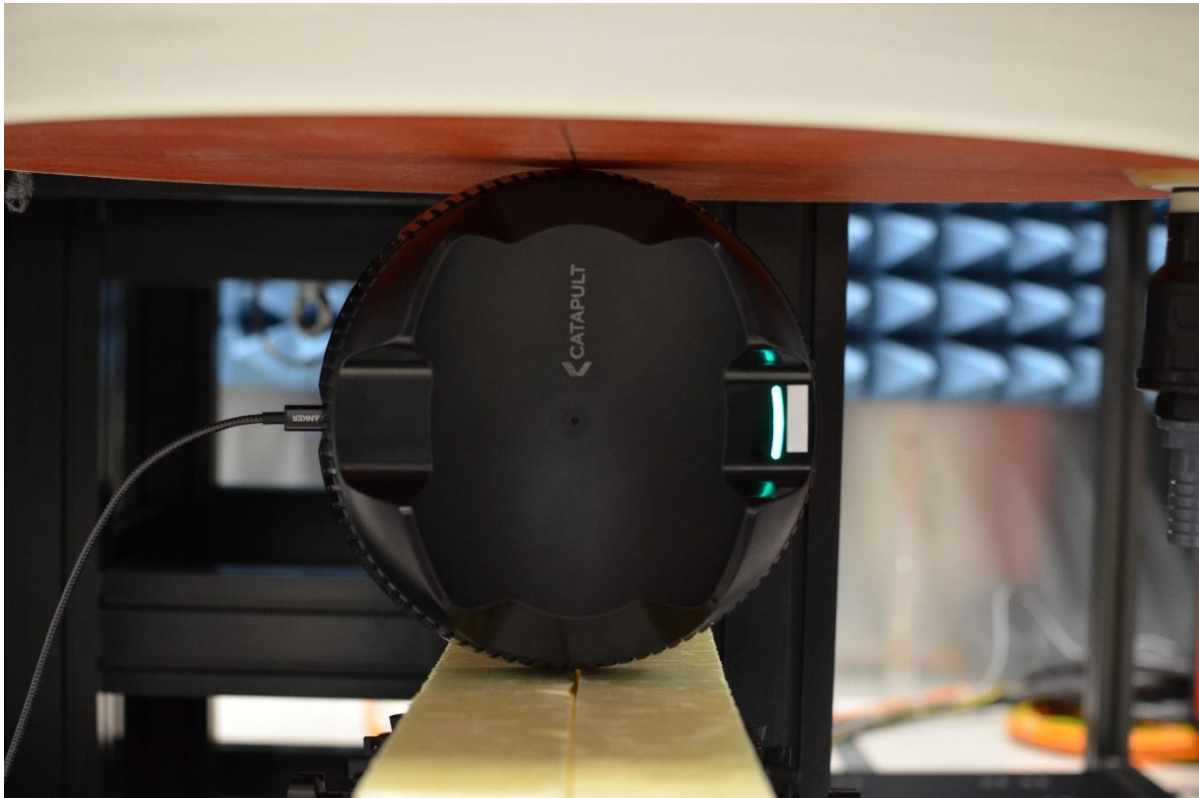
SAR Test Setup Photo 5: Body, Left Edge, 0 mm
