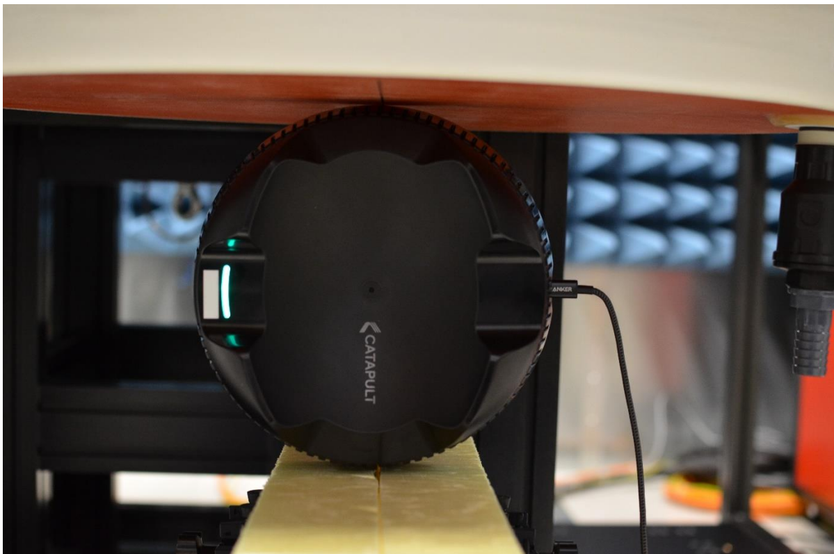
SAR Test Setup Photo 6: Body, Right Edge, 0 mm
