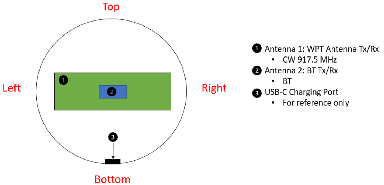
Figure E-1 DUT Antenna Locations
