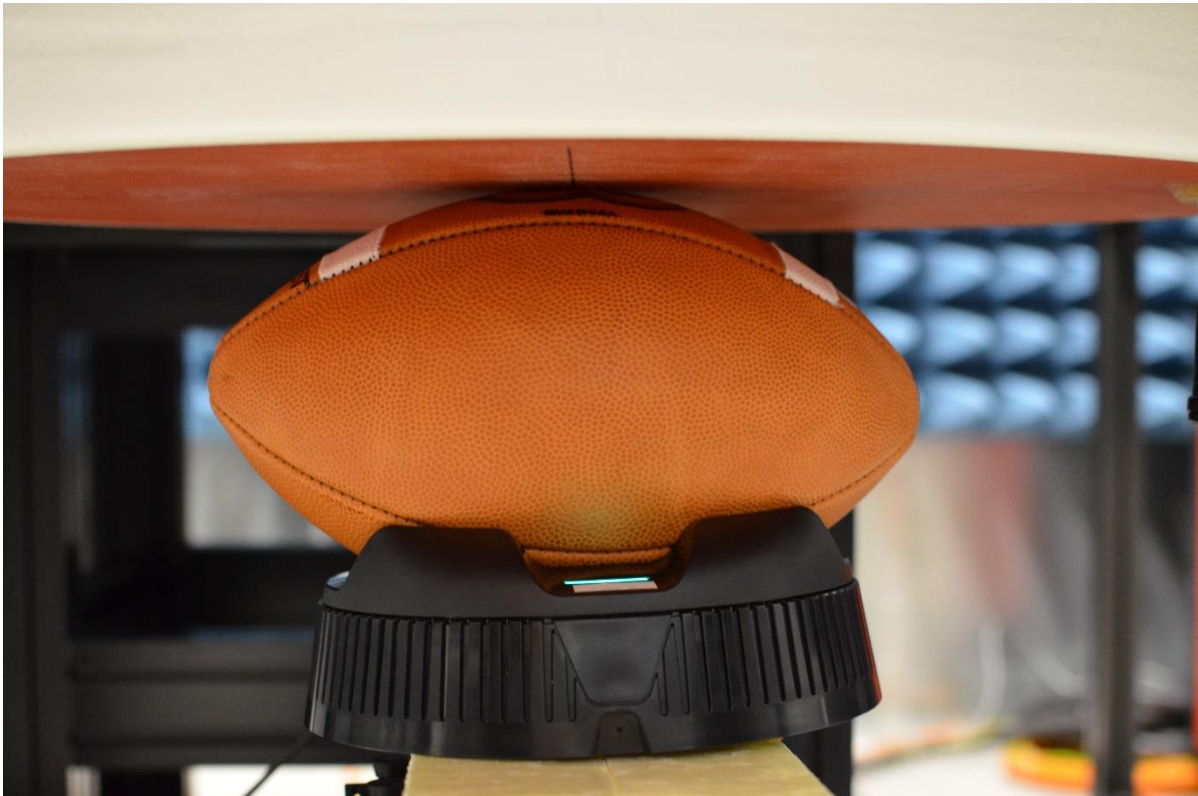
SAR Test Setup Photo 2: Body, Client Device on Cradle – “W” Logo Up, 130 mm
