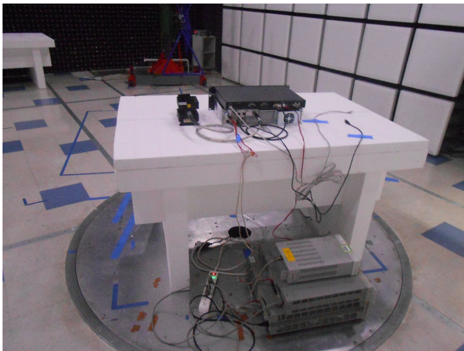
RF Radiated_ below 1 GHz #2
